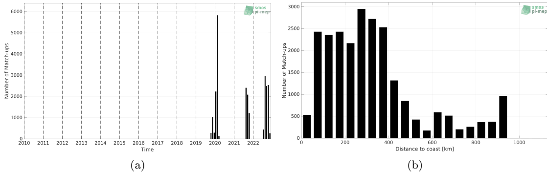
Figure 1: Number of match-ups between Saildrone and SMOS SSS L2Q v331 - With FLAG (CMEMS-CATDS-CPDC) SSS as a function of time (a) and as function of the distance to coast (b) over the Tropical Atlantic Ocean Pi-MEP region and for the full satellite product period.
