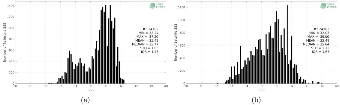
Figure 2: Histograms of SSS from Saildrone (a) and SMOS SSS L2Q v331 - With FLAG (CMEMS-CATDS-CPDC) (b) considering all match-up pairs per bins of 0.1 over the Tropical Atlantic Ocean Pi-MEP region and for the full satellite product period.
