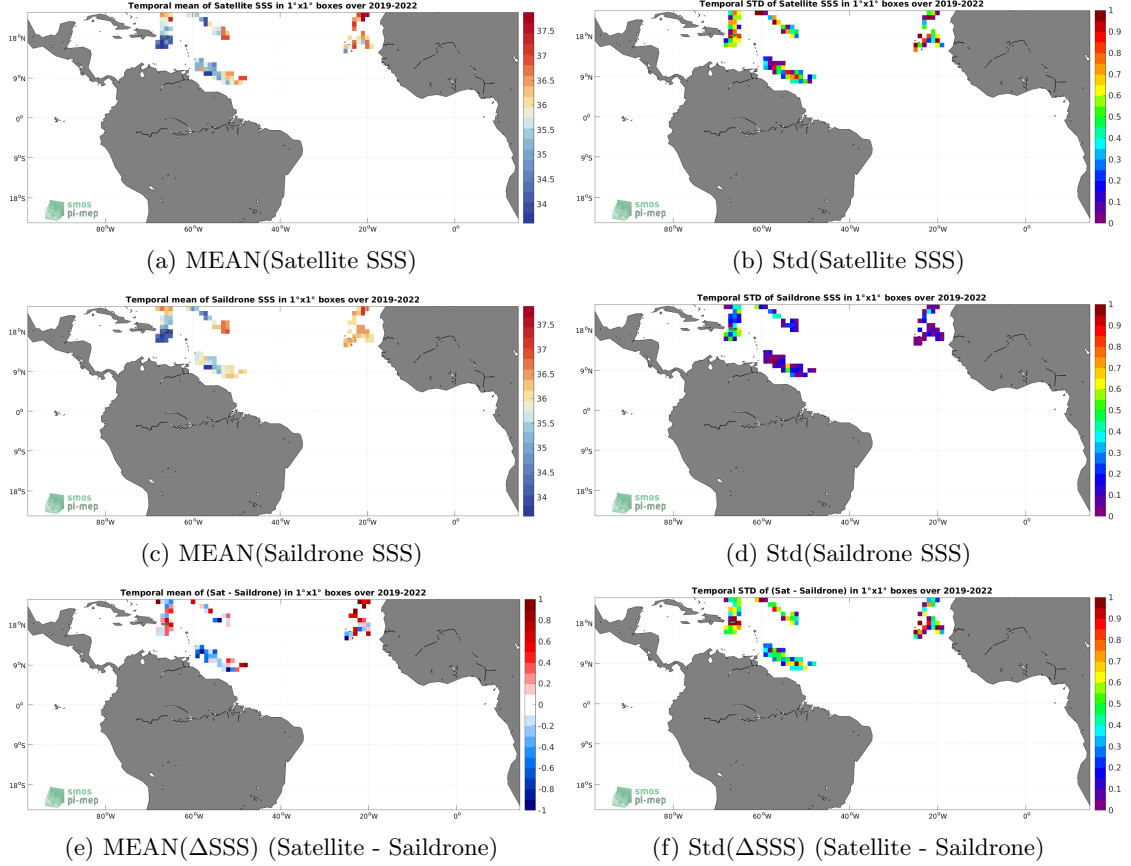
Figure 6: Temporal mean (left) and Std (right) of SSS from SMOS SSS L2Q v331 - With FLAG (CMEMS-CATDS-CPDC) (top), Sairdrone (middle), and of \Delta SSS (Satellite - Sairdrone). Only match-up pairs are used to generate these maps.
