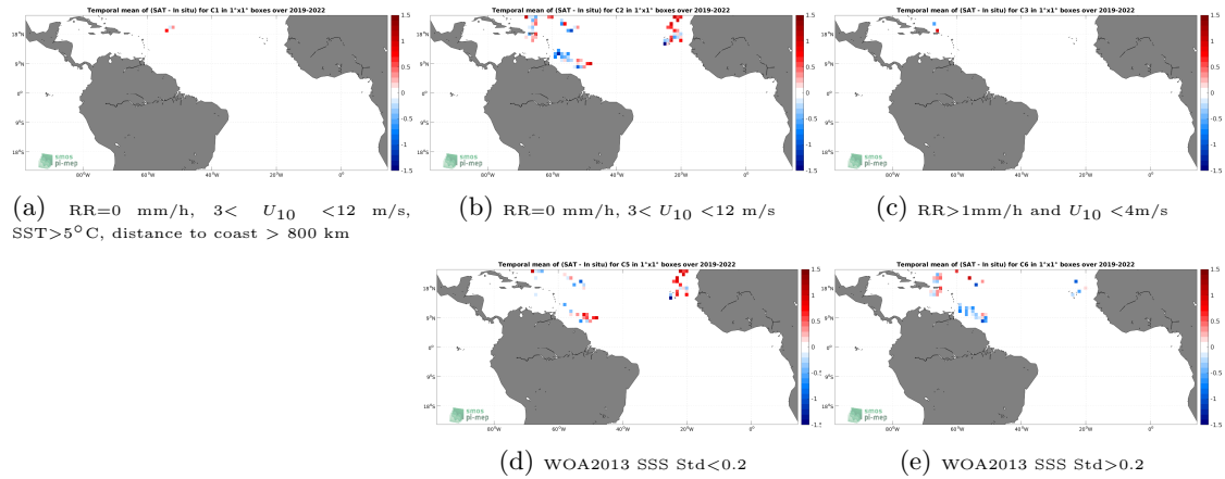
Figure 12: Temporal mean gridded over spatial boxes of size 1^\circ \times 1^\circ of \Delta\text{SSS} (SMOS SSS L2Q v331 - With FLAG (CMEMS-CATDS-CPDC) - Saildrone) for 5 different subdatasets corresponding to:RR=0 mm/h, 3 < U_{10} < 12 m/s, SST >5^\circ\text{C} , distance to coast > 800 km (a), RR=0 mm/h, 3 < U_{10} < 12 m/s (b), RR >1 mm/h and U_{10} < 4 m/s (c), WOA2013 SSS Std <0.2 (d), WOA2013 SSS Std >0.2 (e).
