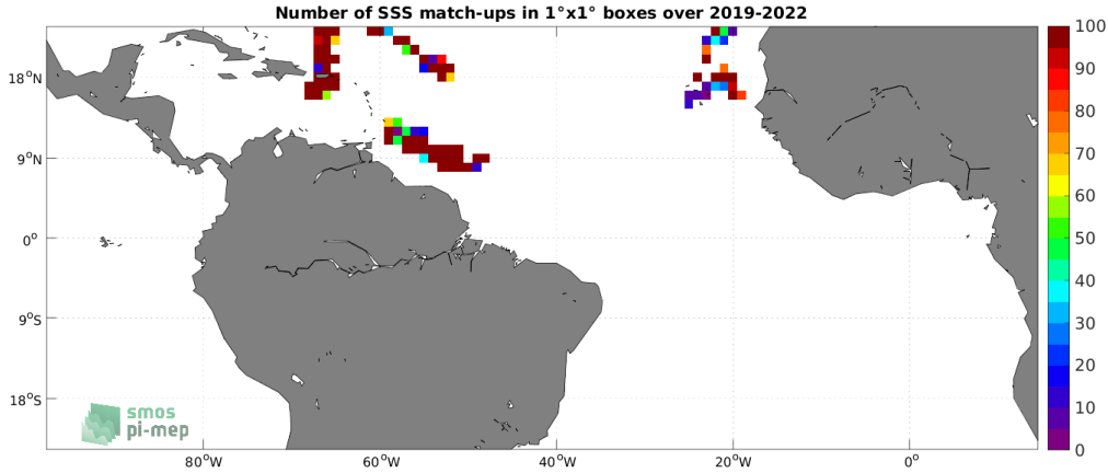
Figure 4: Number of SSS match-ups between Saildrone SSS and the SMOS SSS L2Q v331 - With FLAG (CMEMS-CATDS-CPDC) SSS product for the Tropical Atlantic Ocean Pi-MEP region over 1^\circ \times 1^\circ boxes and for the full satellite product period.
