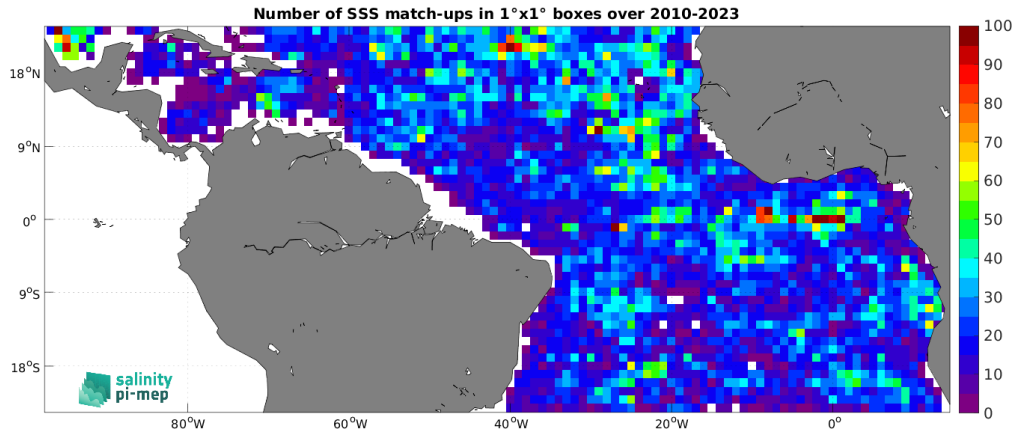
Figure 4: Number of SSS match-ups between Argo SSS and the SMOS SSS L2Q v331 - With FLAG (CMEMS-CATDS-CPDC) SSS product for the Tropical Atlantic Ocean Pi-MEP region over 1^\circ \times 1^\circ boxes and for the full satellite product period.
