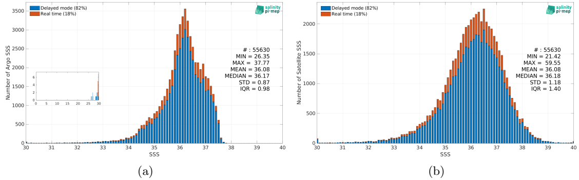
Figure 2: Histograms of SSS from Argo (a) and SMOS SSS L2Q v331 - With FLAG (CMEMS-CATDS-CPDC) (b) considering all match-up pairs per bins of 0.1 over the Tropical Atlantic Ocean Pi-MEP region and for the full satellite product period.
