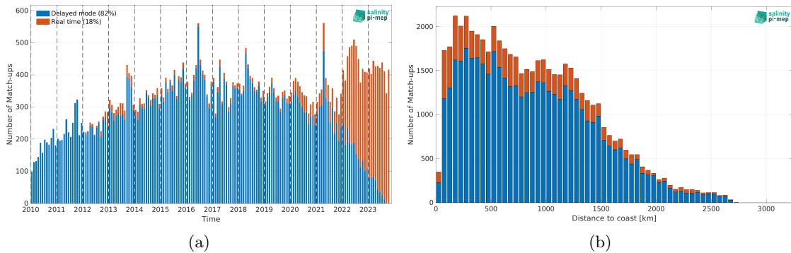
Figure 1: Number of match-ups between Argo and SMOS SSS L2Q v331 - With FLAG (CMEMS-CATDS-CPDC) SSS as a function of time (a) and as function of the distance to coast (b) over the Tropical Atlantic Ocean Pi-MEP region and for the full satellite product period.
