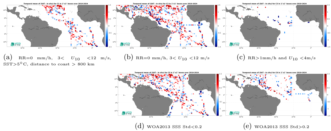
Figure 14: Temporal mean gridded over spatial boxes of size 1^\circ \times 1^\circ of \Delta\text{SSS} (SMOS SSS L2Q v331 - No FLAG (CMEMS-CATDS-CPDC) - TSG (SAMOS)) for 5 different subdatasets corresponding to:RR=0 mm/h, 3 < U_{10} < 12 m/s, SST >5^\circ\text{C} , distance to coast > 800 km (a), RR=0 mm/h, 3 < U_{10} < 12 m/s (b), RR >1 mm/h and U_{10} < 4 m/s (c), WOA2013 SSS Std <0.2 (d), WOA2013 SSS Std >0.2 (e).
