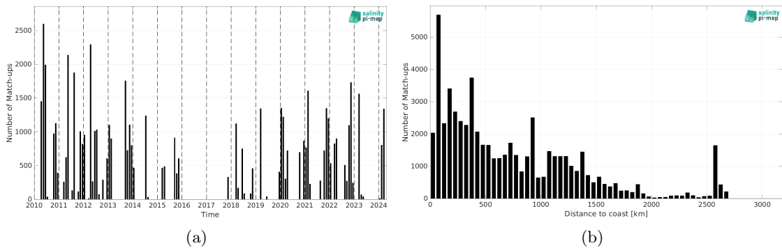
Figure 2: Number of match-ups between TSG (SAMOS) and SMOS SSS L2Q v331 - No FLAG (CMEMS-CATDS-CPDC) SSS as a function of time (a) and as function of the distance to coast (b) over the Tropical Atlantic Ocean Pi-MEP region and for the full satellite product period.
