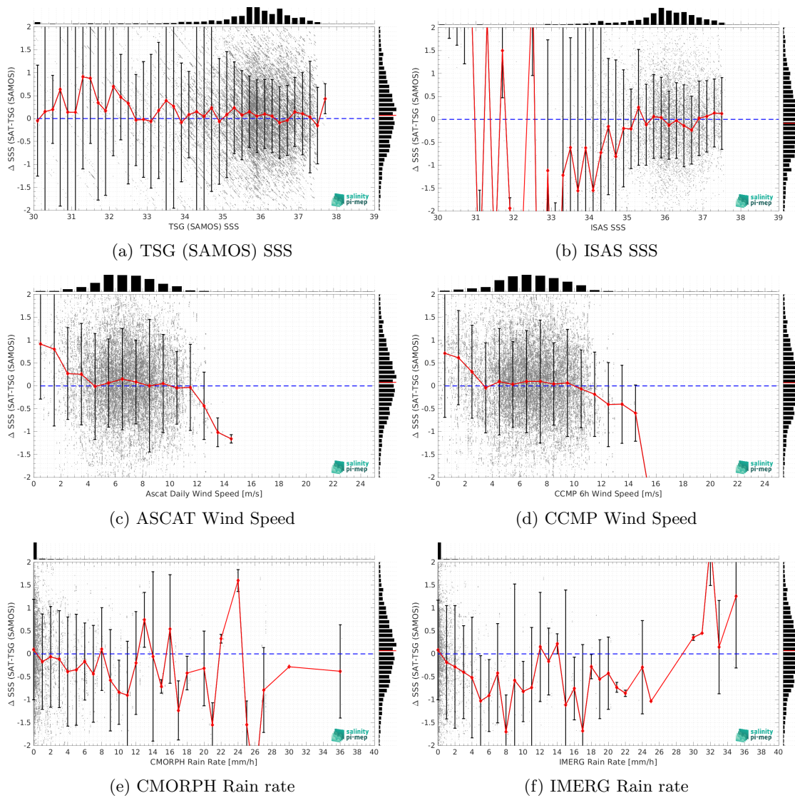
Figure 12: \Delta SSS (Satellite - TSG (SAMOS)) sorted as function of TSG (SAMOS) SSS (a), ISAS SSS (b), ASCAT Wind speed (c), CCMP Wind speed (d), CMORPH rain rate (e) and IMERG rain rate (f). In all plots the median and Std of \Delta SSS for each bin is indicated by the red curves and black vertical thick bars ( \pm 1 Std).
