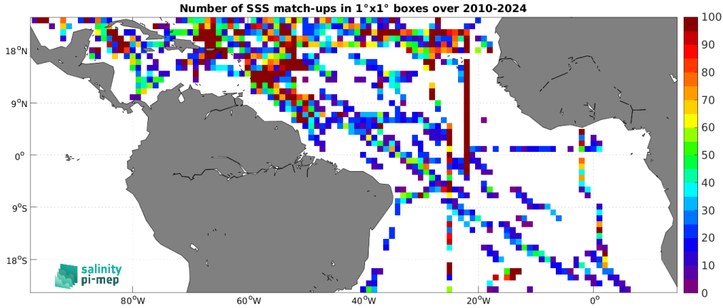
Figure 5: Number of SSS match-ups between TSG (SAMOS) SSS and the SMOS SSS L2Q v331 - No FLAG (CMEMS-CATDS-CPDC) SSS product for the Tropical Atlantic Ocean Pi-MEP region over 1^\circ \times 1^\circ boxes and for the full satellite product period.
