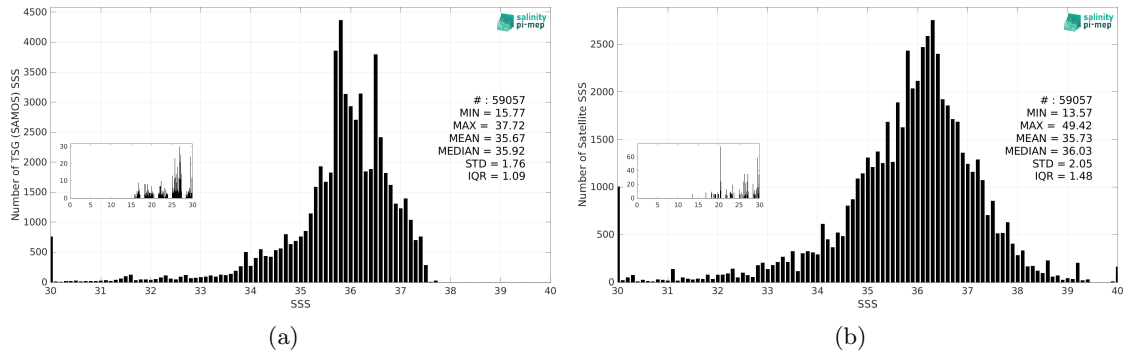
Figure 3: Histograms of SSS from TSG (SAMOS) (a) and SMOS SSS L2Q v331 - No FLAG (CMEMS-CATDS-CPDC) (b) considering all match-up pairs per bins of 0.1 over the Tropical Atlantic Ocean Pi-MEP region and for the full satellite product period.
