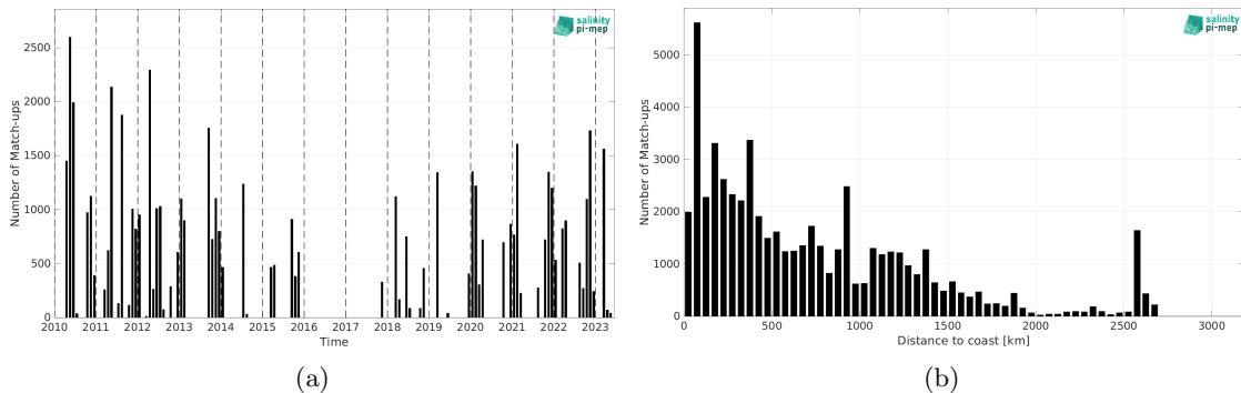
Figure 1: Number of match-ups between TSG (SAMOS) and SMOS SSS L2Q v331 - No FLAG (CMEMS-CATDS-CPDC) SSS as a function of time (a) and as function of the distance to coast (b) over the Tropical Atlantic Ocean Pi-MEP region and for the full satellite product period.
