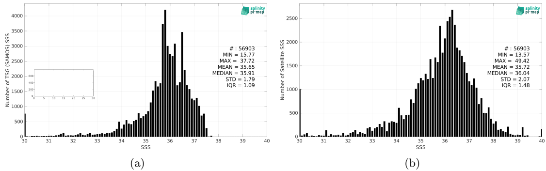
Figure 2: Histograms of SSS from TSG (SAMOS) (a) and SMOS SSS L2Q v331 - No FLAG (CMEMS-CATDS-CPDC) (b) considering all match-up pairs per bins of 0.1 over the Tropical Atlantic Ocean Pi-MEP region and for the full satellite product period.
