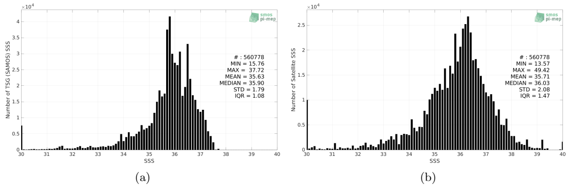
Figure 2: Histograms of SSS from TSG (SAMOS) (a) and SMOS SSS L2Q v331 - No FLAG (CMEMS-CATDS-CPDC) (b) considering all match-up pairs per bins of 0.1 over the Tropical Atlantic Ocean Pi-MEP region and for the full satellite product period.
