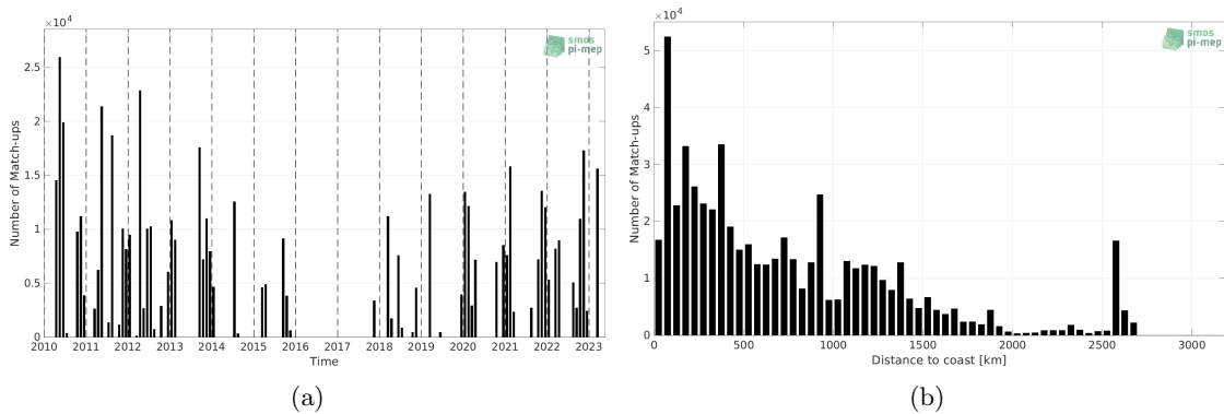
Figure 1: Number of match-ups between TSG (SAMOS) and SMOS SSS L2Q v331 - No FLAG (CMEMS-CATDS-CPDC) SSS as a function of time (a) and as function of the distance to coast (b) over the Tropical Atlantic Ocean Pi-MEP region and for the full satellite product period.
