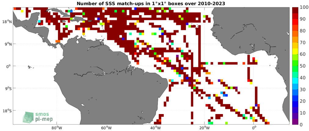
Figure 4: Number of SSS match-ups between TSG (SAMOS) SSS and the SMOS SSS L2Q v331 - No FLAG (CMEMS-CATDS-CPDC) SSS product for the Tropical Atlantic Ocean Pi-MEP region over 1^\circ \times 1^\circ boxes and for the full satellite product period.
