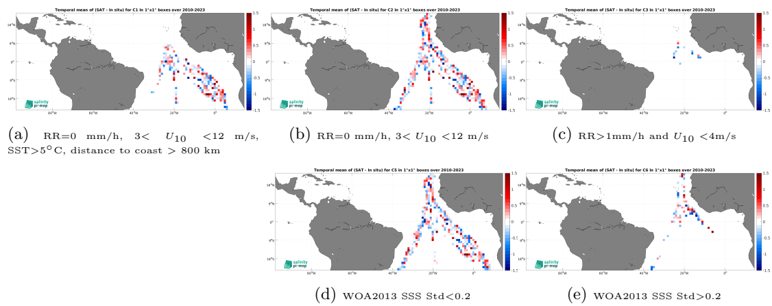
Figure 14: Temporal mean gridded over spatial boxes of size 1^\circ \times 1^\circ of \Delta\text{SSS} (SMOS SSS L2Q v331 - No FLAG (CMEMS-CATDS-CPDC) - TSG (Polarstern)) for 5 different subdatasets corresponding to:RR=0 mm/h, 3 < U_{10} < 12 m/s, SST >5^\circ\text{C} , distance to coast > 800 km (a), RR=0 mm/h, 3 < U_{10} < 12 m/s (b), RR >1 mm/h and U_{10} < 4 m/s (c), WOA2013 SSS Std <0.2 (d), WOA2013 SSS Std >0.2 (e).
