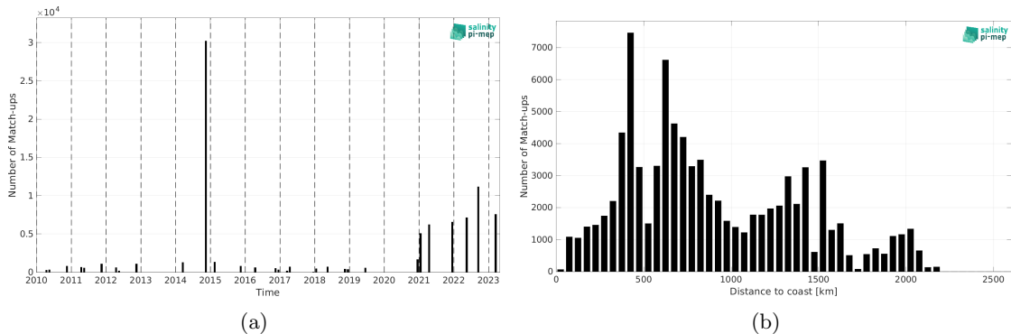
Figure 2: Number of match-ups between TSG (Polarstern) and SMOS SSS L2Q v331 - No FLAG (CMEMS-CATDS-CPDC) SSS as a function of time (a) and as function of the distance to coast (b) over the Tropical Atlantic Ocean Pi-MEP region and for the full satellite product period.
