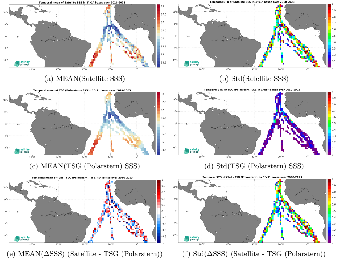
Figure 7: Temporal mean (left) and Std (right) of SSS from SMOS SSS L2Q v331 - No FLAG (CMEMS-CATDS-CPDC) (top), TSG (Polarstern) (middle), and of \Delta\text{SSS} (Satellite - TSG (Polarstern)). Only match-up pairs are used to generate these maps.
