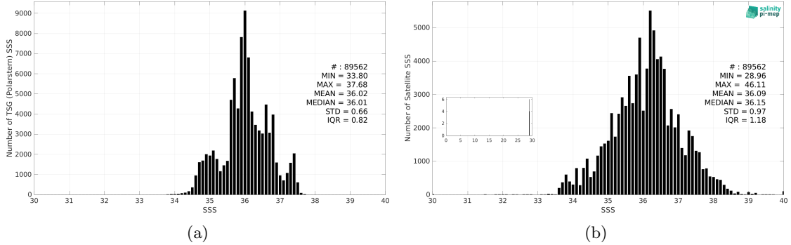
Figure 3: Histograms of SSS from TSG (Polarstern) (a) and SMOS SSS L2Q v331 - No FLAG (CMEMS-CATDS-CPDC) (b) considering all match-up pairs per bins of 0.1 over the Tropical Atlantic Ocean Pi-MEP region and for the full satellite product period.
