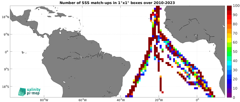
Figure 5: Number of SSS match-ups between TSG (Polarstern) SSS and the SMOS SSS L2Q v331 - No FLAG (CMEMS-CATDS-CPDC) SSS product for the Tropical Atlantic Ocean Pi-MEP region over 1^\circ \times 1^\circ boxes and for the full satellite product period.
