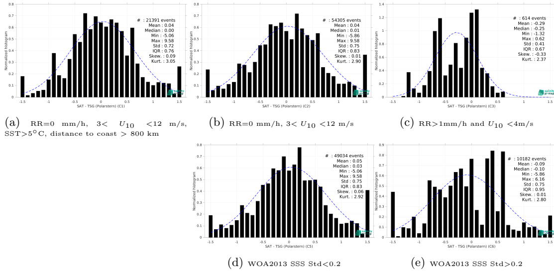
Figure 13: Normalized histogram of \Delta\text{SSS} (SMOS SSS L2Q v331 - No FLAG (CMEMS-CATDS-CPDC) - TSG (Polarstern)) for 5 different subdatasets corresponding to: RR=0 mm/h, 3 < U_{10} < 12 m/s, SST>5°C, distance to coast > 800 km (a), RR=0 mm/h, 3 < U_{10} < 12 m/s (b), RR>1mm/h and U_{10} < 4 m/s (c), WOA2013 SSS Std<0.2 (d), WOA2013 SSS Std>0.2 (e).
