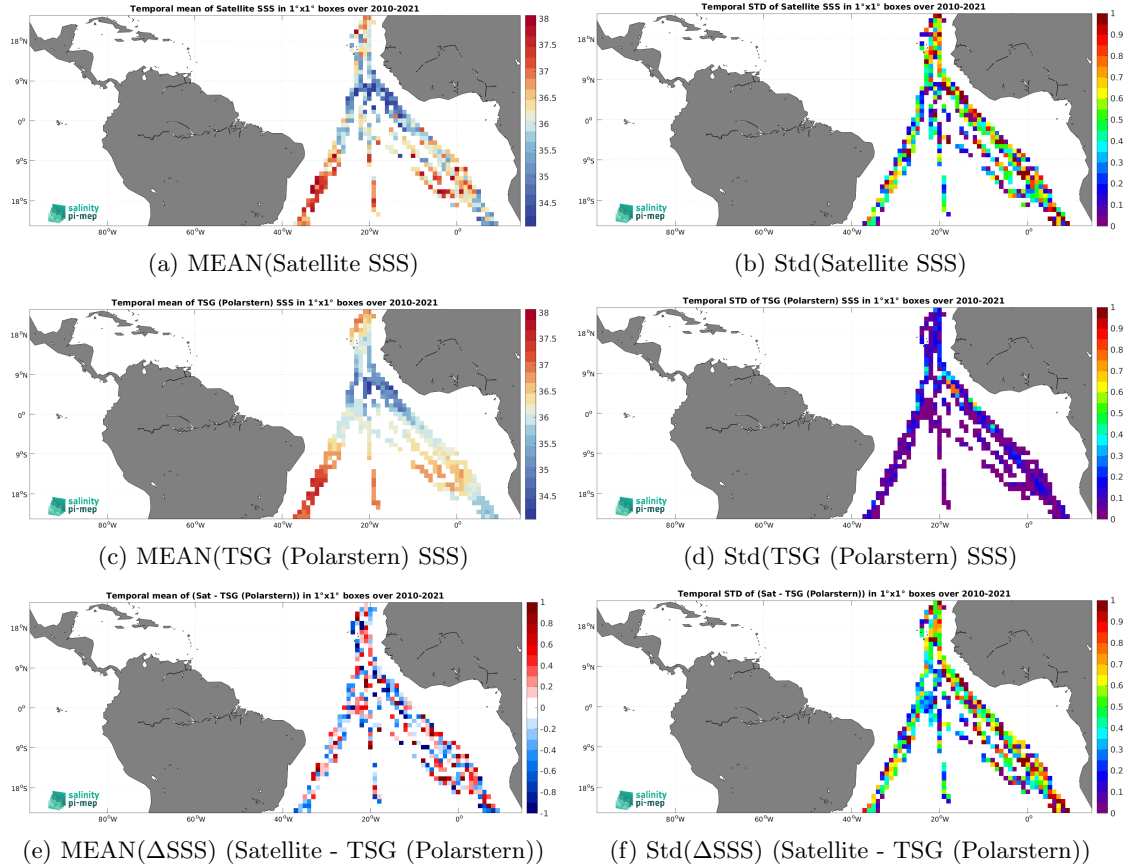
Figure 6: Temporal mean (left) and Std (right) of SSS from SMOS SSS L2Q v331 - No FLAG (CMEMS-CATDS-CPDC) (top), TSG (Polarstern) (middle), and of \Delta\text{SSS} (Satellite - TSG (Polarstern)). Only match-up pairs are used to generate these maps.
