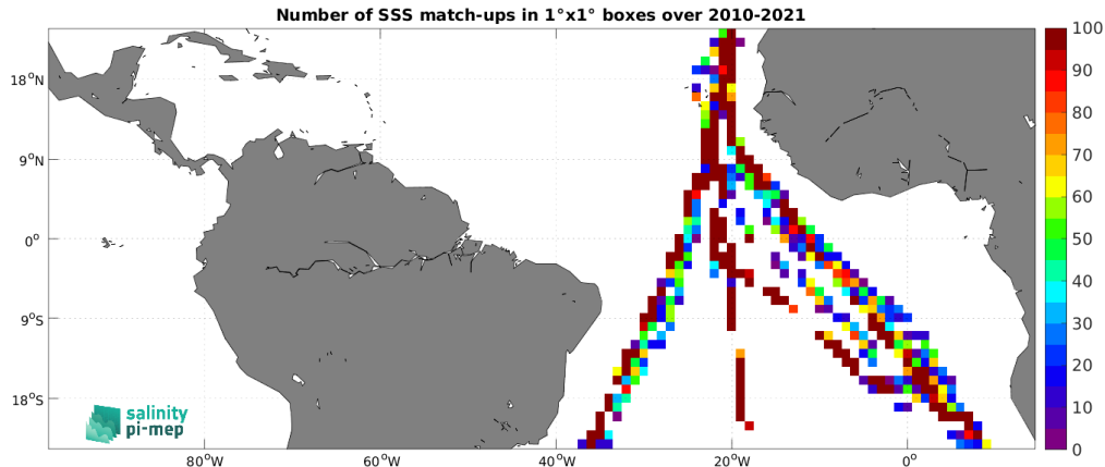
Figure 4: Number of SSS match-ups between TSG (Polarstern) SSS and the SMOS SSS L2Q v331 - No FLAG (CMEMS-CATDS-CPDC) SSS product for the Tropical Atlantic Ocean Pi-MEP region over 1^\circ \times 1^\circ boxes and for the full satellite product period.
