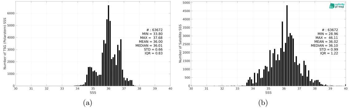
Figure 2: Histograms of SSS from TSG (Polarstern) (a) and SMOS SSS L2Q v331 - No FLAG (CMEMS-CATDS-CPDC) (b) considering all match-up pairs per bins of 0.1 over the Tropical Atlantic Ocean Pi-MEP region and for the full satellite product period.
