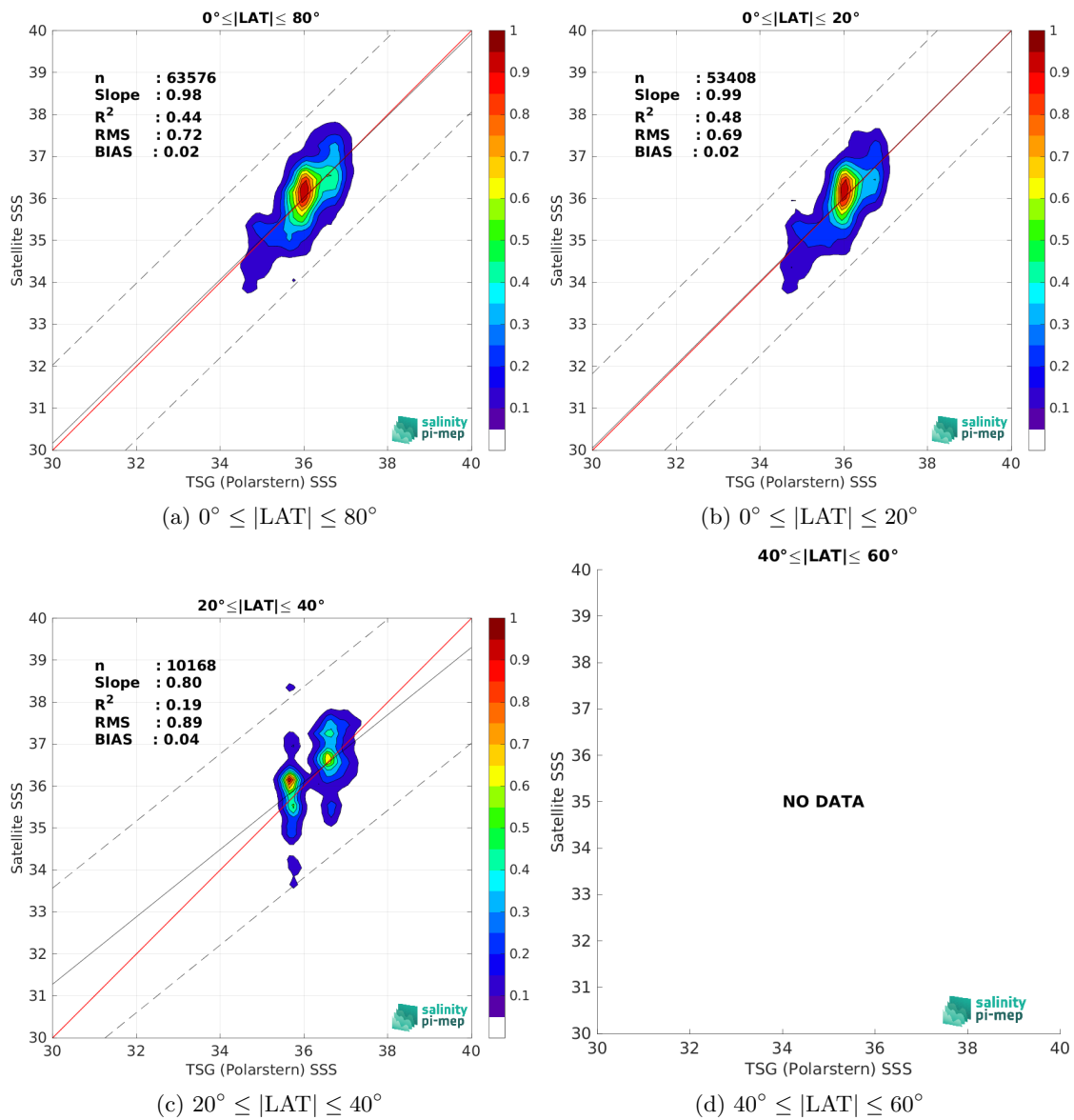
Figure 9: Contour maps of the concentration of SMOS SSS L2Q v331 - No FLAG (CMEMS-CATDS-CPDC) SSS (y-axis) versus TSG (Polarstern) SSS (x-axis) at match-up pairs for different latitude bands. For each plot, the red line shows x=y . The black thin and dashed lines indicate a linear fit through the data cloud and the \pm 95\% confidence levels, respectively. The number match-up pairs n , the slope and R^2 coefficient of the linear fit, the root mean square (RMS) and the mean bias between satellite and in situ data are indicated for each latitude band in each plots.
