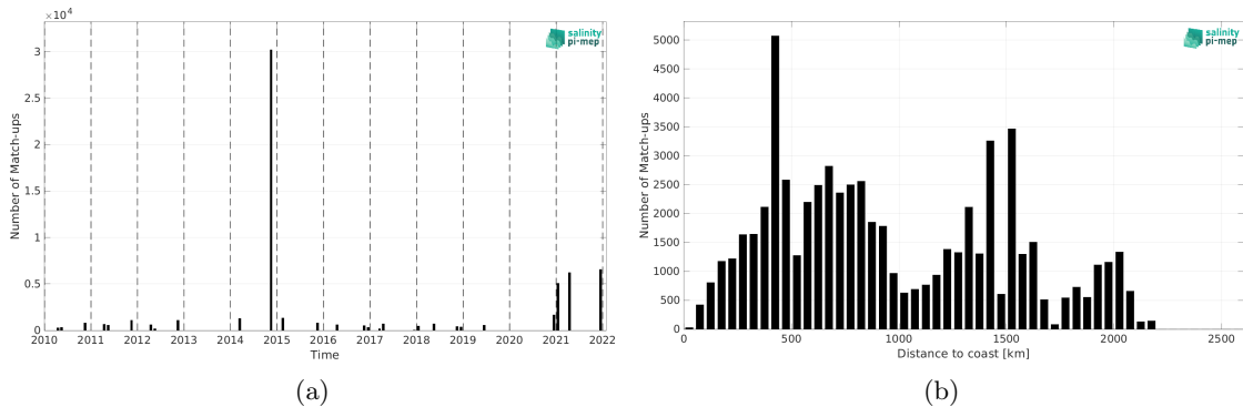
Figure 1: Number of match-ups between TSG (Polarstern) and SMOS SSS L2Q v331 - No FLAG (CMEMS-CATDS-CPDC) SSS as a function of time (a) and as function of the distance to coast (b) over the Tropical Atlantic Ocean Pi-MEP region and for the full satellite product period.
