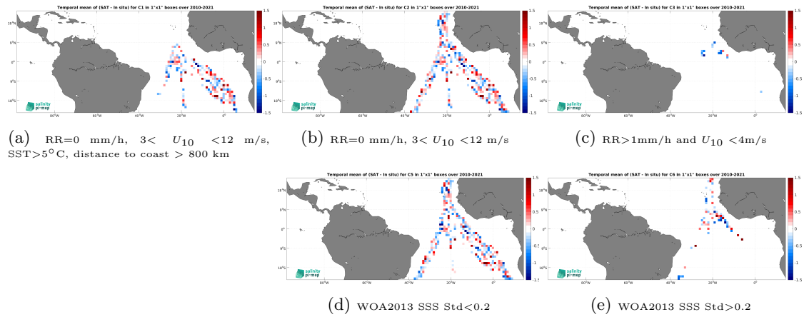
Figure 12: Temporal mean gridded over spatial boxes of size 1^{\circ}\times 1^{\circ} of \Delta\text{SSS} (SMOS SSS L2Q v331 - No FLAG (CMEMS-CATDS-CPDC) - TSG (Polarstern)) for 5 different subdatasets corresponding to:RR=0 mm/h, 3 < U_{10} < 12 m/s, SST > 5^{\circ}\text{C} , distance to coast > 800 km (a), RR=0 mm/h, 3 < U_{10} < 12 m/s (b), RR > 1 mm/h and U_{10} < 4 m/s (c), WOA2013 SSS Std < 0.2 (d), WOA2013 SSS Std > 0.2 (e).
