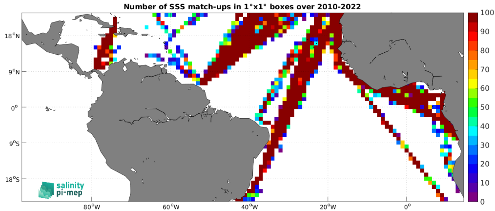
Figure 5: Number of SSS match-ups between TSG (LEGOS-DM) SSS and the SMOS SSS L2Q v331 - No FLAG (CMEMS-CATDS-CPDC) SSS product for the Tropical Atlantic Ocean Pi-MEP region over 1^\circ \times 1^\circ boxes and for the full satellite product period.
