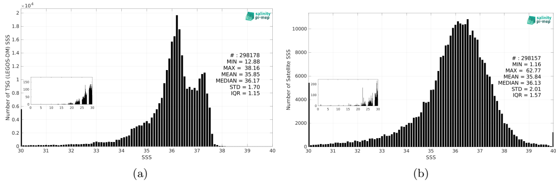
Figure 3: Histograms of SSS from TSG (LEGOS-DM) (a) and SMOS SSS L2Q v331 - No FLAG (CMEMS-CATDS-CPDC) (b) considering all match-up pairs per bins of 0.1 over the Tropical Atlantic Ocean Pi-MEP region and for the full satellite product period.
