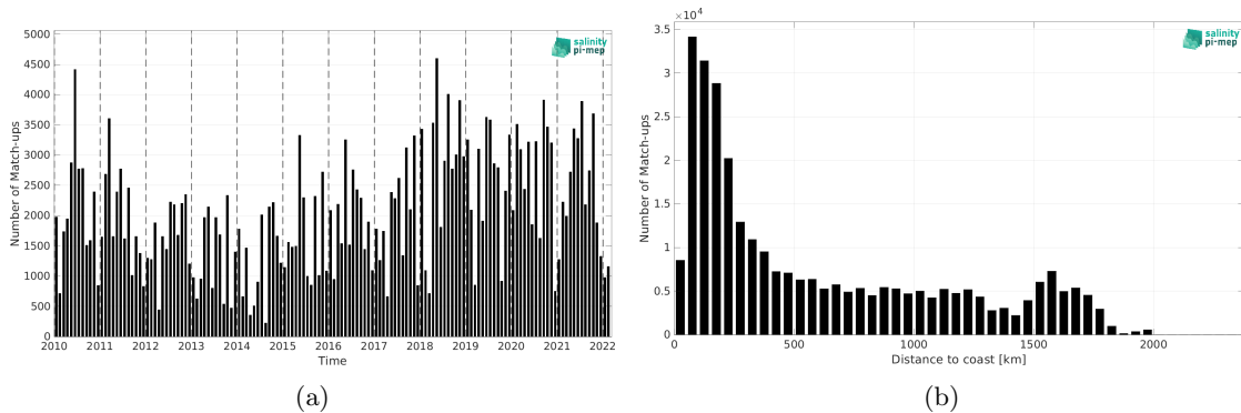
Figure 2: Number of match-ups between TSG (LEGOS-DM) and SMOS SSS L2Q v331 - No FLAG (CMEMS-CATDS-CPDC) SSS as a function of time (a) and as function of the distance to coast (b) over the Tropical Atlantic Ocean Pi-MEP region and for the full satellite product period.
