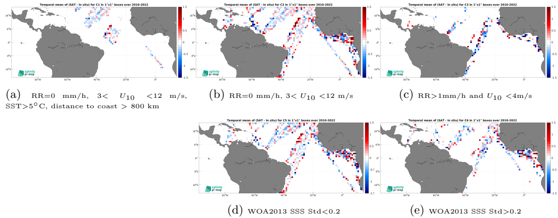
Figure 12: Temporal mean gridded over spatial boxes of size 1^\circ \times 1^\circ of \Delta\text{SSS} (SMOS SSS L2Q v331 - No FLAG (CMEMS-CATDS-CPDC) - TSG (LEGOS-DM)) for 5 different subdatasets corresponding to:RR=0 mm/h, 3 < U_{10} < 12 m/s, SST >5^\circ\text{C} , distance to coast > 800 km (a), RR=0 mm/h, 3 < U_{10} < 12 m/s (b), RR >1 mm/h and U_{10} < 4 m/s (c), WOA2013 SSS Std <0.2 (d), WOA2013 SSS Std >0.2 (e).
