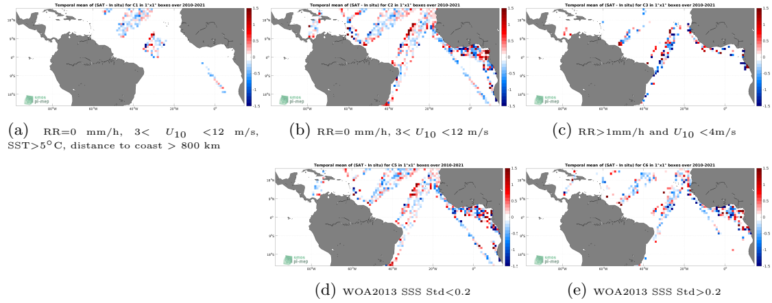
Figure 12: Temporal mean gridded over spatial boxes of size 1^{\circ}\times 1^{\circ} of \Delta\text{SSS} (SMOS SSS L2Q v331 - No FLAG (CMEMS-CATDS-CPDC) - TSG (LEGOS-DM)) for 5 different subdatasets corresponding to:RR=0 mm/h, 3 < U_{10} < 12 m/s, SST > 5^{\circ}\text{C} , distance to coast > 800 km (a), RR=0 mm/h, 3 < U_{10} < 12 m/s (b), RR > 1 mm/h and U_{10} < 4 m/s (c), WOA2013 SSS Std < 0.2 (d), WOA2013 SSS Std > 0.2 (e).
