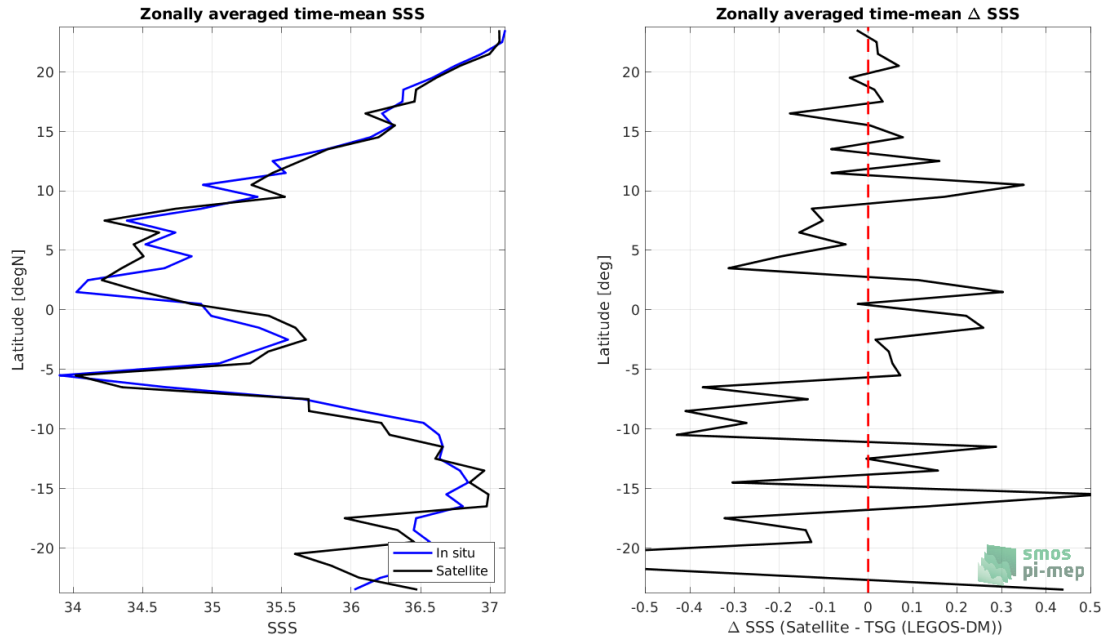
Figure 8: Left panel: Zonal mean SSS from SMOS SSS L2Q v331 - No FLAG (CMEMS-CATDS-CPDC) satellite product (black) and from TSG (LEGOS-DM) (blue). Right panel: Zonal mean of \Delta SSS (Satellite - TSG (LEGOS-DM)) for all the collected Pi-MEP match-up pairs estimated over the full satellite product period.
