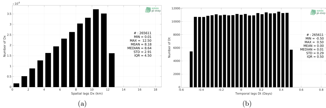
Figure 5: Histograms of the spatial (a) and temporal (b) lags between the location/time of the TSG (LEGOS-DM) measurement and the date of the corresponding SMOS SSS L2Q v331 - No FLAG (CMEMS-CATDS-CPDC) SSS pixel.
