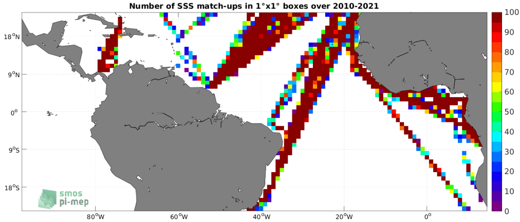
Figure 4: Number of SSS match-ups between TSG (LEGOS-DM) SSS and the SMOS SSS L2Q v331 - No FLAG (CMEMS-CATDS-CPDC) SSS product for the Tropical Atlantic Ocean Pi-MEP region over 1^\circ \times 1^\circ boxes and for the full satellite product period.
