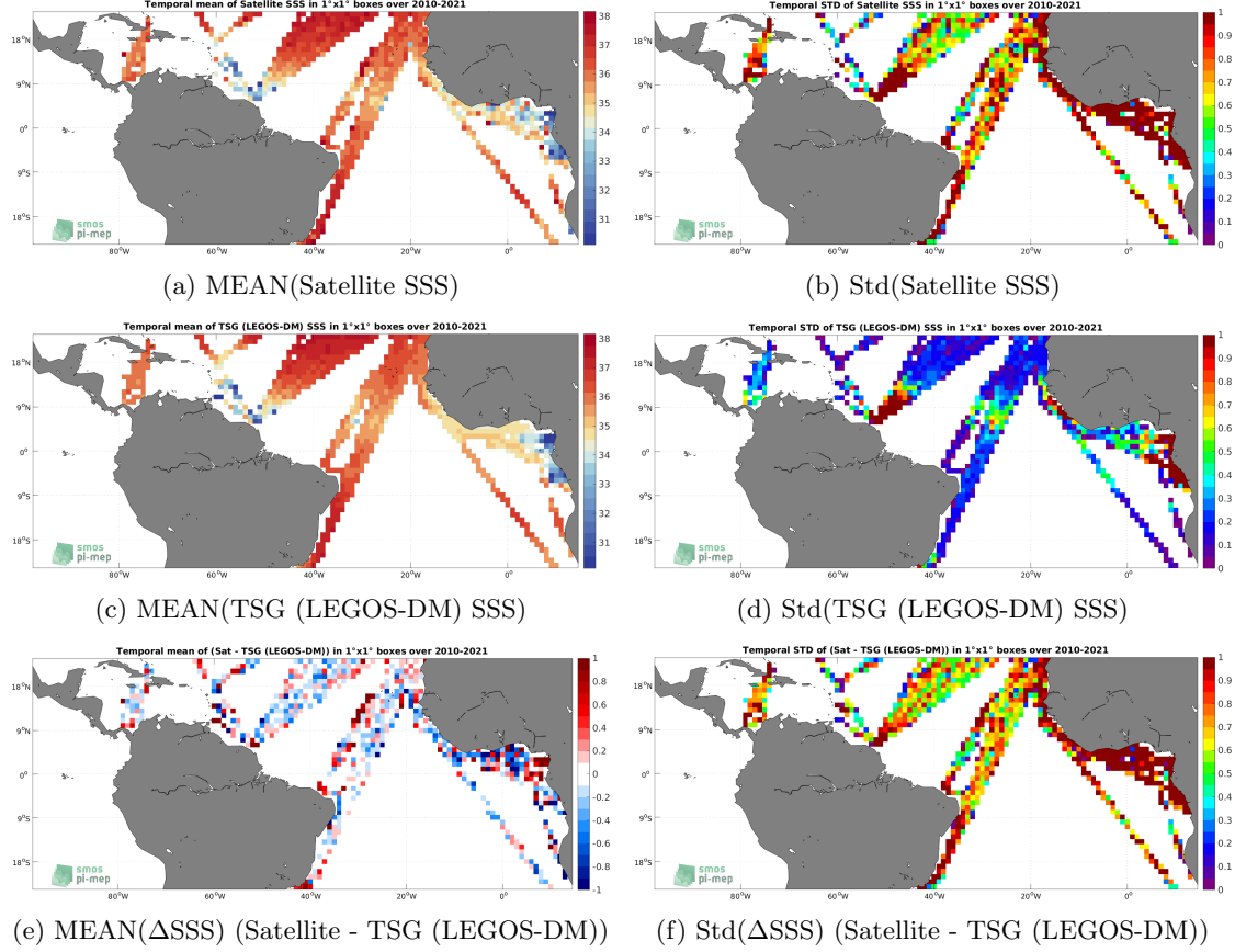
Figure 6: Temporal mean (left) and Std (right) of SSS from SMOS SSS L2Q v331 - No FLAG (CMEMS-CATDS-CPDC) (top), TSG (LEGOS-DM) (middle), and of \Delta\text{SSS} (Satellite - TSG (LEGOS-DM)). Only match-up pairs are used to generate these maps.
