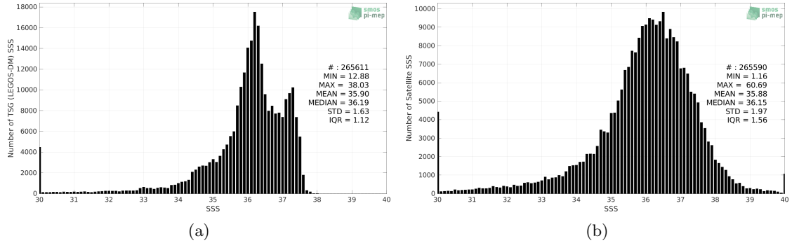
Figure 2: Histograms of SSS from TSG (LEGOS-DM) (a) and SMOS SSS L2Q v331 - No FLAG (CMEMS-CATDS-CPDC) (b) considering all match-up pairs per bins of 0.1 over the Tropical Atlantic Ocean Pi-MEP region and for the full satellite product period.
