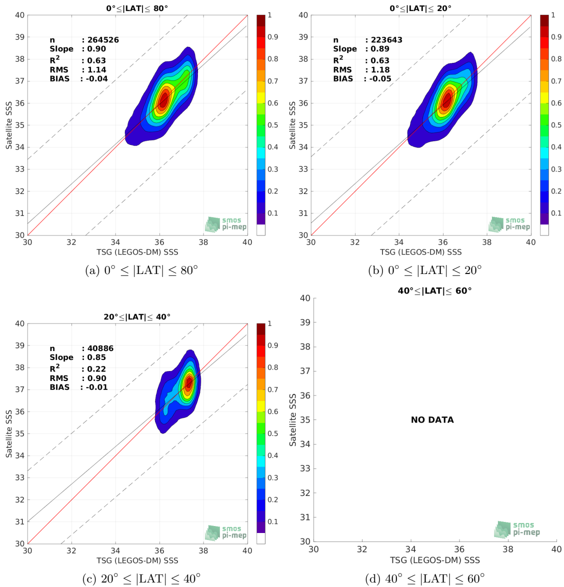
Figure 9: Contour maps of the concentration of SMOS SSS L2Q v331 - No FLAG (CMEMS-CATDS-CPDC) SSS (y-axis) versus TSG (LEGOS-DM) SSS (x-axis) at match-up pairs for different latitude bands. For each plot, the red line shows x=y . The black thin and dashed lines indicate a linear fit through the data cloud and the \pm 95\% confidence levels, respectively. The number match-up pairs n , the slope and R^2 coefficient of the linear fit, the root mean square (RMS) and the mean bias between satellite and in situ data are indicated for each latitude band in each plots.
