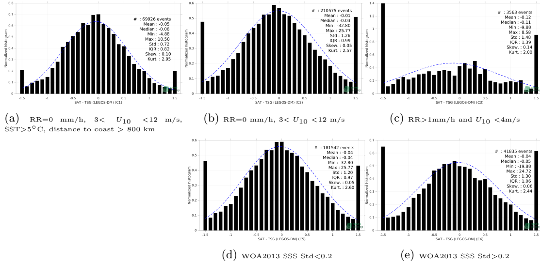
Figure 13: Normalized histogram of \Delta SSS (SMOS SSS L2Q v331 - No FLAG (CMEMS-CATDS-CPDC) - TSG (LEGOS-DM)) for 5 different subdatasets corresponding to: RR=0 mm/h, 3 < U_{10} < 12 m/s, SST>5°C, distance to coast > 800 km (a), RR=0 mm/h, 3 < U_{10} < 12 m/s (b), RR>1mm/h and U_{10} < 4 m/s (c), WOA2013 SSS Std<0.2 (d), WOA2013 SSS Std>0.2 (e).
