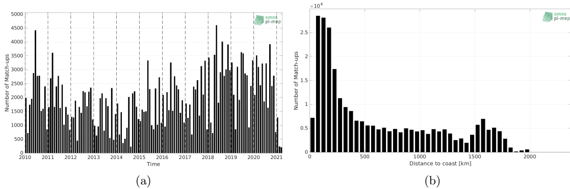
Figure 1: Number of match-ups between TSG (LEGOS-DM) and SMOS SSS L2Q v331 - No FLAG (CMEMS-CATDS-CPDC) SSS as a function of time (a) and as function of the distance to coast (b) over the Tropical Atlantic Ocean Pi-MEP region and for the full satellite product period.
