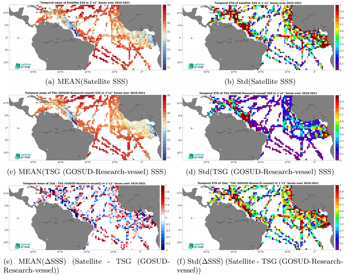
Figure 7: Temporal mean (left) and Std (right) of SSS from SMOS SSS L2Q v331 - No FLAG (CMEMS-CATDS-CPDC) (top), TSG (GOSUD-Research-vessel) (middle), and of \Delta\text{SSS} (Satellite - TSG (GOSUD-Research-vessel)). Only match-up pairs are used to generate these maps.
