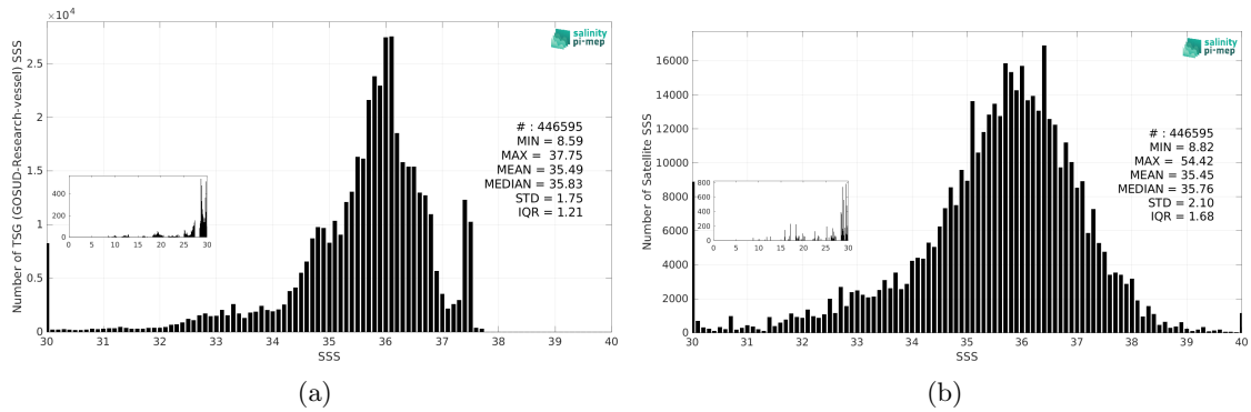
Figure 3: Histograms of SSS from TSG (GOSUD-Research-vessel) (a) and SMOS SSS L2Q v331 - No FLAG (CMEMS-CATDS-CPDC) (b) considering all match-up pairs per bins of 0.1 over the Tropical Atlantic Ocean Pi-MEP region and for the full satellite product period.
