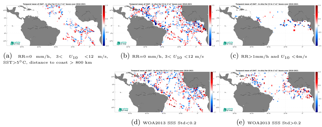
Figure 12: Temporal mean gridded over spatial boxes of size 1^\circ \times 1^\circ of \Delta SSS (SMOS SSS L2Q v331 - No FLAG (CMEMS-CATDS-CPDC) - TSG (GOSUD-Research-vessel)) for 5 different subdatasets corresponding to:RR=0 mm/h, 3 < U_{10} < 12 m/s, SST >5^\circ\text{C} , distance to coast > 800 km (a), RR=0 mm/h, 3 < U_{10} < 12 m/s (b), RR >1 mm/h and U_{10} < 4 m/s (c), WOA2013 SSS Std <0.2 (d), WOA2013 SSS Std >0.2 (e).
