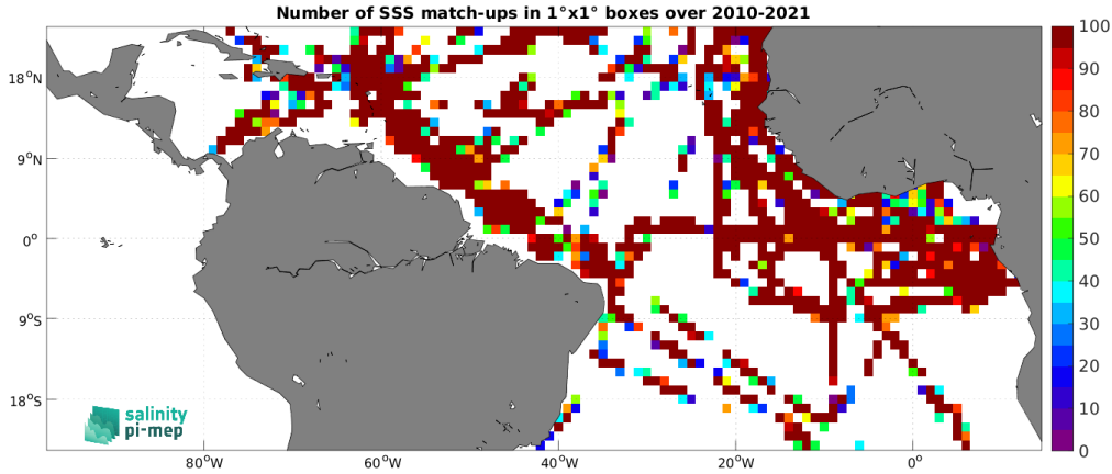
Figure 4: Number of SSS match-ups between TSG (GOSUD-Research-vessel) SSS and the SMOS SSS L2Q v331 - No FLAG (CMEMS-CATDS-CPDC) SSS product for the Tropical Atlantic Ocean Pi-MEP region over 1^\circ \times 1^\circ boxes and for the full satellite product period.
