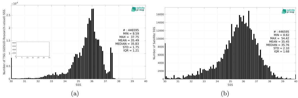
Figure 2: Histograms of SSS from TSG (GOSUD-Research-vessel) (a) and SMOS SSS L2Q v331 - No FLAG (CMEMS-CATDS-CPDC) (b) considering all match-up pairs per bins of 0.1 over the Tropical Atlantic Ocean Pi-MEP region and for the full satellite product period.
