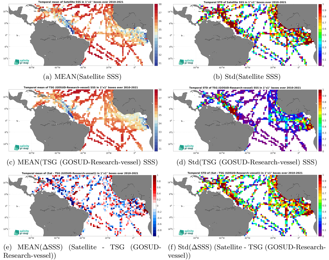
Figure 6: Temporal mean (left) and Std (right) of SSS from SMOS SSS L2Q v331 - No FLAG (CMEMS-CATDS-CPDC) (top), TSG (GOSUD-Research-vessel) (middle), and of \Delta\text{SSS} (Satellite - TSG (GOSUD-Research-vessel)). Only match-up pairs are used to generate these maps.
