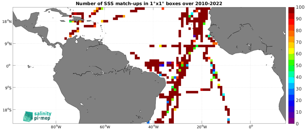
Figure 5: Number of SSS match-ups between TSG (CSIC-UTM) SSS and the SMOS SSS L2Q v331 - No FLAG (CMEMS-CATDS-CPDC) SSS product for the Tropical Atlantic Ocean Pi-MEP region over 1^\circ \times 1^\circ boxes and for the full satellite product period.
