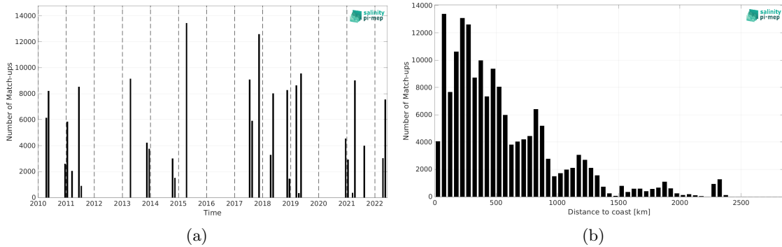
Figure 2: Number of match-ups between TSG (CSIC-UTM) and SMOS SSS L2Q v331 - No FLAG (CMEMS-CATDS-CPDC) SSS as a function of time (a) and as function of the distance to coast (b) over the Tropical Atlantic Ocean Pi-MEP region and for the full satellite product period.
