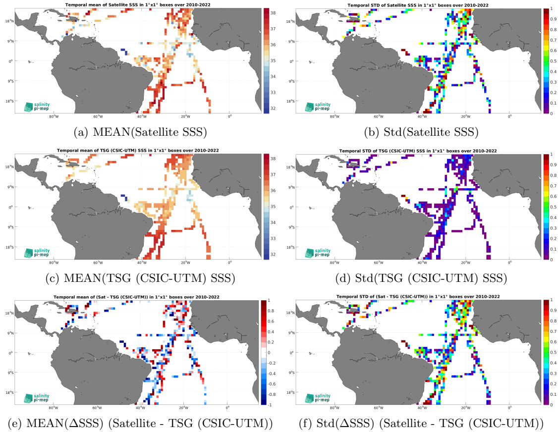
Figure 7: Temporal mean (left) and Std (right) of SSS from SMOS SSS L2Q v331 - No FLAG (CMEMS-CATDS-CPDC) (top), TSG (CSIC-UTM) (middle), and of \Delta\text{SSS} (Satellite - TSG (CSIC-UTM)). Only match-up pairs are used to generate these maps.
