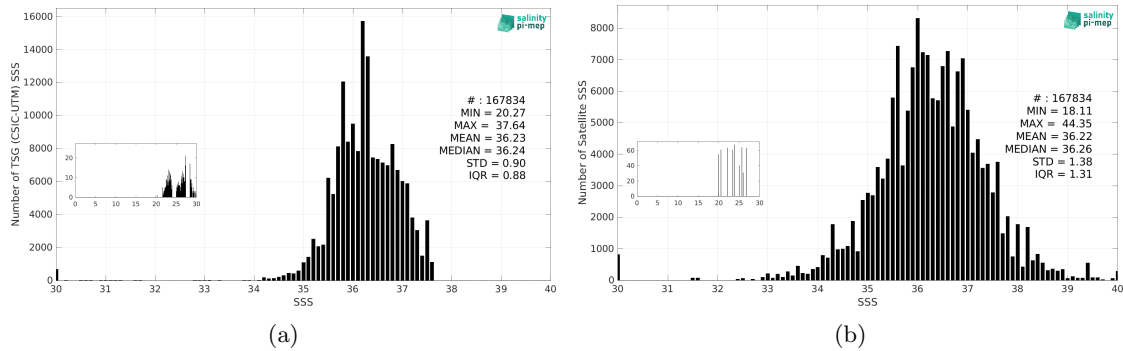
Figure 3: Histograms of SSS from TSG (CSIC-UTM) (a) and SMOS SSS L2Q v331 - No FLAG (CMEMS-CATDS-CPDC) (b) considering all match-up pairs per bins of 0.1 over the Tropical Atlantic Ocean Pi-MEP region and for the full satellite product period.
