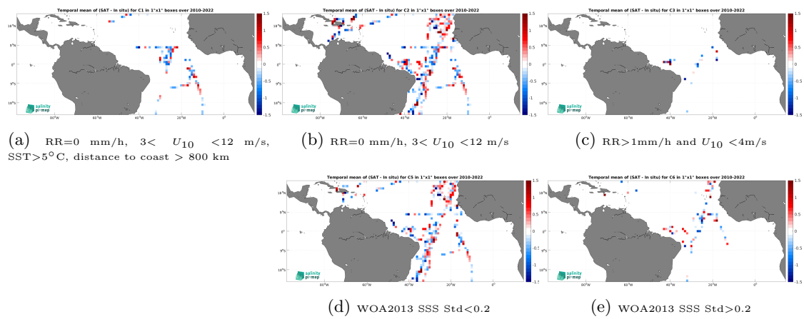
Figure 14: Temporal mean gridded over spatial boxes of size 1^\circ \times 1^\circ of \Delta SSS (SMOS SSS L2Q v331 - No FLAG (CMEMS-CATDS-CPDC) - TSG (CSIC-UTM)) for 5 different subdatasets corresponding to:RR=0 mm/h, 3 < U_{10} < 12 m/s, SST >5^\circ\text{C} , distance to coast > 800 km (a), RR=0 mm/h, 3 < U_{10} < 12 m/s (b), RR >1 mm/h and U_{10} < 4 m/s (c), WOA2013 SSS Std <0.2 (d), WOA2013 SSS Std >0.2 (e).
