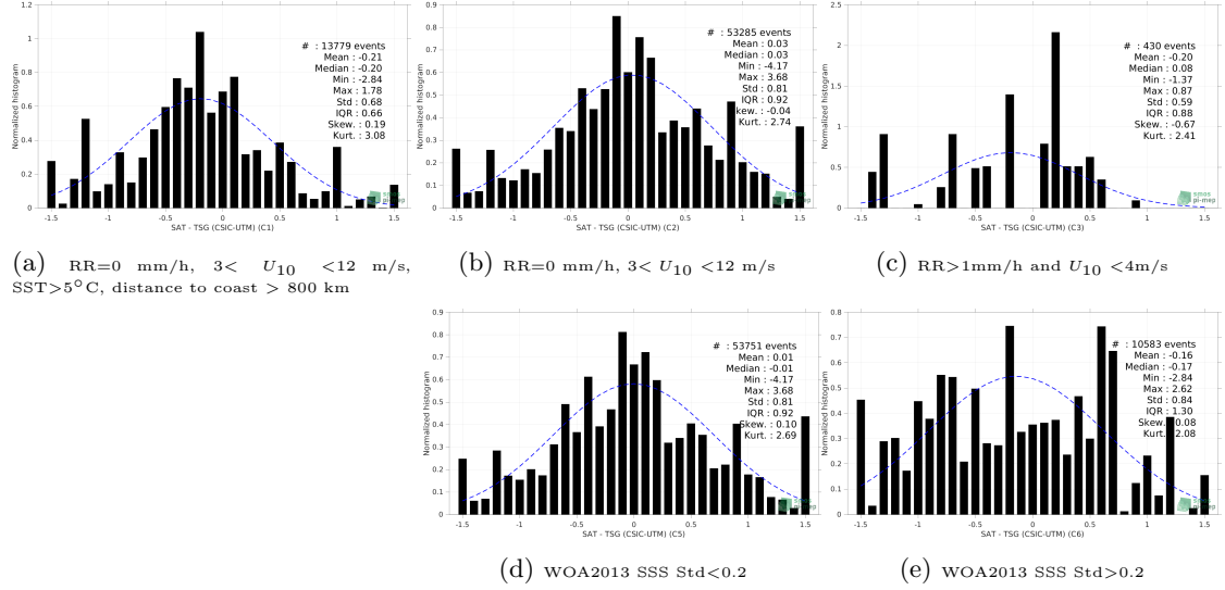
Figure 13: Normalized histogram of \Delta SSS (SMOS SSS L2Q v331 - No FLAG (CMEMS-CATDS-CPDC) - TSG (CSIC-UTM)) for 5 different subdatasets corresponding to: RR=0 mm/h, 3 < U_{10} < 12 m/s, SST>5°C, distance to coast > 800 km (a), RR=0 mm/h, 3 < U_{10} < 12 m/s (b), RR>1mm/h and U_{10} < 4 m/s (c), WOA2013 SSS Std<0.2 (d), WOA2013 SSS Std>0.2 (e).
