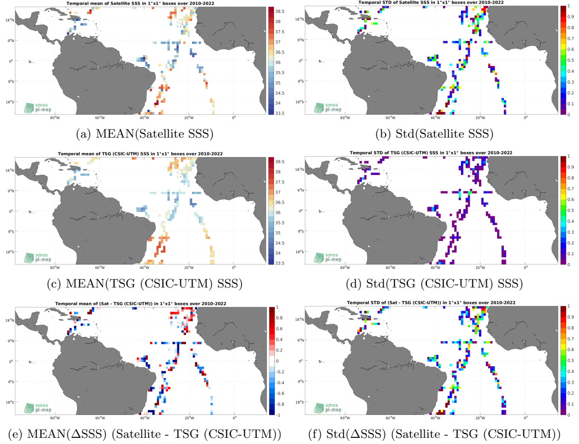
Figure 6: Temporal mean (left) and Std (right) of SSS from SMOS SSS L2Q v331 - No FLAG (CMEMS-CATDS-CPDC) (top), TSG (CSIC-UTM) (middle), and of \Delta\text{SSS} (Satellite - TSG (CSIC-UTM)). Only match-up pairs are used to generate these maps.
