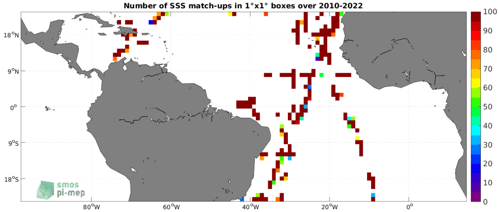
Figure 4: Number of SSS match-ups between TSG (CSIC-UTM) SSS and the SMOS SSS L2Q v331 - No FLAG (CMEMS-CATDS-CPDC) SSS product for the Tropical Atlantic Ocean Pi-MEP region over 1^\circ \times 1^\circ boxes and for the full satellite product period.
