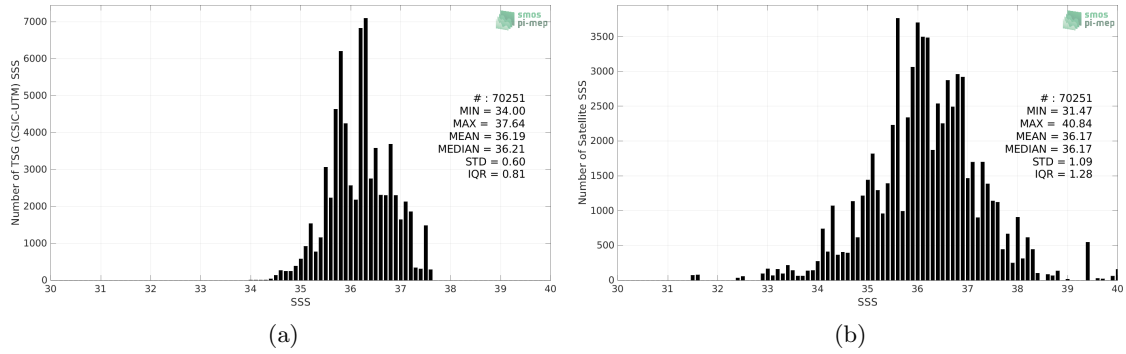
Figure 2: Histograms of SSS from TSG (CSIC-UTM) (a) and SMOS SSS L2Q v331 - No FLAG (CMEMS-CATDS-CPDC) (b) considering all match-up pairs per bins of 0.1 over the Tropical Atlantic Ocean Pi-MEP region and for the full satellite product period.
