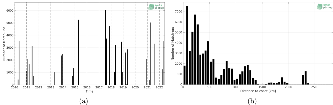
Figure 1: Number of match-ups between TSG (CSIC-UTM) and SMOS SSS L2Q v331 - No FLAG (CMEMS-CATDS-CPDC) SSS as a function of time (a) and as function of the distance to coast (b) over the Tropical Atlantic Ocean Pi-MEP region and for the full satellite product period.
