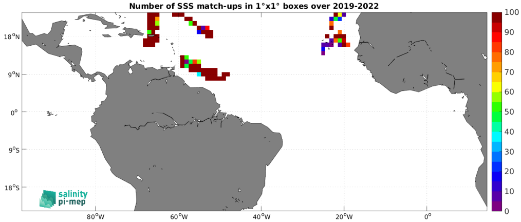
Figure 5: Number of SSS match-ups between Saildrone SSS and the SMOS SSS L2Q v331 - No FLAG (CMEMS-CATDS-CPDC) SSS product for the Tropical Atlantic Ocean Pi-MEP region over 1^\circ \times 1^\circ boxes and for the full satellite product period.
