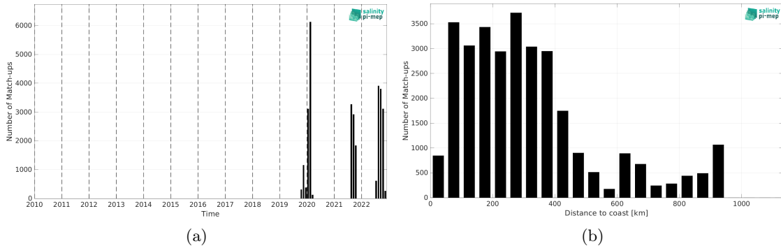
Figure 2: Number of match-ups between Saildrone and SMOS SSS L2Q v331 - No FLAG (CMEMS-CATDS-CPDC) SSS as a function of time (a) and as function of the distance to coast (b) over the Tropical Atlantic Ocean Pi-MEP region and for the full satellite product period.
