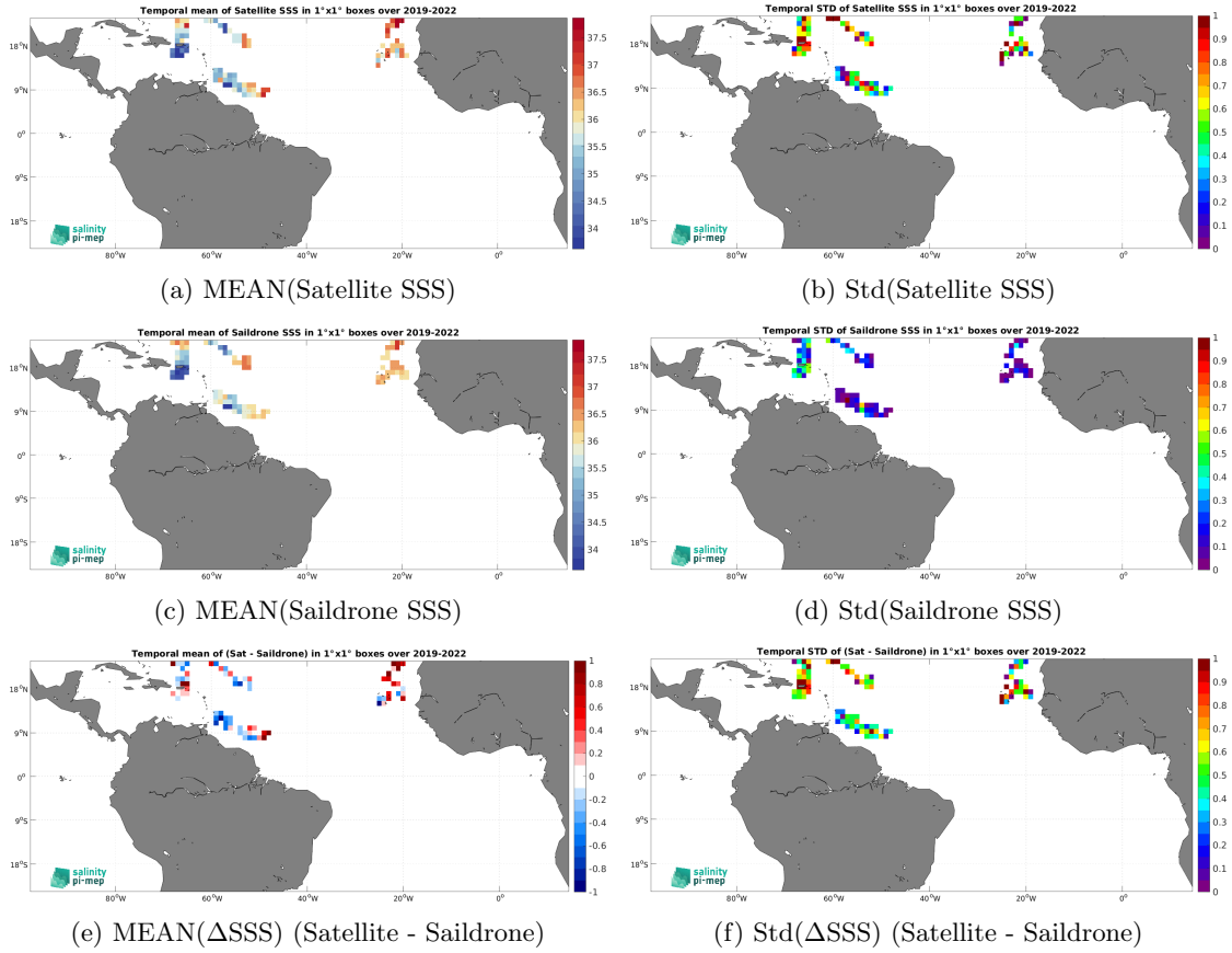
Figure 7: Temporal mean (left) and Std (right) of SSS from SMOS SSS L2Q v331 - No FLAG (CMEMS-CATDS-CPDC) (top), Sairdrone (middle), and of \Delta SSS (Satellite - Sairdrone). Only match-up pairs are used to generate these maps.
