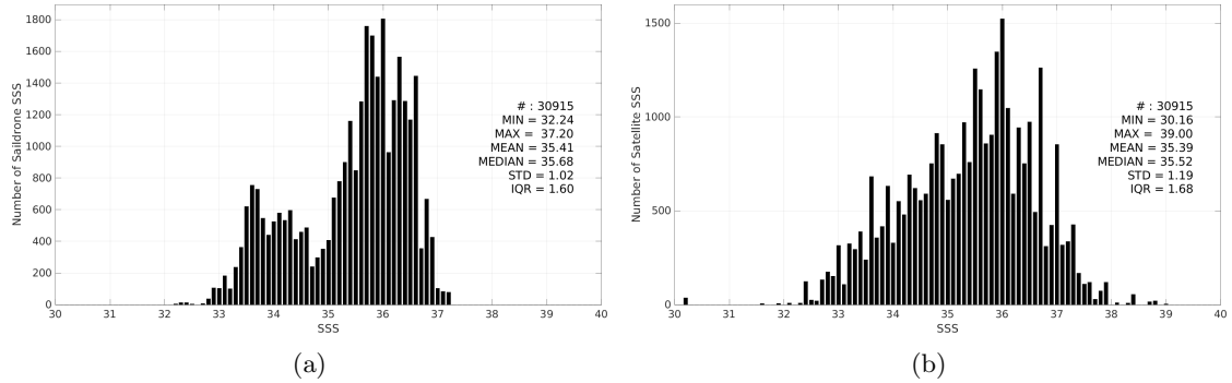
Figure 3: Histograms of SSS from Saildrone (a) and SMOS SSS L2Q v331 - No FLAG (CMEMS-CATDS-CPDC) (b) considering all match-up pairs per bins of 0.1 over the Tropical Atlantic Ocean Pi-MEP region and for the full satellite product period.
