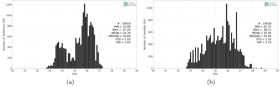
Figure 2: Histograms of SSS from Saildrone (a) and SMOS SSS L2Q v331 - No FLAG (CMEMS-CATDS-CPDC) (b) considering all match-up pairs per bins of 0.1 over the Tropical Atlantic Ocean Pi-MEP region and for the full satellite product period.
