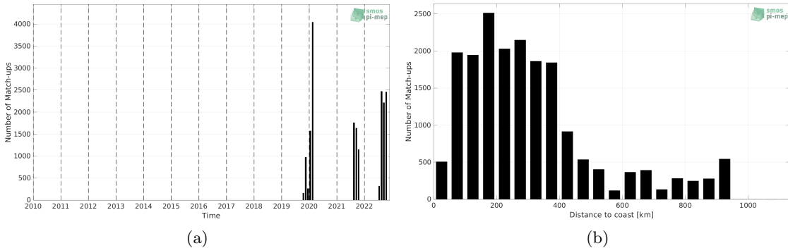
Figure 1: Number of match-ups between Saildrone and SMOS SSS L2Q v331 - No FLAG (CMEMS-CATDS-CPDC) SSS as a function of time (a) and as function of the distance to coast (b) over the Tropical Atlantic Ocean Pi-MEP region and for the full satellite product period.
