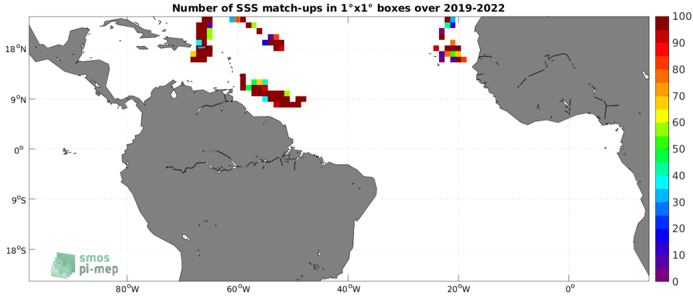
Figure 4: Number of SSS match-ups between Saildrone SSS and the SMOS SSS L2Q v331 - No FLAG (CMEMS-CATDS-CPDC) SSS product for the Tropical Atlantic Ocean Pi-MEP region over 1^\circ \times 1^\circ boxes and for the full satellite product period.
