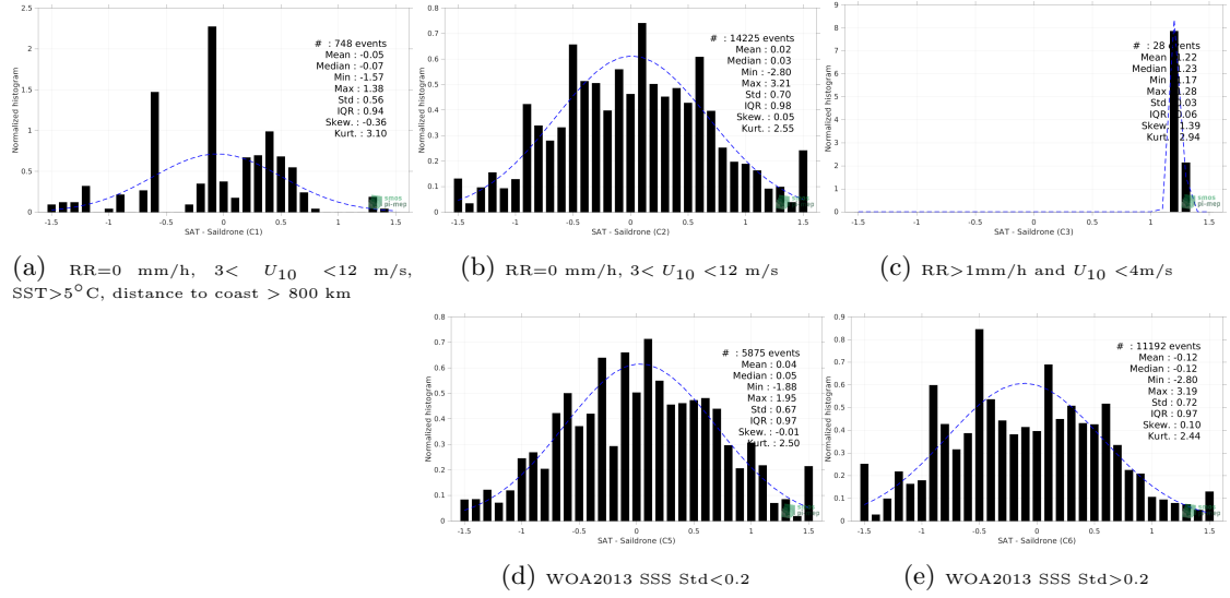
Figure 13: Normalized histogram of \Delta SSS (SMOS SSS L2Q v331 - No FLAG (CMEMS-CATDS-CPDC) - Saldrone) for 5 different subdatasets corresponding to: RR=0 mm/h, 3 < U_{10} < 12 m/s, SST > 5°C, distance to coast > 800 km (a), RR=0 mm/h, 3 < U_{10} < 12 m/s (b), RR > 1mm/h and U_{10} < 4 m/s (c), WOA2013 SSS Std < 0.2 (d), WOA2013 SSS Std > 0.2 (e).
