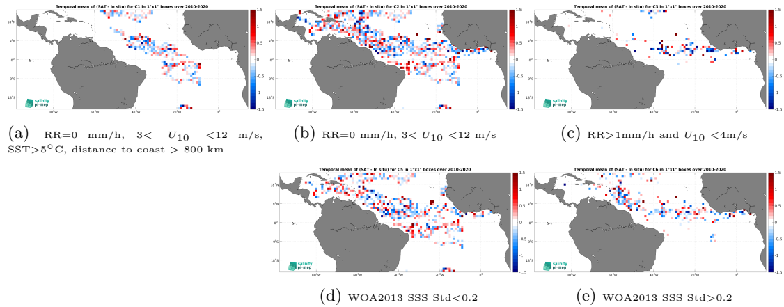
Figure 13: Temporal mean gridded over spatial boxes of size 1^\circ \times 1^\circ of \Delta SSS (SMOS SSS L2Q v331 - No FLAG (CMEMS-CATDS-CPDC) - Surface drifters) for 5 different subdatasets corresponding to:RR=0 mm/h, 3 < U_{10} < 12 m/s, SST >5^\circ\text{C} , distance to coast > 800 km (a), RR=0 mm/h, 3 < U_{10} < 12 m/s (b), RR >1 mm/h and U_{10} < 4 m/s (c), WOA2013 SSS Std <0.2 (d), WOA2013 SSS Std >0.2 (e).
