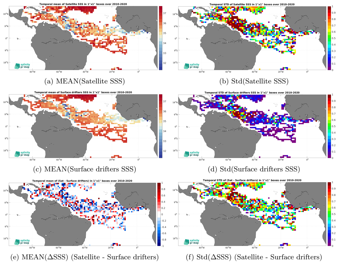
Figure 6: Temporal mean (left) and Std (right) of SSS from SMOS SSS L2Q v331 - No FLAG (CMEMS-CATDS-CPDC) (top), Surface drifters (middle), and of \Delta SSS (Satellite - Surface drifters). Only match-up pairs are used to generate these maps.
