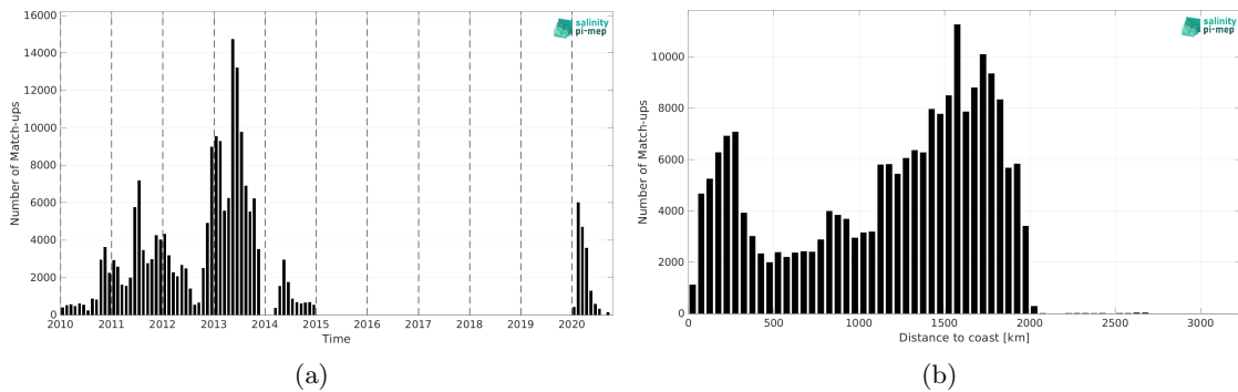
Figure 2: Number of match-ups between Surface drifters and SMOS SSS L2Q v331 - No FLAG (CMEMS-CATDS-CPDC) SSS as a function of time (a) and as function of the distance to coast (b) over the Tropical Atlantic Ocean Pi-MEP region and for the full satellite product period.
