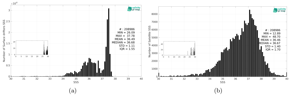
Figure 3: Histograms of SSS from Surface drifters (a) and SMOS SSS L2Q v331 - No FLAG (CMEMS-CATDS-CPDC) (b) considering all match-up pairs per bins of 0.1 over the Tropical Atlantic Ocean Pi-MEP region and for the full satellite product period.
