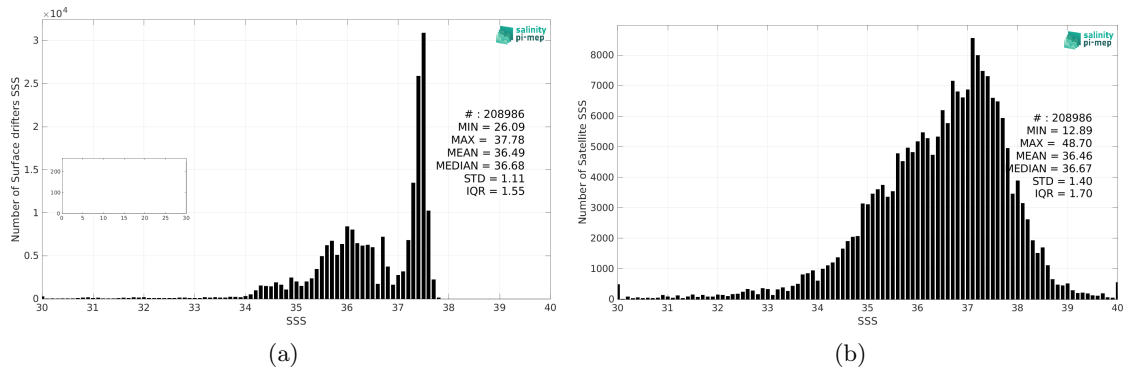
Figure 2: Histograms of SSS from Surface drifters (a) and SMOS SSS L2Q v331 - No FLAG (CMEMS-CATDS-CPDC) (b) considering all match-up pairs per bins of 0.1 over the Tropical Atlantic Ocean Pi-MEP region and for the full satellite product period.
