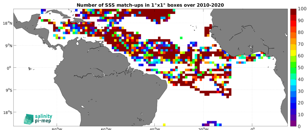
Figure 3: Number of SSS match-ups between Surface drifters SSS and the SMOS SSS L2Q v331 - No FLAG (CMEMS-CATDS-CPDC) SSS product for the Tropical Atlantic Ocean Pi-MEP region over 1^\circ \times 1^\circ boxes and for the full satellite product period.
