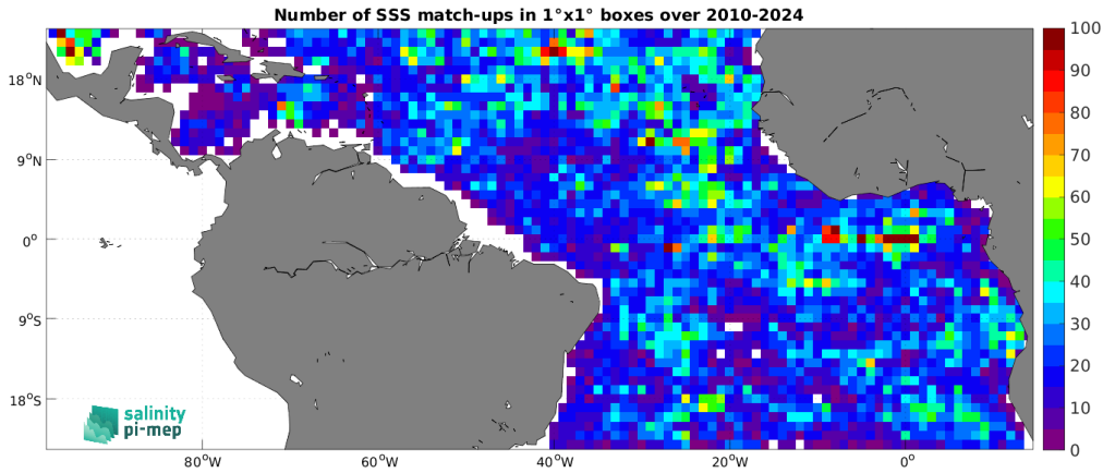
Figure 5: Number of SSS match-ups between Argo SSS and the SMOS SSS L2Q v331 - No FLAG (CMEMS-CATDS-CPDC) SSS product for the Tropical Atlantic Ocean Pi-MEP region over 1^\circ \times 1^\circ boxes and for the full satellite product period.
