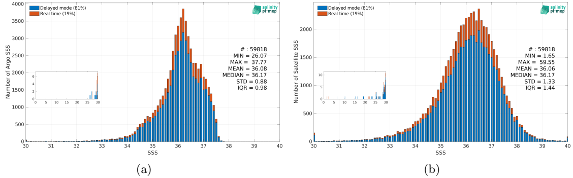
Figure 3: Histograms of SSS from Argo (a) and SMOS SSS L2Q v331 - No FLAG (CMEMS-CATDS-CPDC) (b) considering all match-up pairs per bins of 0.1 over the Tropical Atlantic Ocean Pi-MEP region and for the full satellite product period.
