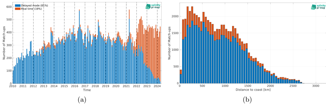
Figure 2: Number of match-ups between Argo and SMOS SSS L2Q v331 - No FLAG (CMEMS-CATDS-CPDC) SSS as a function of time (a) and as function of the distance to coast (b) over the Tropical Atlantic Ocean Pi-MEP region and for the full satellite product period.
