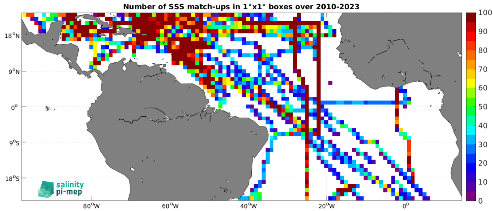
Figure 4: Number of SSS match-ups between TSG (SAMOS) SSS and the SMOS SSS L3 v9 - 9 Days (CATDS-CEC-LOCEAN) SSS product for the Tropical Atlantic Ocean Pi-MEP region over 1^\circ \times 1^\circ boxes and for the full satellite product period.
