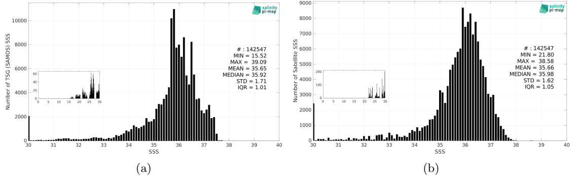
Figure 2: Histograms of SSS from TSG (SAMOS) (a) and SMOS SSS L3 v9 - 9 Days (CATDS-CEC-LOCEAN) (b) considering all match-up pairs per bins of 0.1 over the Tropical Atlantic Ocean Pi-MEP region and for the full satellite product period.
