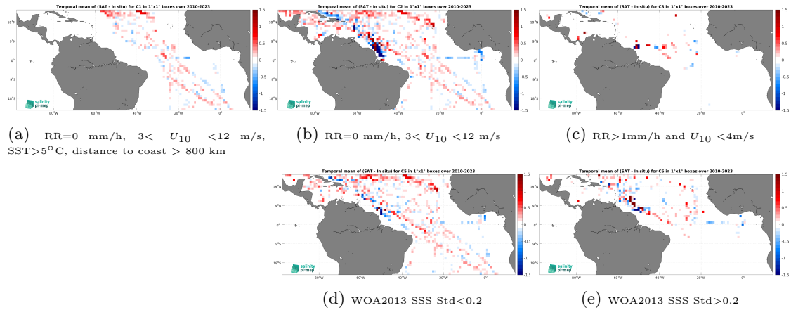
Figure 12: Temporal mean gridded over spatial boxes of size 1^\circ \times 1^\circ of \Delta\text{SSS} (SMOS SSS L3 v9 - 9 Days (CATDS-CEC-LOCEAN) - TSG (SAMOS)) for 5 different subdatasets corresponding to:RR=0 mm/h, 3 < U_{10} < 12 m/s, SST >5^\circ\text{C} , distance to coast > 800 km (a), RR=0 mm/h, 3 < U_{10} < 12 m/s (b), RR >1 mm/h and U_{10} < 4 m/s (c), WOA2013 SSS Std <0.2 (d), WOA2013 SSS Std >0.2 (e).
