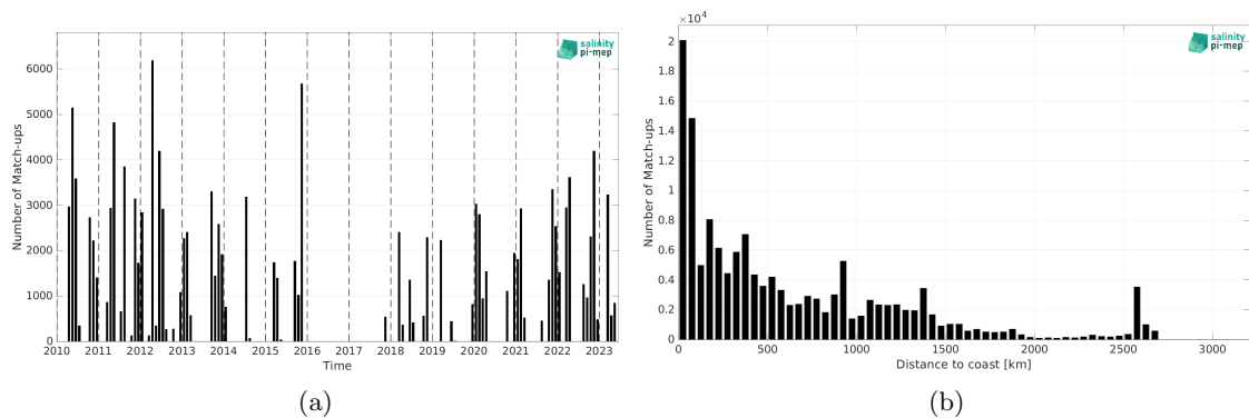
Figure 1: Number of match-ups between TSG (SAMOS) and SMOS SSS L3 v9 - 9 Days (CATDS-CEC-LOCEAN) SSS as a function of time (a) and as function of the distance to coast (b) over the Tropical Atlantic Ocean Pi-MEP region and for the full satellite product period.
