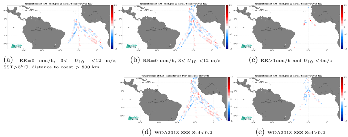
Figure 14: Temporal mean gridded over spatial boxes of size 1^\circ \times 1^\circ of \Delta\text{SSS} (SMOS SSS L3 v9 - 9 Days (CATDS-CEC-LOCEAN) - TSG (Polarstern)) for 5 different subdatasets corresponding to:RR=0 mm/h, 3 < U_{10} < 12 m/s, SST >5^\circ\text{C} , distance to coast > 800 km (a), RR=0 mm/h, 3 < U_{10} < 12 m/s (b), RR >1 mm/h and U_{10} < 4 m/s (c), WOA2013 SSS Std <0.2 (d), WOA2013 SSS Std >0.2 (e).
