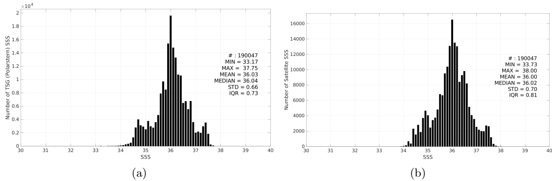
Figure 3: Histograms of SSS from TSG (Polarstern) (a) and SMOS SSS L3 v9 - 9 Days (CATDS-CEC-LOCEAN) (b) considering all match-up pairs per bins of 0.1 over the Tropical Atlantic Ocean Pi-MEP region and for the full satellite product period.
