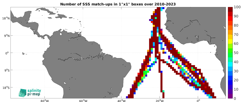
Figure 5: Number of SSS match-ups between TSG (Polarstern) SSS and the SMOS SSS L3 v9 - 9 Days (CATDS-CEC-LOCEAN) SSS product for the Tropical Atlantic Ocean Pi-MEP region over 1^\circ \times 1^\circ boxes and for the full satellite product period.
