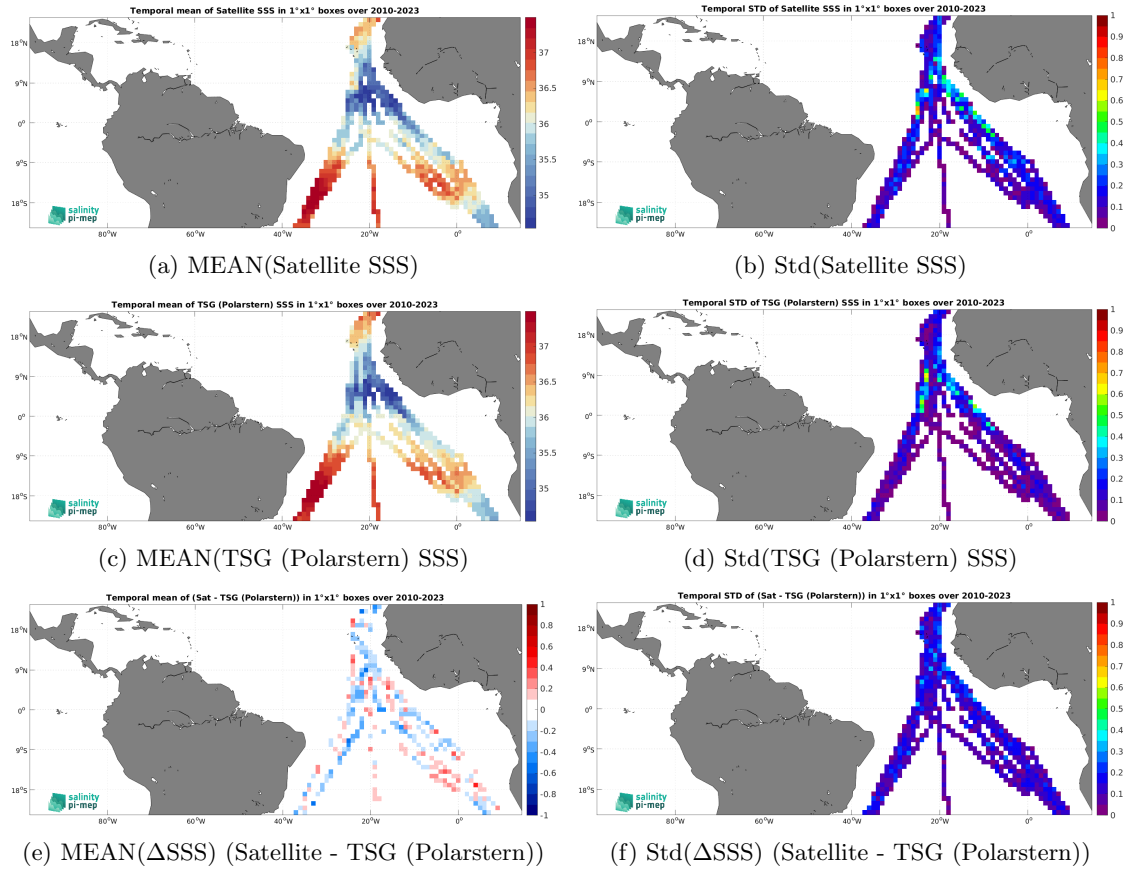
Figure 7: Temporal mean (left) and Std (right) of SSS from SMOS SSS L3 v9 - 9 Days (CATDS-CEC-LOCEAN) (top), TSG (Polarstern) (middle), and of \Delta SSS (Satellite - TSG (Polarstern)). Only match-up pairs are used to generate these maps.
