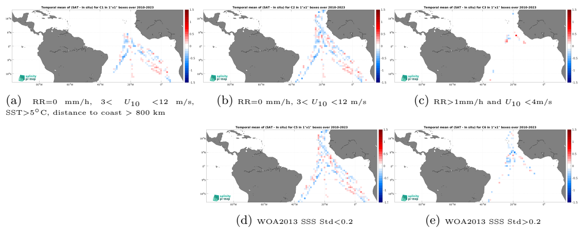
Figure 14: Temporal mean gridded over spatial boxes of size 1^\circ \times 1^\circ of \Delta\text{SSS} (SMOS SSS L3 v9 - 9 Days (CATDS-CEC-LOCEAN) - TSG (Polarstern)) for 5 different subdatasets corresponding to:RR=0 mm/h, 3 < U_{10} < 12 m/s, SST >5^\circ\text{C} , distance to coast > 800 km (a), RR=0 mm/h, 3 < U_{10} < 12 m/s (b), RR >1 mm/h and U_{10} < 4 m/s (c), WOA2013 SSS Std <0.2 (d), WOA2013 SSS Std >0.2 (e).
