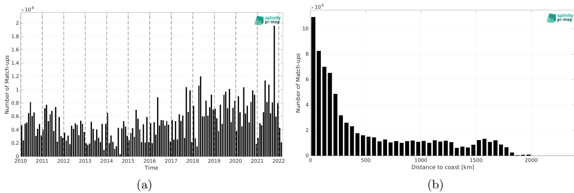
Figure 2: Number of match-ups between TSG (LEGOS-DM) and SMOS SSS L3 v9 - 9 Days (CATDS-CEC-LOCEAN) SSS as a function of time (a) and as function of the distance to coast (b) over the Tropical Atlantic Ocean Pi-MEP region and for the full satellite product period.
