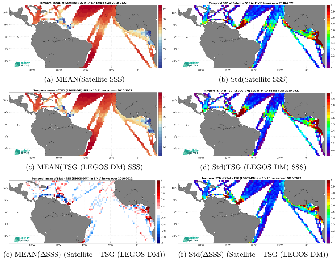
Figure 7: Temporal mean (left) and Std (right) of SSS from SMOS SSS L3 v9 - 9 Days (CATDS-CEC-LOCEAN) (top), TSG (LEGOS-DM) (middle), and of \Delta\text{SSS} (Satellite - TSG (LEGOS-DM)). Only match-up pairs are used to generate these maps.
