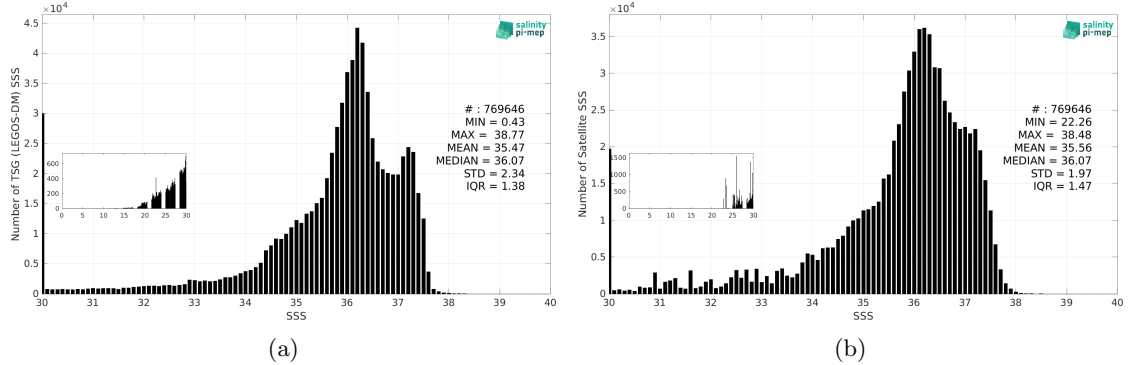
Figure 3: Histograms of SSS from TSG (LEGOS-DM) (a) and SMOS SSS L3 v9 - 9 Days (CATDS-CEC-LOCEAN) (b) considering all match-up pairs per bins of 0.1 over the Tropical Atlantic Ocean Pi-MEP region and for the full satellite product period.
