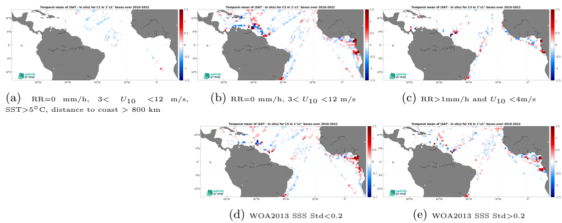
Figure 14: Temporal mean gridded over spatial boxes of size 1^\circ \times 1^\circ of \Delta SSS (SMOS SSS L3 v9 - 9 Days (CATDS-CEC-LOCEAN) - TSG (LEGOS-DM)) for 5 different subdatasets corresponding to:RR=0 mm/h, 3 < U_{10} < 12 m/s, SST >5^\circ\text{C} , distance to coast > 800 km (a), RR=0 mm/h, 3 < U_{10} < 12 m/s (b), RR >1 mm/h and U_{10} < 4 m/s (c), WOA2013 SSS Std <0.2 (d), WOA2013 SSS Std >0.2 (e).
