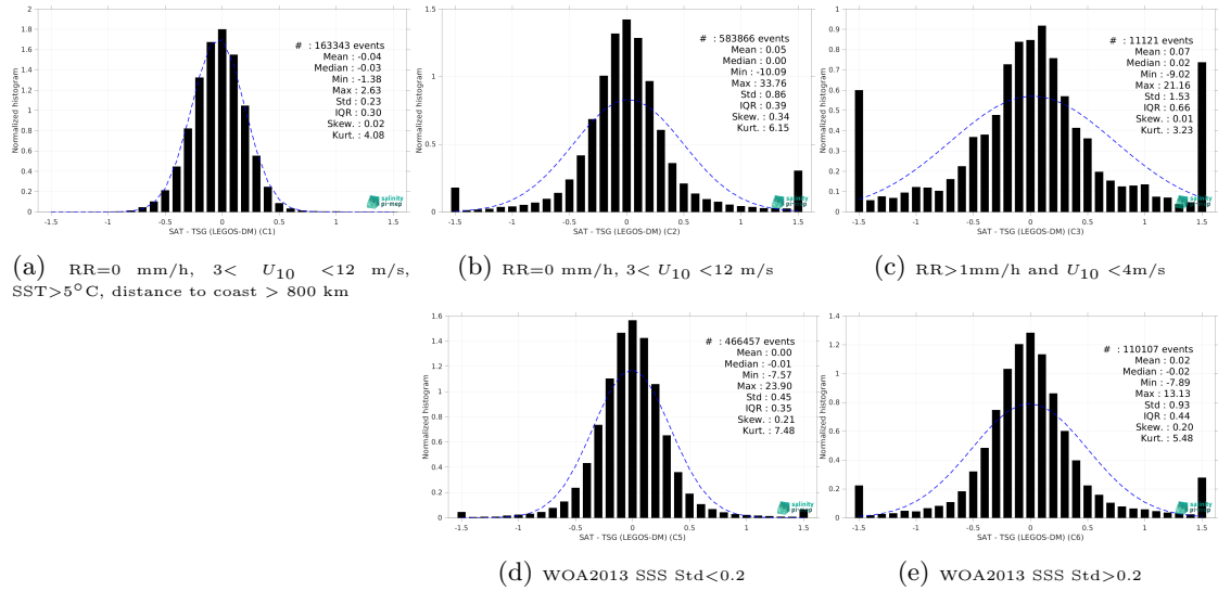
Figure 13: Normalized histogram of \Delta\text{SSS} (SMOS SSS L3 v9 - 9 Days (CATDS-CEC-LOCEAN) - TSG (LEGOS-DM)) for 5 different subdatasets corresponding to: RR=0 mm/h, 3 < U_{10} < 12 m/s, SST > 5^\circ\text{C} , distance to coast > 800 km (a), RR=0 mm/h, 3 < U_{10} < 12 m/s (b), RR > 1 mm/h and U_{10} < 4 m/s (c), WOA2013 SSS Std < 0.2 (d), WOA2013 SSS Std > 0.2 (e).
