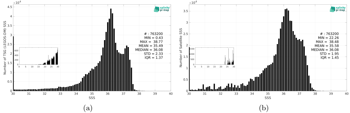
Figure 2: Histograms of SSS from TSG (LEGOS-DM) (a) and SMOS SSS L3 v9 - 9 Days (CATDS-CEC-LOCEAN) (b) considering all match-up pairs per bins of 0.1 over the Tropical Atlantic Ocean Pi-MEP region and for the full satellite product period.
