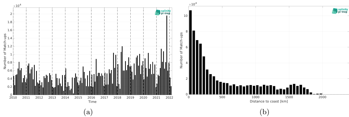
Figure 1: Number of match-ups between TSG (LEGOS-DM) and SMOS SSS L3 v9 - 9 Days (CATDS-CEC-LOCEAN) SSS as a function of time (a) and as function of the distance to coast (b) over the Tropical Atlantic Ocean Pi-MEP region and for the full satellite product period.
