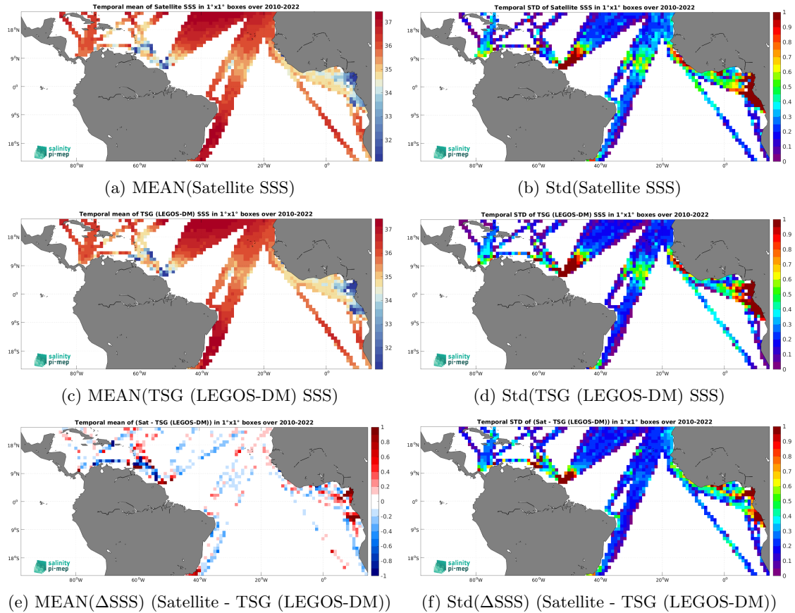
Figure 6: Temporal mean (left) and Std (right) of SSS from SMOS SSS L3 v9 - 9 Days (CATDS-CEC-LOCEAN) (top), TSG (LEGOS-DM) (middle), and of \Delta\text{SSS} (Satellite - TSG (LEGOS-DM)). Only match-up pairs are used to generate these maps.
