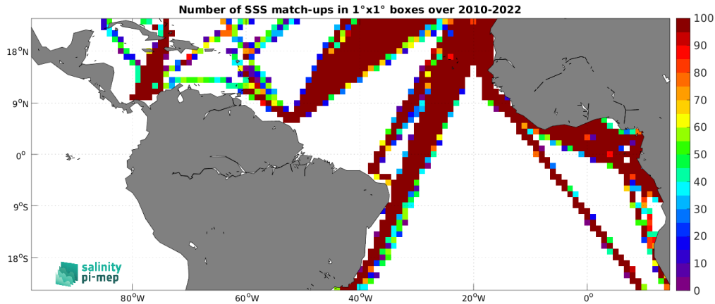
Figure 4: Number of SSS match-ups between TSG (LEGOS-DM) SSS and the SMOS SSS L3 v9 - 9 Days (CATDS-CEC-LOCEAN) SSS product for the Tropical Atlantic Ocean Pi-MEP region over 1^\circ \times 1^\circ boxes and for the full satellite product period.
