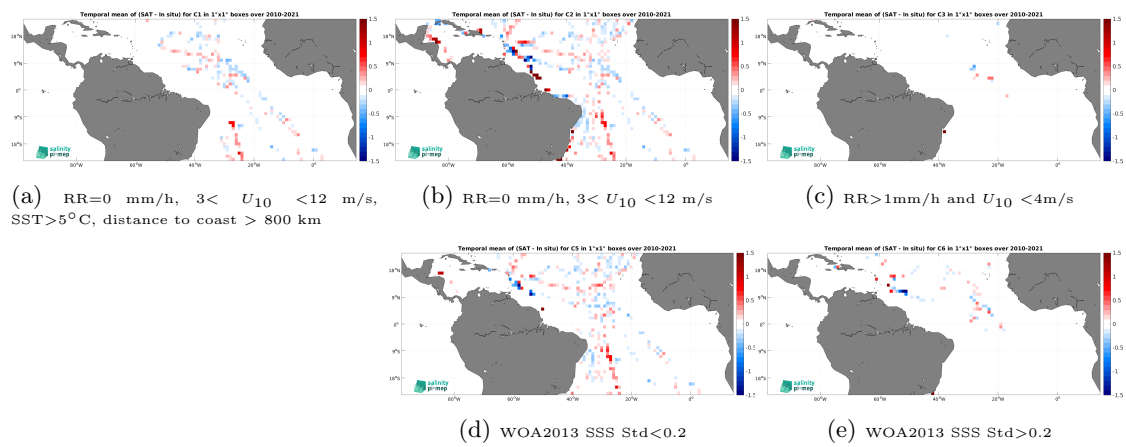
Figure 14: Temporal mean gridded over spatial boxes of size 1^\circ \times 1^\circ of \Delta SSS (SMOS SSS L3 v9 - 9 Days (CATDS-CEC-LOCEAN) - TSG (GOSUD-Sailing-ship)) for 5 different subdatasets corresponding to:RR=0 mm/h, 3 < U_{10} < 12 m/s, SST >5^\circ\text{C} , distance to coast > 800 km (a), RR=0 mm/h, 3 < U_{10} < 12 m/s (b), RR >1 mm/h and U_{10} < 4 m/s (c), WOA2013 SSS Std <0.2 (d), WOA2013 SSS Std >0.2 (e).
