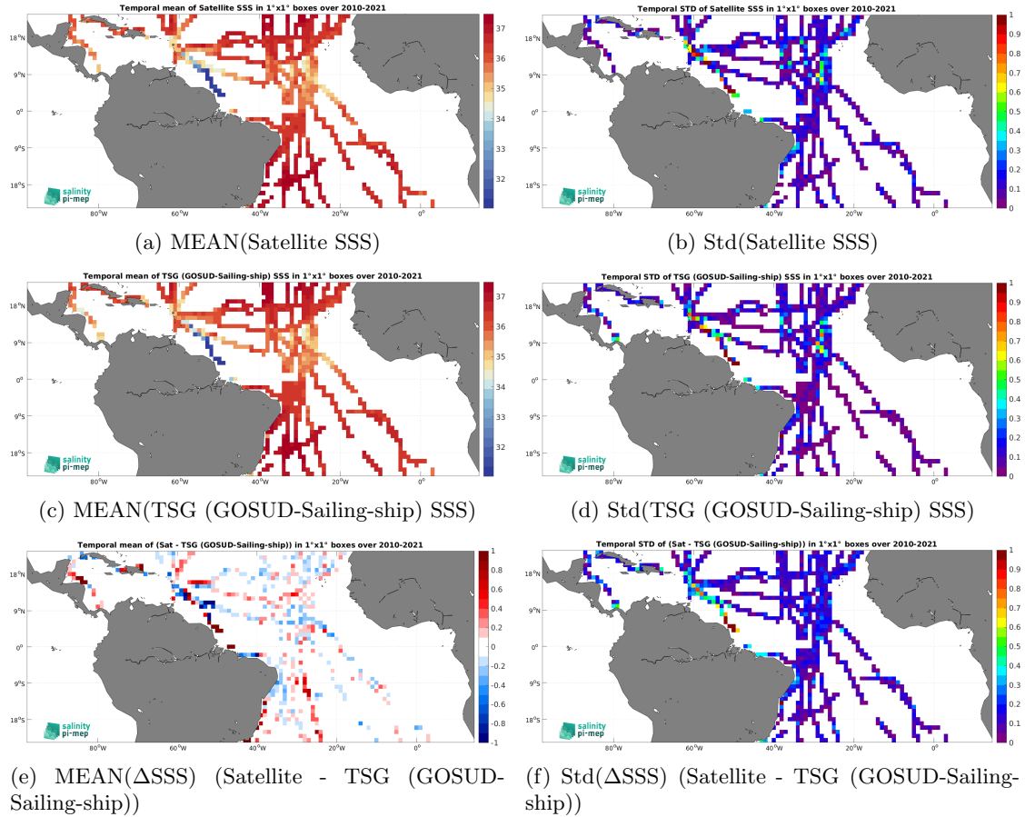
Figure 7: Temporal mean (left) and Std (right) of SSS from SMOS SSS L3 v9 - 9 Days (CATDS-CEC-LOCEAN) (top), TSG (GOSUD-Sailing-ship) (middle), and of \Delta\text{SSS} (Satellite - TSG (GOSUD-Sailing-ship)). Only match-up pairs are used to generate these maps.
