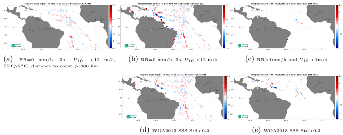
Figure 14: Temporal mean gridded over spatial boxes of size 1^\circ \times 1^\circ of \Delta\text{SSS} (SMOS SSS L3 v9 - 9 Days (CATDS-CEC-LOCEAN) - TSG (GOSUD-Sailing-ship)) for 5 different subdatasets corresponding to:RR=0 mm/h, 3 < U_{10} < 12 m/s, SST>5°C, distance to coast > 800 km (a), RR=0 mm/h, 3 < U_{10} < 12 m/s (b), RR>1mm/h and U_{10} < 4 m/s (c), WOA2013 SSS Std<0.2 (d), WOA2013 SSS Std>0.2 (e).
