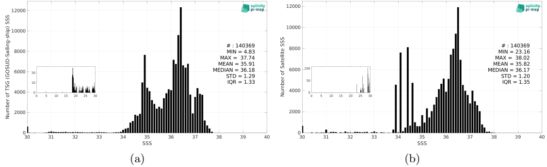
Figure 3: Histograms of SSS from TSG (GOSUD-Sailing-ship) (a) and SMOS SSS L3 v9 - 9 Days (CATDS-CEC-LOCEAN) (b) considering all match-up pairs per bins of 0.1 over the Tropical Atlantic Ocean Pi-MEP region and for the full satellite product period.
