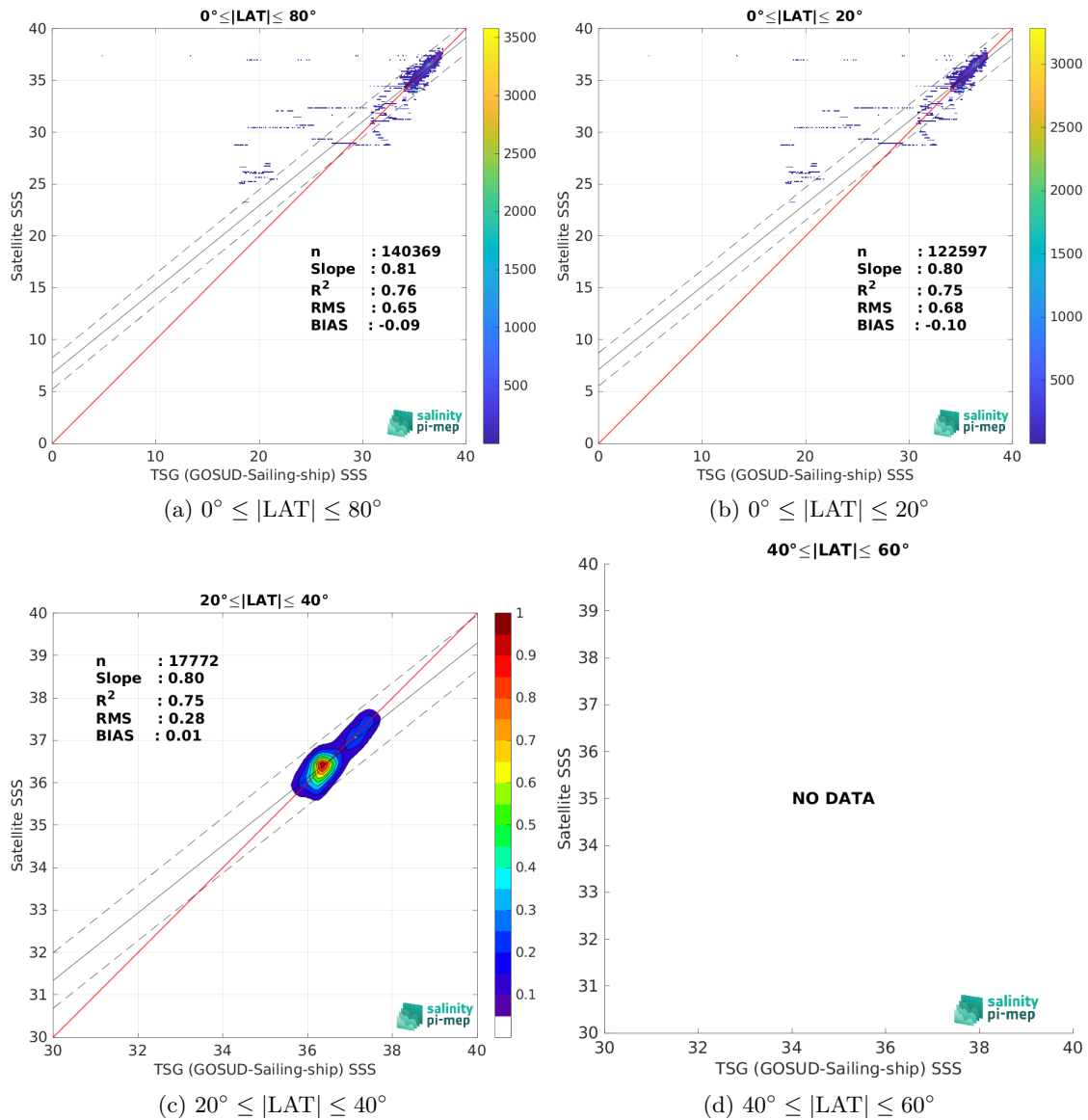
Figure 10: Contour maps of the concentration of SMOS SSS L3 v9 - 9 Days (CATDS-CEC-LOCEAN) SSS (y-axis) versus TSG (GOSUD-Sailing-ship) SSS (x-axis) at match-up pairs for different latitude bands. For each plot, the red line shows x=y . The black thin and dashed lines indicate a linear fit through the data cloud and the \pm 95\% confidence levels, respectively. The number match-up pairs n , the slope and R^2 coefficient of the linear fit, the root mean square (RMS) and the mean bias between satellite and in situ data are indicated for each latitude band in each plots.
