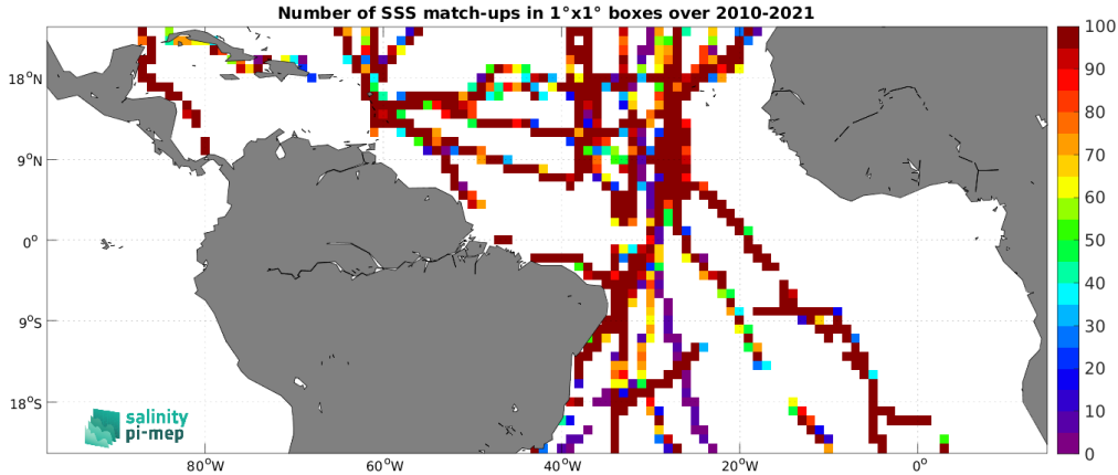
Figure 5: Number of SSS match-ups between TSG (GOSUD-Sailing-ship) SSS and the SMOS SSS L3 v9 - 9 Days (CATDS-CEC-LOCEAN) SSS product for the Tropical Atlantic Ocean Pi-MEP region over 1^\circ \times 1^\circ boxes and for the full satellite product period.
