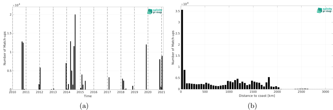
Figure 2: Number of match-ups between TSG (GOSUD-Sailing-ship) and SMOS SSS L3 v9 - 9 Days (CATDS-CEC-LOCEAN) SSS as a function of time (a) and as function of the distance to coast (b) over the Tropical Atlantic Ocean Pi-MEP region and for the full satellite product period.
