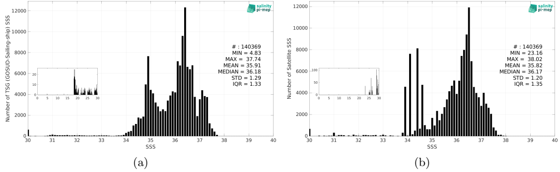
Figure 2: Histograms of SSS from TSG (GOSUD-Sailing-ship) (a) and SMOS SSS L3 v9 - 9 Days (CATDS-CEC-LOCEAN) (b) considering all match-up pairs per bins of 0.1 over the Tropical Atlantic Ocean Pi-MEP region and for the full satellite product period.
