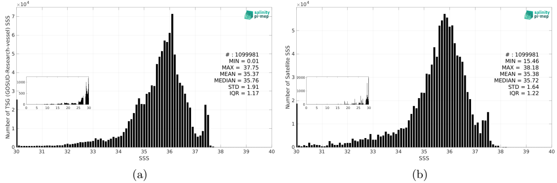
Figure 2: Histograms of SSS from TSG (GOSUD-Research-vessel) (a) and SMOS SSS L3 v9 - 9 Days (CATDS-CEC-LOCEAN) (b) considering all match-up pairs per bins of 0.1 over the Tropical Atlantic Ocean Pi-MEP region and for the full satellite product period.
