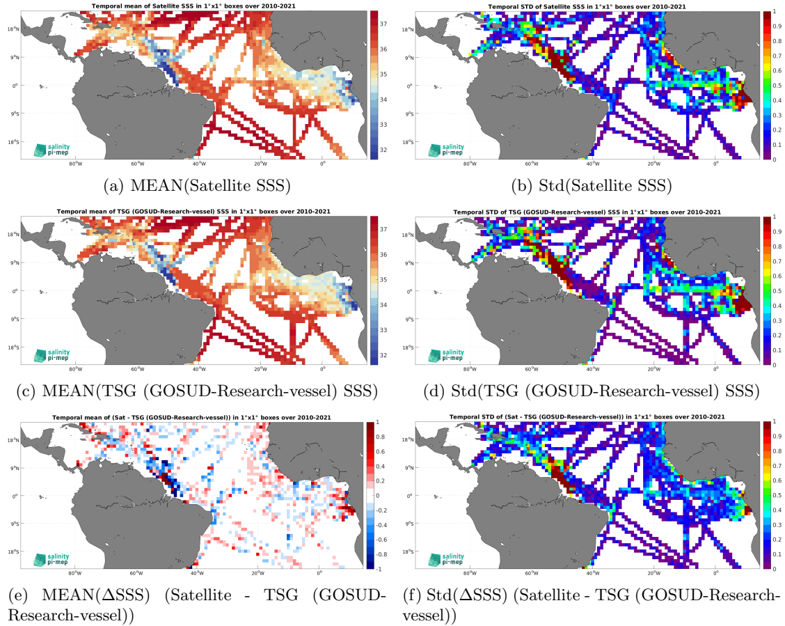
Figure 6: Temporal mean (left) and Std (right) of SSS from SMOS SSS L3 v9 - 9 Days (CATDS-CEC-LOCEAN) (top), TSG (GOSUD-Research-vessel) (middle), and of \Delta\text{SSS} (Satellite - TSG (GOSUD-Research-vessel)). Only match-up pairs are used to generate these maps.
