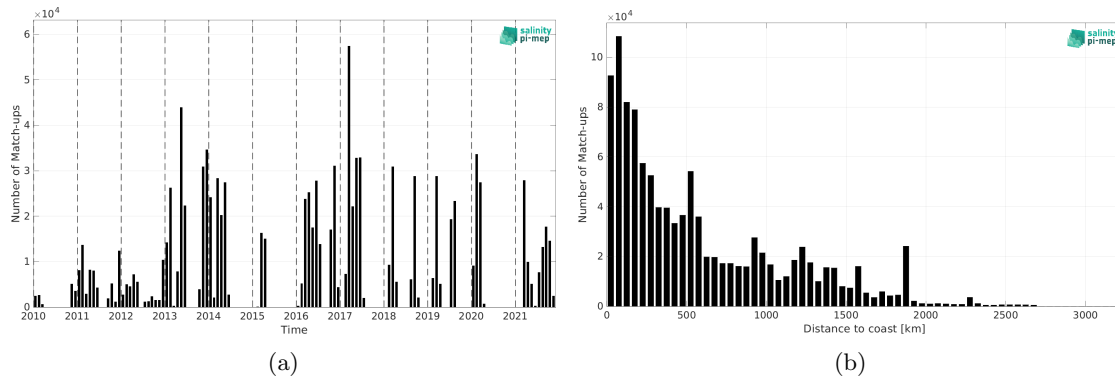
Figure 1: Number of match-ups between TSG (GOSUD-Research-vessel) and SMOS SSS L3 v9 - 9 Days (CATDS-CEC-LOCEAN) SSS as a function of time (a) and as function of the distance to coast (b) over the Tropical Atlantic Ocean Pi-MEP region and for the full satellite product period.
