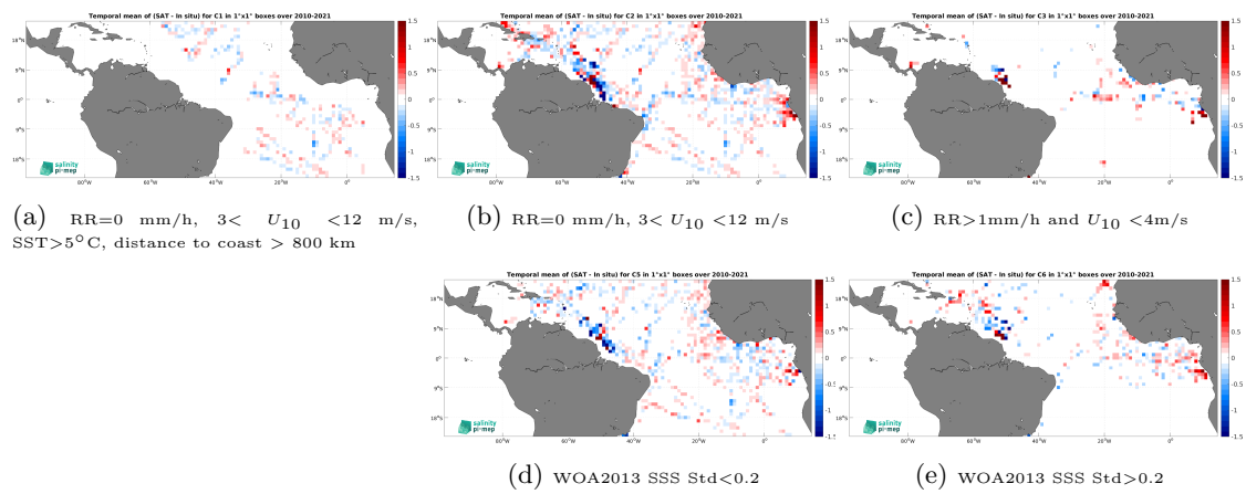
Figure 12: Temporal mean gridded over spatial boxes of size 1^\circ \times 1^\circ of \Delta\text{SSS} (SMOS SSS L3 v9 - 9 Days (CATDS-CEC-LOCEAN) - TSG (GOSUD-Research-vessel)) for 5 different subdatasets corresponding to:RR=0 mm/h, 3 < U_{10} < 12 m/s, SST>5°C, distance to coast > 800 km (a), RR=0 mm/h, 3 < U_{10} < 12 m/s (b), RR>1mm/h and U_{10} < 4 m/s (c), WOA2013 SSS Std<0.2 (d), WOA2013 SSS Std>0.2 (e).
