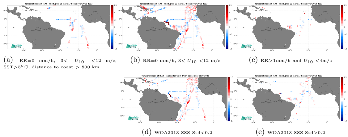
Figure 14: Temporal mean gridded over spatial boxes of size 1^\circ \times 1^\circ of \Delta\text{SSS} (SMOS SSS L3 v9 - 9 Days (CATDS-CEC-LOCEAN) - TSG (CSIC-UTM)) for 5 different subdatasets corresponding to:RR=0 mm/h, 3 < U_{10} < 12 m/s, SST>5°C, distance to coast > 800 km (a), RR=0 mm/h, 3 < U_{10} < 12 m/s (b), RR>1mm/h and U_{10} < 4 m/s (c), WOA2013 SSS Std<0.2 (d), WOA2013 SSS Std>0.2 (e).
