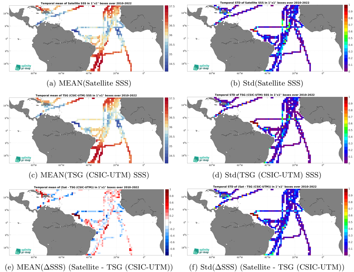
Figure 6: Temporal mean (left) and Std (right) of SSS from SMOS SSS L3 v9 - 9 Days (CATDS-CEC-LOCEAN) (top), TSG (CSIC-UTM) (middle), and of \Delta\text{SSS} (Satellite - TSG (CSIC-UTM)). Only match-up pairs are used to generate these maps.
