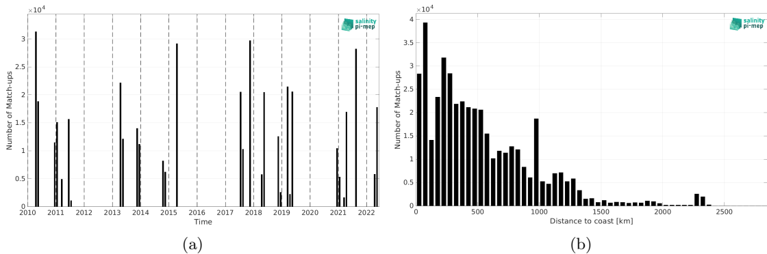
Figure 1: Number of match-ups between TSG (CSIC-UTM) and SMOS SSS L3 v9 - 9 Days (CATDS-CEC-LOCEAN) SSS as a function of time (a) and as function of the distance to coast (b) over the Tropical Atlantic Ocean Pi-MEP region and for the full satellite product period.
