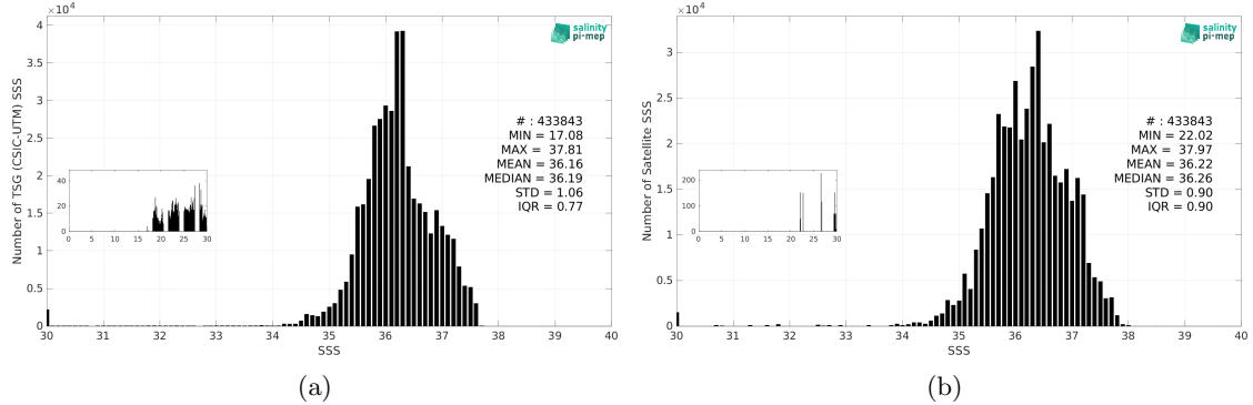
Figure 2: Histograms of SSS from TSG (CSIC-UTM) (a) and SMOS SSS L3 v9 - 9 Days (CATDS-CEC-LOCEAN) (b) considering all match-up pairs per bins of 0.1 over the Tropical Atlantic Ocean Pi-MEP region and for the full satellite product period.
