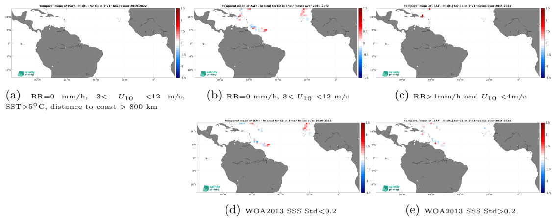
Figure 14: Temporal mean gridded over spatial boxes of size 1^\circ \times 1^\circ of \Delta\text{SSS} (SMOS SSS L3 v9 - 9 Days (CATDS-CEC-LOCEAN) - Saildrone) for 5 different subdatasets corresponding to:RR=0 mm/h, 3 < U_{10} < 12 m/s, SST >5^\circ\text{C} , distance to coast > 800 km (a), RR=0 mm/h, 3 < U_{10} < 12 m/s (b), RR >1 mm/h and U_{10} < 4 m/s (c), WOA2013 SSS Std <0.2 (d), WOA2013 SSS Std >0.2 (e).
