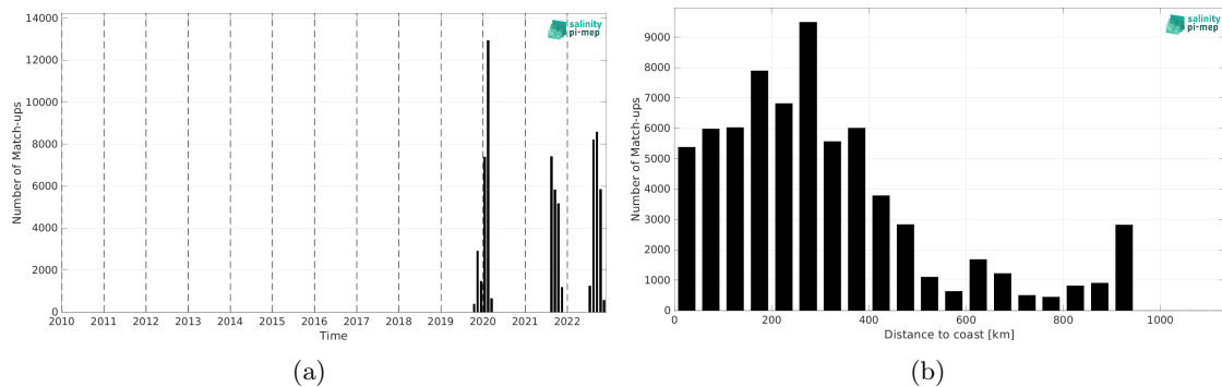
Figure 1: Number of match-ups between Saildrone and SMOS SSS L3 v9 - 9 Days (CATDS-CEC-LOCEAN) SSS as a function of time (a) and as function of the distance to coast (b) over the Tropical Atlantic Ocean Pi-MEP region and for the full satellite product period.
