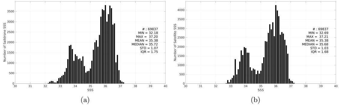
Figure 2: Histograms of SSS from Saildrone (a) and SMOS SSS L3 v9 - 9 Days (CATDS-CEC-LOCEAN) (b) considering all match-up pairs per bins of 0.1 over the Tropical Atlantic Ocean Pi-MEP region and for the full satellite product period.
