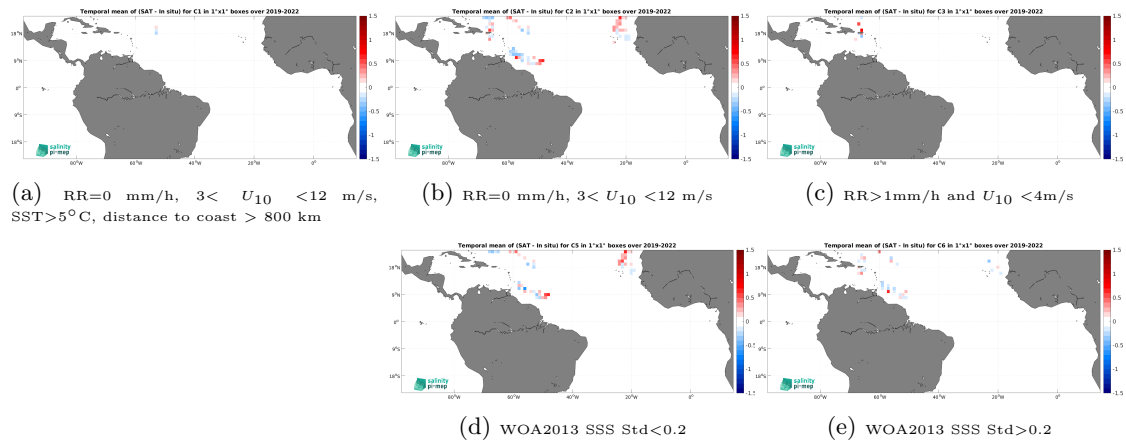
Figure 12: Temporal mean gridded over spatial boxes of size 1^\circ \times 1^\circ of \Delta\text{SSS} (SMOS SSS L3 v9 - 9 Days (CATDS-CEC-LOCEAN) - Saildrone) for 5 different subdatasets corresponding to:RR=0 mm/h, 3 < U_{10} < 12 m/s, SST >5^\circ\text{C} , distance to coast > 800 km (a), RR=0 mm/h, 3 < U_{10} < 12 m/s (b), RR >1 mm/h and U_{10} < 4 m/s (c), WOA2013 SSS Std <0.2 (d), WOA2013 SSS Std >0.2 (e).
