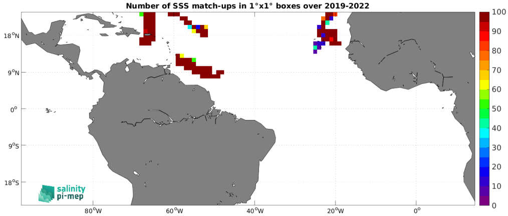
Figure 4: Number of SSS match-ups between Saildrone SSS and the SMOS SSS L3 v9 - 9 Days (CATDS-CEC-LOCEAN) SSS product for the Tropical Atlantic Ocean Pi-MEP region over 1^\circ \times 1^\circ boxes and for the full satellite product period.
