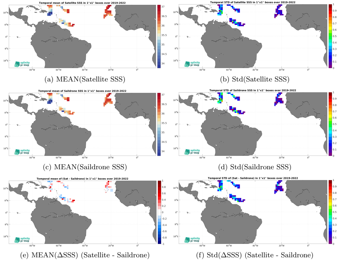
Figure 6: Temporal mean (left) and Std (right) of SSS from SMOS SSS L3 v9 - 9 Days (CATDS-CEC-LOCEAN) (top), Saildrone (middle), and of \Delta\text{SSS} (Satellite - Saildrone). Only match-up pairs are used to generate these maps.
