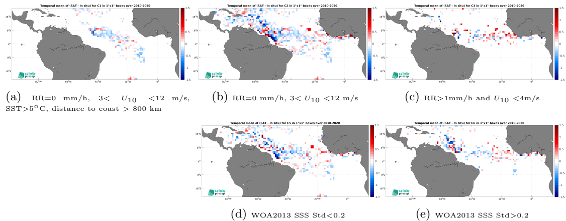
Figure 13: Temporal mean gridded over spatial boxes of size 1^\circ \times 1^\circ of \Delta SSS (SMOS SSS L3 v9 - 9 Days (CATDS-CEC-LOCEAN) - Surface drifters) for 5 different subdatasets corresponding to:RR=0 mm/h, 3 < U_{10} < 12 m/s, SST >5^\circ\text{C} , distance to coast > 800 km (a), RR=0 mm/h, 3 < U_{10} < 12 m/s (b), RR >1 mm/h and U_{10} < 4 m/s (c), WOA2013 SSS Std <0.2 (d), WOA2013 SSS Std >0.2 (e).
