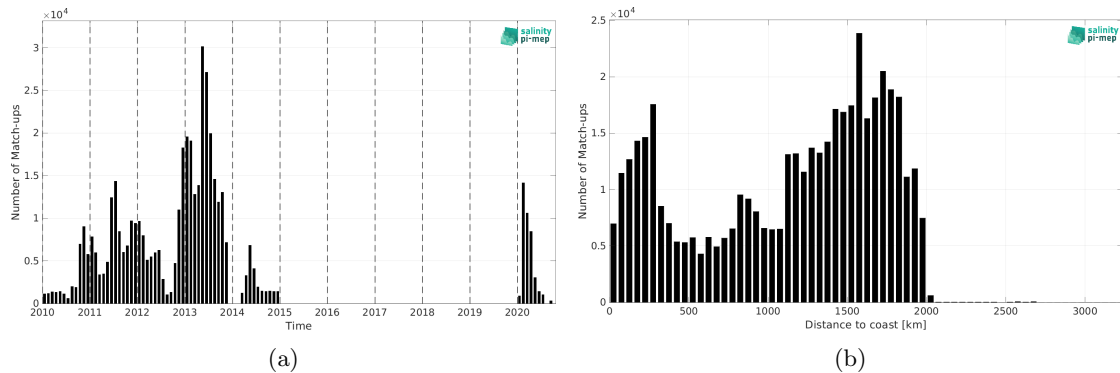
Figure 2: Number of match-ups between Surface drifters and SMOS SSS L3 v9 - 9 Days (CATDS-CEC-LOCEAN) SSS as a function of time (a) and as function of the distance to coast (b) over the Tropical Atlantic Ocean Pi-MEP region and for the full satellite product period.
