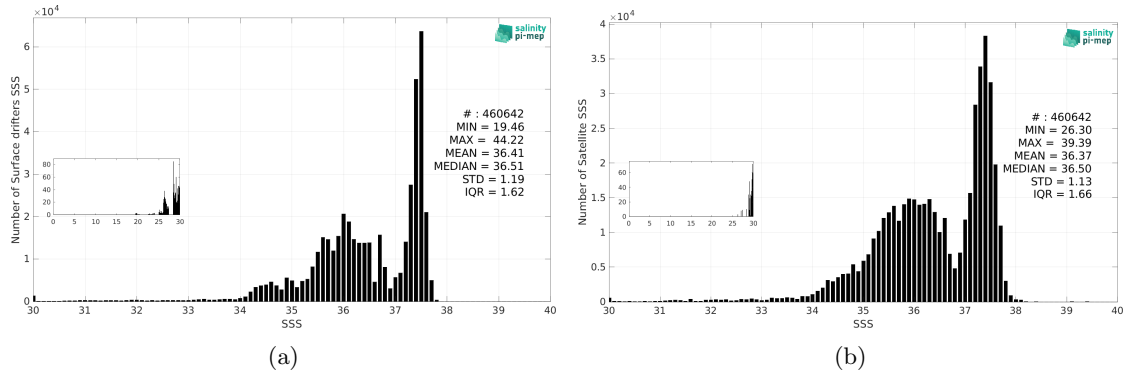
Figure 3: Histograms of SSS from Surface drifters (a) and SMOS SSS L3 v9 - 9 Days (CATDS-CEC-LOCEAN) (b) considering all match-up pairs per bins of 0.1 over the Tropical Atlantic Ocean Pi-MEP region and for the full satellite product period.
