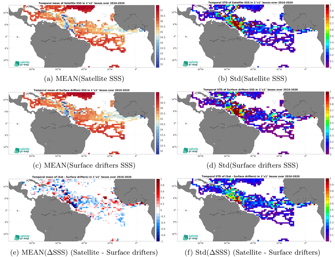
Figure 6: Temporal mean (left) and Std (right) of SSS from SMOS SSS L3 v9 - 9 Days (CATDS-CEC-LOCEAN) (top), Surface drifters (middle), and of \Delta SSS (Satellite - Surface drifters). Only match-up pairs are used to generate these maps.
