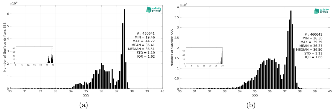
Figure 2: Histograms of SSS from Surface drifters (a) and SMOS SSS L3 v9 - 9 Days (CATDS-CEC-LOCEAN) (b) considering all match-up pairs per bins of 0.1 over the Tropical Atlantic Ocean Pi-MEP region and for the full satellite product period.
