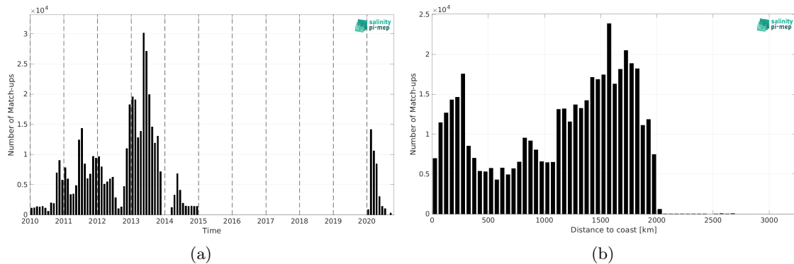
Figure 1: Number of match-ups between Surface drifters and SMOS SSS L3 v9 - 9 Days (CATDS-CEC-LOCEAN) SSS as a function of time (a) and as function of the distance to coast (b) over the Tropical Atlantic Ocean Pi-MEP region and for the full satellite product period.
