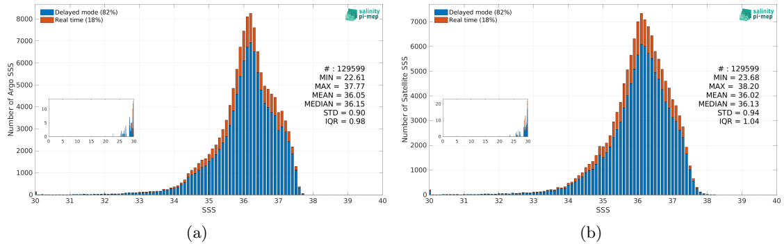
Figure 2: Histograms of SSS from Argo (a) and SMOS SSS L3 v9 - 9 Days (CATDS-CEC-LOCEAN) (b) considering all match-up pairs per bins of 0.1 over the Tropical Atlantic Ocean Pi-MEP region and for the full satellite product period.
