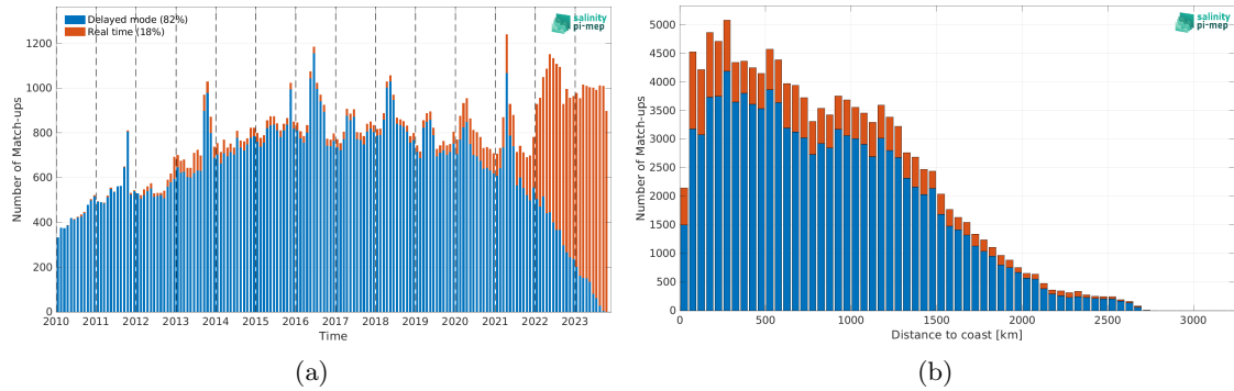
Figure 1: Number of match-ups between Argo and SMOS SSS L3 v9 - 9 Days (CATDS-CEC-LOCEAN) SSS as a function of time (a) and as function of the distance to coast (b) over the Tropical Atlantic Ocean Pi-MEP region and for the full satellite product period.
