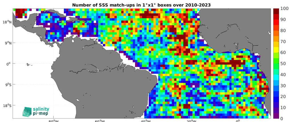
Figure 4: Number of SSS match-ups between Argo SSS and the SMOS SSS L3 v9 - 9 Days (CATDS-CEC-LOCEAN) SSS product for the Tropical Atlantic Ocean Pi-MEP region over 1^\circ \times 1^\circ boxes and for the full satellite product period.
