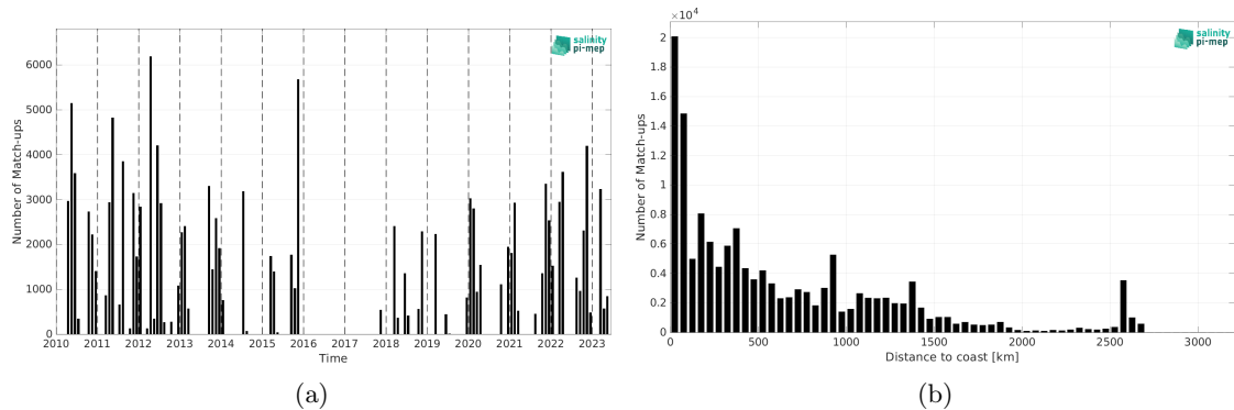
Figure 2: Number of match-ups between TSG (SAMOS) and SMOS SSS L3 v9 - 18 Days (CATDS-CEC-LOCEAN) SSS as a function of time (a) and as function of the distance to coast (b) over the Tropical Atlantic Ocean Pi-MEP region and for the full satellite product period.
