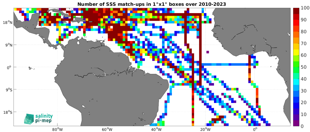
Figure 5: Number of SSS match-ups between TSG (SAMOS) SSS and the SMOS SSS L3 v9 - 18 Days (CATDS-CEC-LOCEAN) SSS product for the Tropical Atlantic Ocean Pi-MEP region over 1^\circ \times 1^\circ boxes and for the full satellite product period.
