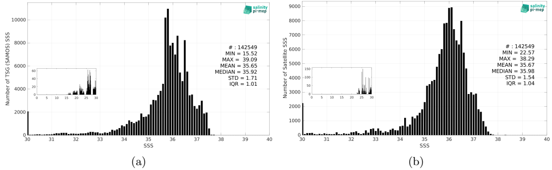
Figure 3: Histograms of SSS from TSG (SAMOS) (a) and SMOS SSS L3 v9 - 18 Days (CATDS-CEC-LOCEAN) (b) considering all match-up pairs per bins of 0.1 over the Tropical Atlantic Ocean Pi-MEP region and for the full satellite product period.
