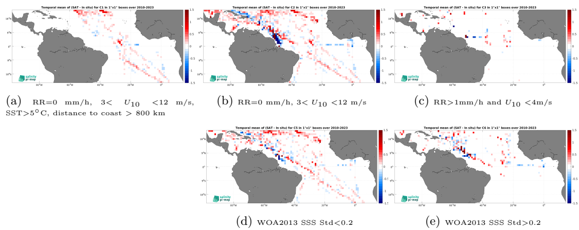
Figure 14: Temporal mean gridded over spatial boxes of size 1^\circ \times 1^\circ of \Delta\text{SSS} (SMOS SSS L3 v9 - 18 Days (CATDS-CEC-LOCEAN) - TSG (SAMOS)) for 5 different subdatasets corresponding to:RR=0 mm/h, 3 < U_{10} < 12 m/s, SST>5°C, distance to coast > 800 km (a), RR=0 mm/h, 3 < U_{10} < 12 m/s (b), RR>1mm/h and U_{10} < 4 m/s (c), WOA2013 SSS Std<0.2 (d), WOA2013 SSS Std>0.2 (e).
