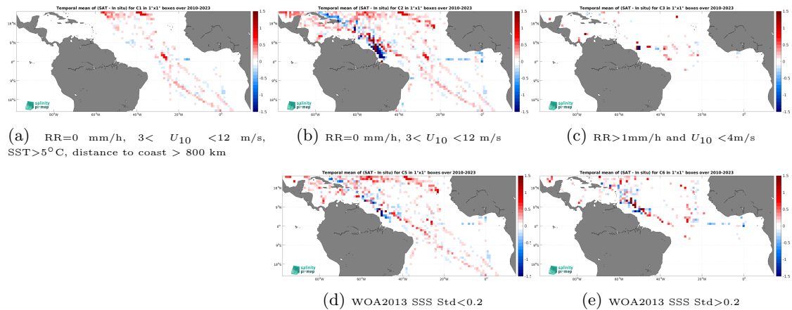
Figure 12: Temporal mean gridded over spatial boxes of size 1^\circ \times 1^\circ of \Delta SSS (SMOS SSS L3 v9 - 18 Days (CATDS-CEC-LOCEAN) - TSG (SAMOS)) for 5 different subdatasets corresponding to:RR=0 mm/h, 3 < U_{10} < 12 m/s, SST >5^\circ C, distance to coast > 800 km (a), RR=0 mm/h, 3 < U_{10} < 12 m/s (b), RR >1 mm/h and U_{10} < 4 m/s (c), WOA2013 SSS Std <0.2 (d), WOA2013 SSS Std >0.2 (e).
