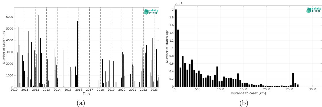
Figure 1: Number of match-ups between TSG (SAMOS) and SMOS SSS L3 v9 - 18 Days (CATDS-CEC-LOCEAN) SSS as a function of time (a) and as function of the distance to coast (b) over the Tropical Atlantic Ocean Pi-MEP region and for the full satellite product period.
