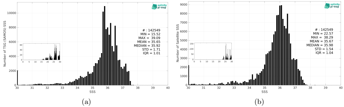
Figure 2: Histograms of SSS from TSG (SAMOS) (a) and SMOS SSS L3 v9 - 18 Days (CATDS-CEC-LOCEAN) (b) considering all match-up pairs per bins of 0.1 over the Tropical Atlantic Ocean Pi-MEP region and for the full satellite product period.
