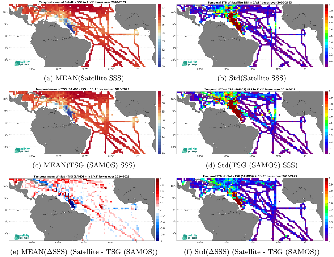
Figure 6: Temporal mean (left) and Std (right) of SSS from SMOS SSS L3 v9 - 18 Days (CATDS-CEC-LOCEAN) (top), TSG (SAMOS) (middle), and of \Delta\text{SSS} (Satellite - TSG (SAMOS)). Only match-up pairs are used to generate these maps.
