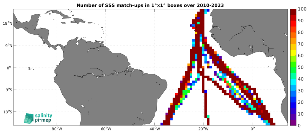
Figure 5: Number of SSS match-ups between TSG (Polarstern) SSS and the SMOS SSS L3 v9 - 18 Days (CATDS-CEC-LOCEAN) SSS product for the Tropical Atlantic Ocean Pi-MEP region over 1^\circ \times 1^\circ boxes and for the full satellite product period.
