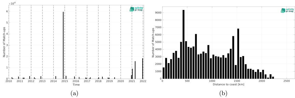
Figure 1: Number of match-ups between TSG (Polarstern) and SMOS SSS L3 v9 - 18 Days (CATDS-CEC-LOCEAN) SSS as a function of time (a) and as function of the distance to coast (b) over the Tropical Atlantic Ocean Pi-MEP region and for the full satellite product period.
