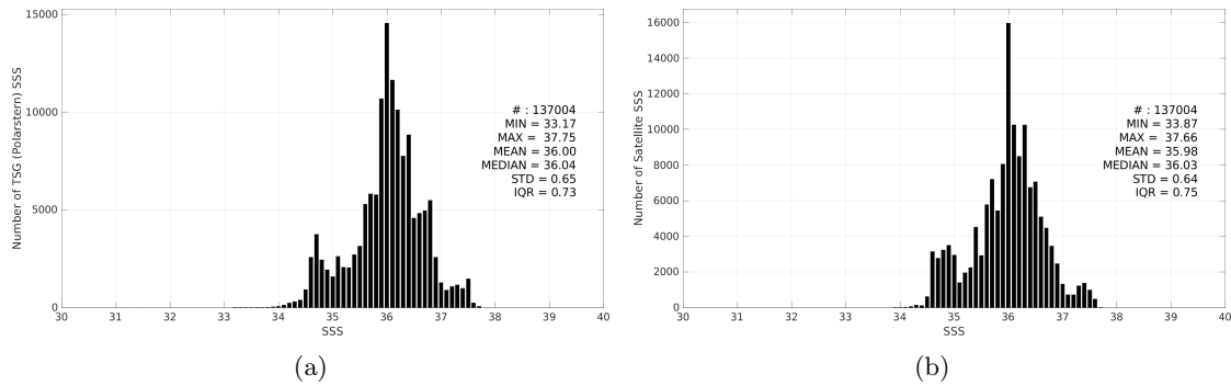
Figure 2: Histograms of SSS from TSG (Polarstern) (a) and SMOS SSS L3 v9 - 18 Days (CATDS-CEC-LOCEAN) (b) considering all match-up pairs per bins of 0.1 over the Tropical Atlantic Ocean Pi-MEP region and for the full satellite product period.
