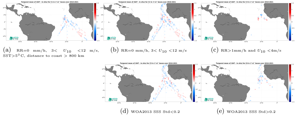
Figure 12: Temporal mean gridded over spatial boxes of size 1^{\circ}\times 1^{\circ} of \Delta\text{SSS} (SMOS SSS L3 v9 - 18 Days (CATDS-CEC-LOCEAN) - TSG (Polarstern)) for 5 different subdatasets corresponding to: RR=0 mm/h, 3 < U_{10} < 12 m/s, SST > 5^{\circ}\text{C} , distance to coast > 800 km (a), RR=0 mm/h, 3 < U_{10} < 12 m/s (b), RR > 1 mm/h and U_{10} < 4 m/s (c), WOA2013 SSS Std < 0.2 (d), WOA2013 SSS Std > 0.2 (e).
