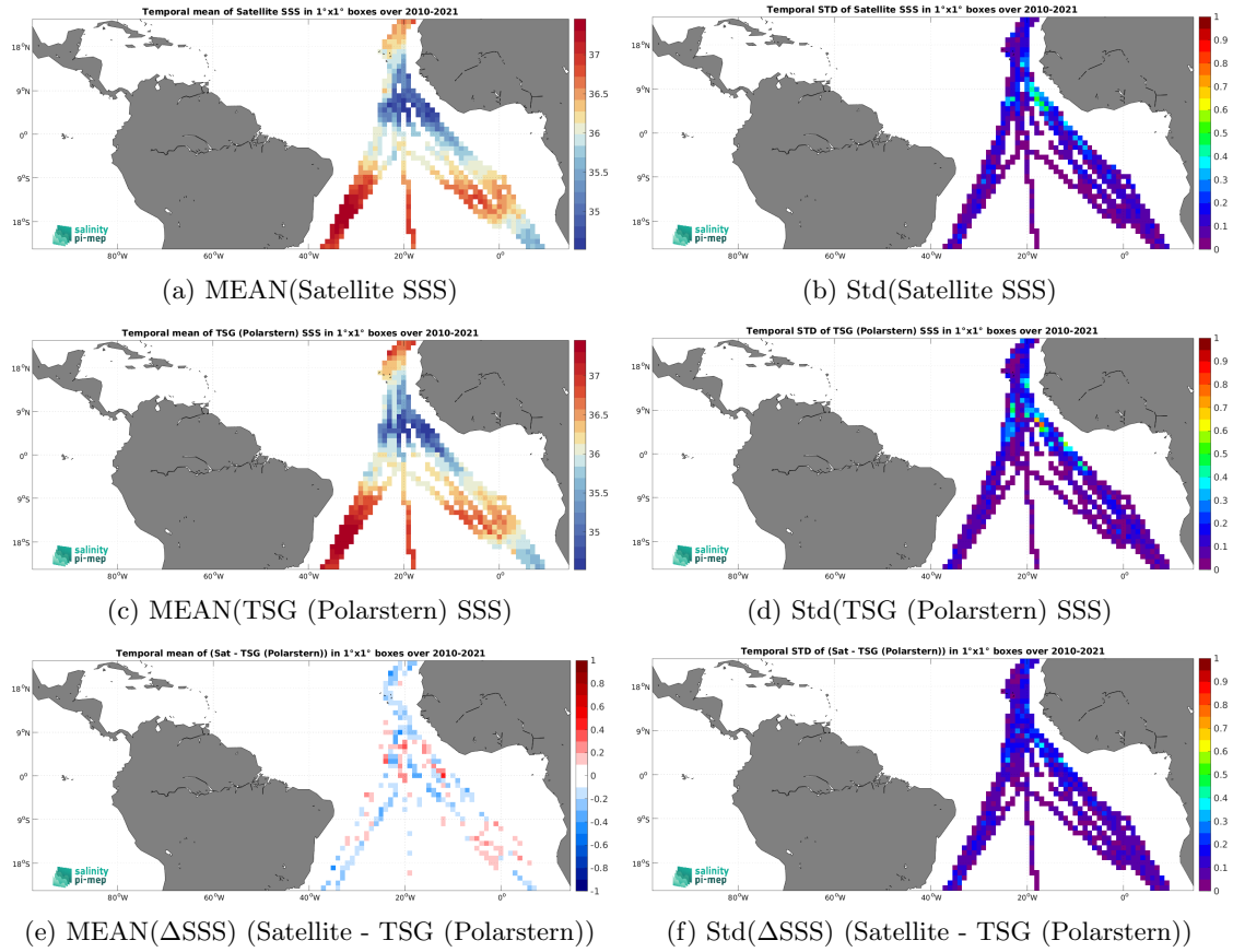
Figure 6: Temporal mean (left) and Std (right) of SSS from SMOS SSS L3 v9 - 18 Days (CATDS-CEC-LOCEAN) (top), TSG (Polarstern) (middle), and of \Delta SSS (Satellite - TSG (Polarstern)). Only match-up pairs are used to generate these maps.
