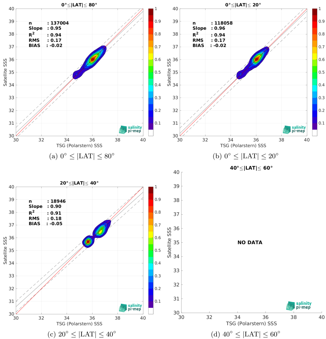
Figure 9: Contour maps of the concentration of SMOS SSS L3 v9 - 18 Days (CATDS-CEC-LOCEAN) SSS (y-axis) versus TSG (Polarstern) SSS (x-axis) at match-up pairs for different latitude bands. For each plot, the red line shows x=y . The black thin and dashed lines indicate a linear fit through the data cloud and the \pm 95\% confidence levels, respectively. The number match-up pairs n , the slope and R^2 coefficient of the linear fit, the root mean square (RMS) and the mean bias between satellite and in situ data are indicated for each latitude band in each plots.
