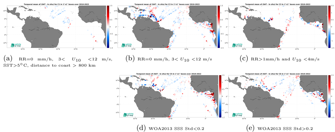
Figure 14: Temporal mean gridded over spatial boxes of size 1^\circ \times 1^\circ of \Delta\text{SSS} (SMOS SSS L3 v9 - 18 Days (CATDS-CEC-LOCEAN) - TSG (LEGOS-DM)) for 5 different subdatasets corresponding to:RR=0 mm/h, 3 < U_{10} < 12 m/s, SST>5°C, distance to coast > 800 km (a), RR=0 mm/h, 3 < U_{10} < 12 m/s (b), RR>1mm/h and U_{10} < 4 m/s (c), WOA2013 SSS Std<0.2 (d), WOA2013 SSS Std>0.2 (e).
