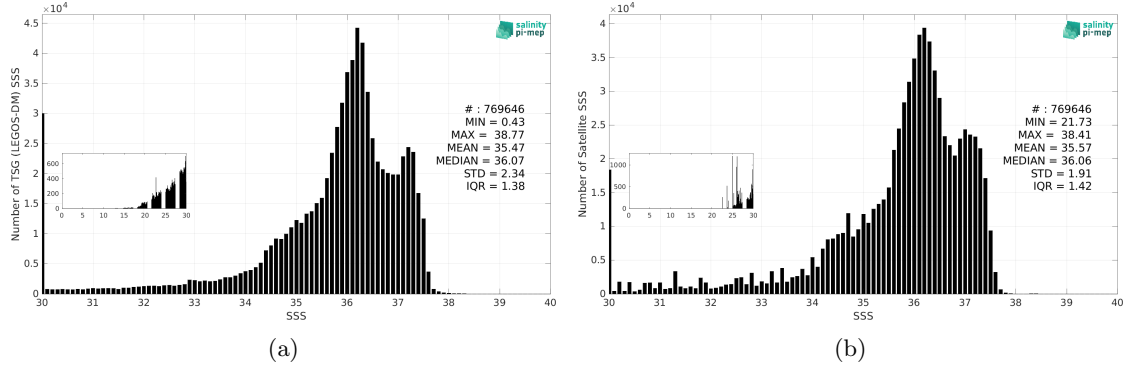
Figure 3: Histograms of SSS from TSG (LEGOS-DM) (a) and SMOS SSS L3 v9 - 18 Days (CATDS-CEC-LOCEAN) (b) considering all match-up pairs per bins of 0.1 over the Tropical Atlantic Ocean Pi-MEP region and for the full satellite product period.
