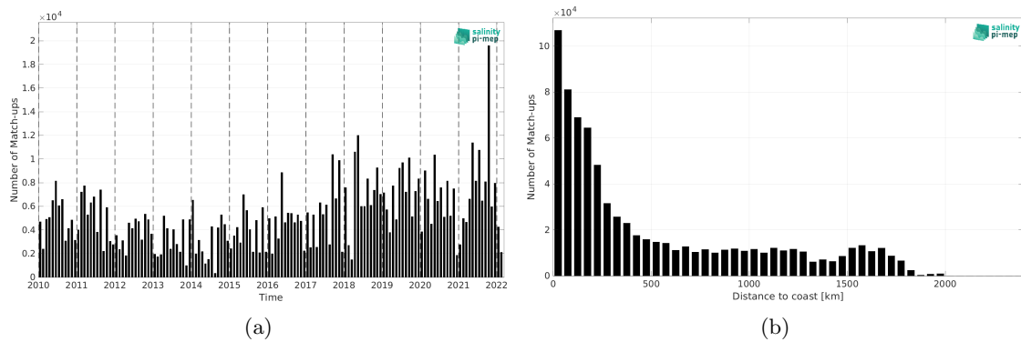
Figure 1: Number of match-ups between TSG (LEGOS-DM) and SMOS SSS L3 v9 - 18 Days (CATDS-CEC-LOCEAN) SSS as a function of time (a) and as function of the distance to coast (b) over the Tropical Atlantic Ocean Pi-MEP region and for the full satellite product period.
