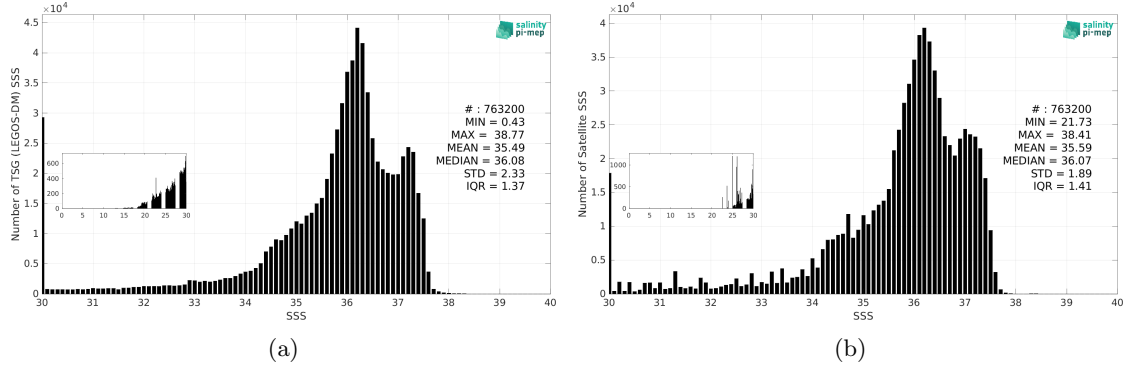
Figure 2: Histograms of SSS from TSG (LEGOS-DM) (a) and SMOS SSS L3 v9 - 18 Days (CATDS-CEC-LOCEAN) (b) considering all match-up pairs per bins of 0.1 over the Tropical Atlantic Ocean Pi-MEP region and for the full satellite product period.
