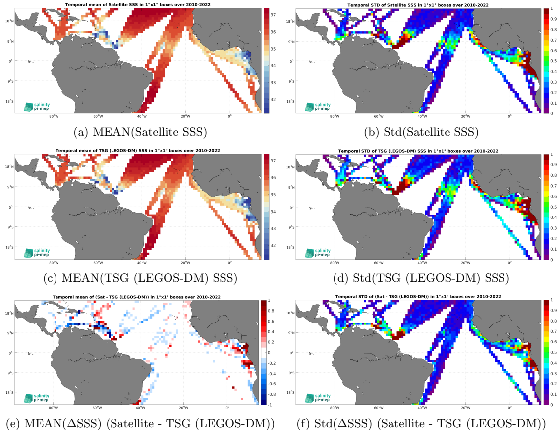
Figure 6: Temporal mean (left) and Std (right) of SSS from SMOS SSS L3 v9 - 18 Days (CATDS-CEC-LOCEAN) (top), TSG (LEGOS-DM) (middle), and of \Delta\text{SSS} (Satellite - TSG (LEGOS-DM)). Only match-up pairs are used to generate these maps.
