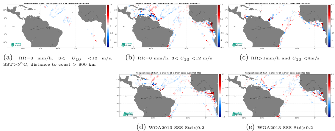
Figure 12: Temporal mean gridded over spatial boxes of size 1^\circ \times 1^\circ of \Delta\text{SSS} (SMOS SSS L3 v9 - 18 Days (CATDS-CEC-LOCEAN) - TSG (LEGOS-DM)) for 5 different subdatasets corresponding to:RR=0 mm/h, 3 < U_{10} < 12 m/s, SST >5^\circ\text{C} , distance to coast > 800 km (a), RR=0 mm/h, 3 < U_{10} < 12 m/s (b), RR >1 mm/h and U_{10} < 4 m/s (c), WOA2013 SSS Std <0.2 (d), WOA2013 SSS Std >0.2 (e).
