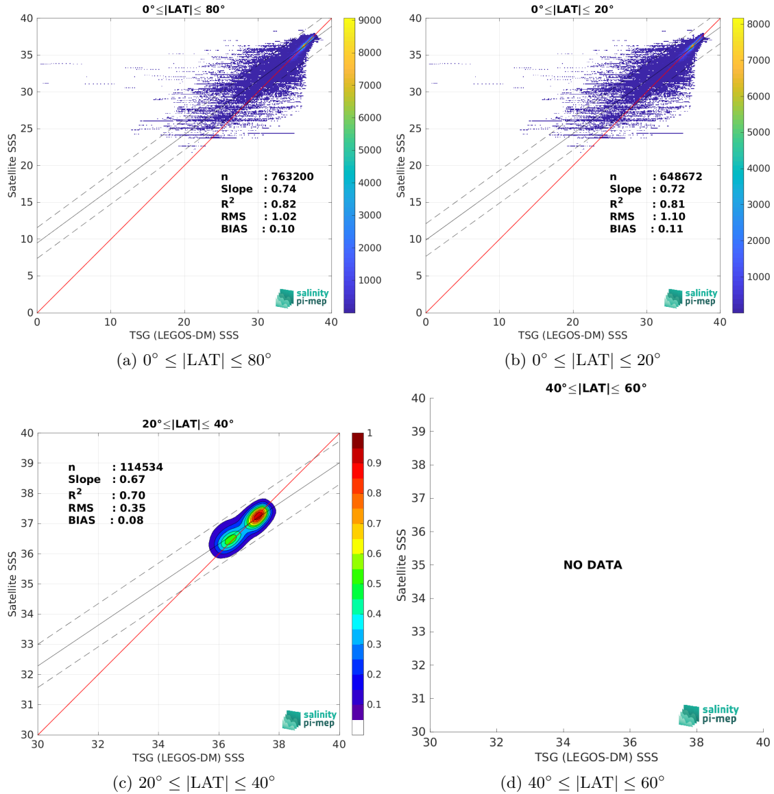
Figure 9: Contour maps of the concentration of SMOS SSS L3 v9 - 18 Days (CATDS-CEC-LOCEAN) SSS (y-axis) versus TSG (LEGOS-DM) SSS (x-axis) at match-up pairs for different latitude bands. For each plot, the red line shows x=y . The black thin and dashed lines indicate a linear fit through the data cloud and the \pm 95\% confidence levels, respectively. The number of match-up pairs n , the slope and R^2 coefficient of the linear fit, the root mean square (RMS) and the mean bias between satellite and in situ data are indicated for each latitude band in each plot.
