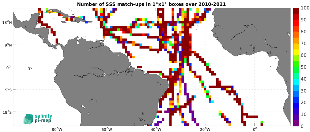
Figure 5: Number of SSS match-ups between TSG (GOSUD-Sailing-ship) SSS and the SMOS SSS L3 v9 - 18 Days (CATDS-CEC-LOCEAN) SSS product for the Tropical Atlantic Ocean Pi-MEP region over 1^\circ \times 1^\circ boxes and for the full satellite product period.
