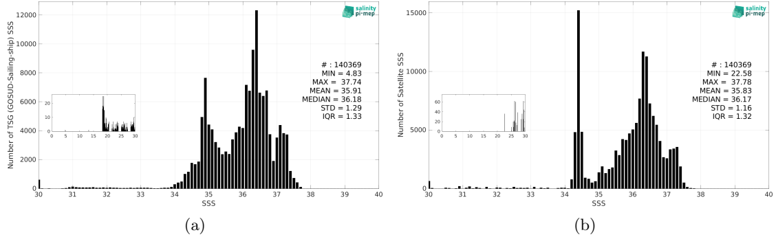
Figure 3: Histograms of SSS from TSG (GOSUD-Sailing-ship) (a) and SMOS SSS L3 v9 - 18 Days (CATDS-CEC-LOCEAN) (b) considering all match-up pairs per bins of 0.1 over the Tropical Atlantic Ocean Pi-MEP region and for the full satellite product period.
