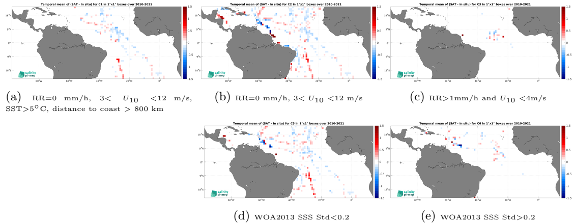
Figure 12: Temporal mean gridded over spatial boxes of size 1^{\circ}\times 1^{\circ} of \Delta SSS (SMOS SSS L3 v9 - 18 Days (CATDS-CEC-LOCEAN) - TSG (GOSUD-Sailing-ship)) for 5 different subdatasets corresponding to:RR=0 mm/h, 3 < U_{10} < 12 m/s, SST >5^{\circ}\text{C} , distance to coast > 800 km (a), RR=0 mm/h, 3 < U_{10} < 12 m/s (b), RR >1 mm/h and U_{10} < 4 m/s (c), WOA2013 SSS Std <0.2 (d), WOA2013 SSS Std >0.2 (e).
