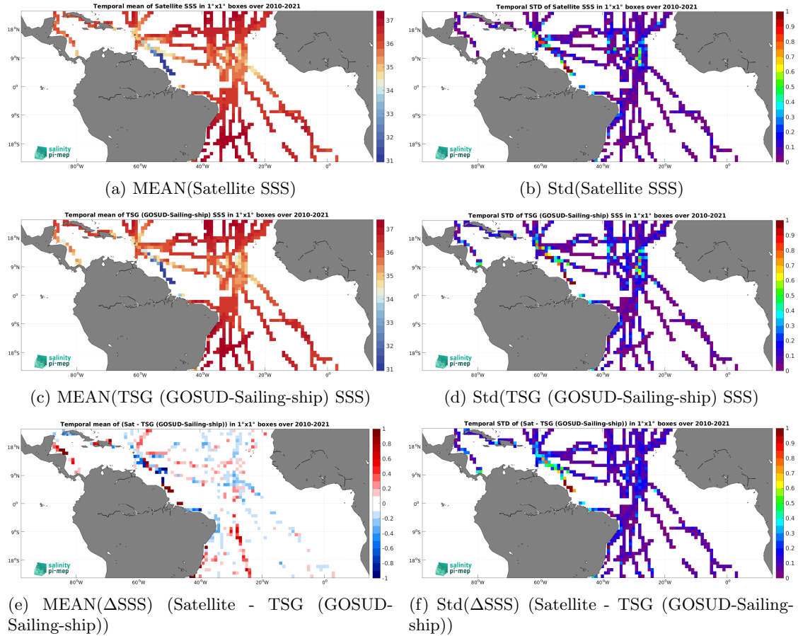
Figure 6: Temporal mean (left) and Std (right) of SSS from SMOS SSS L3 v9 - 18 Days (CATDS-CEC-LOCEAN) (top), TSG (GOSUD-Sailing-ship) (middle), and of \Delta\text{SSS} (Satellite - TSG (GOSUD-Sailing-ship)). Only match-up pairs are used to generate these maps.
