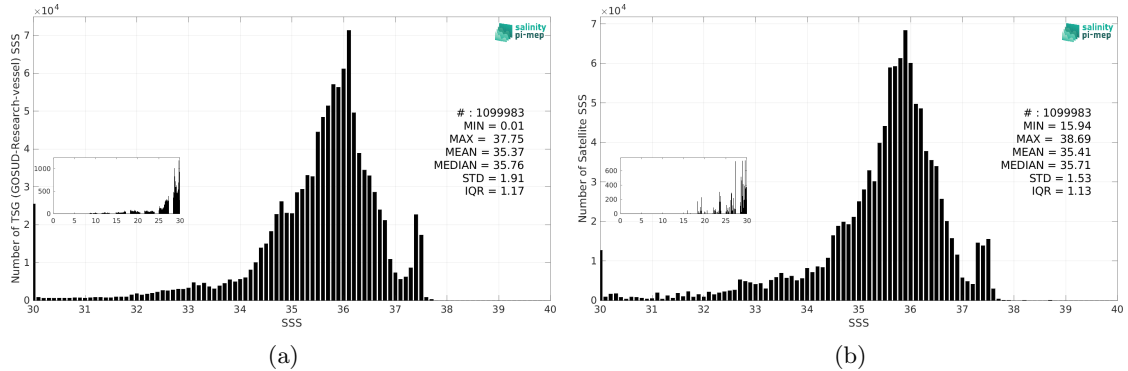
Figure 3: Histograms of SSS from TSG (GOSUD-Research-vessel) (a) and SMOS SSS L3 v9 - 18 Days (CATDS-CEC-LOCEAN) (b) considering all match-up pairs per bins of 0.1 over the Tropical Atlantic Ocean Pi-MEP region and for the full satellite product period.
