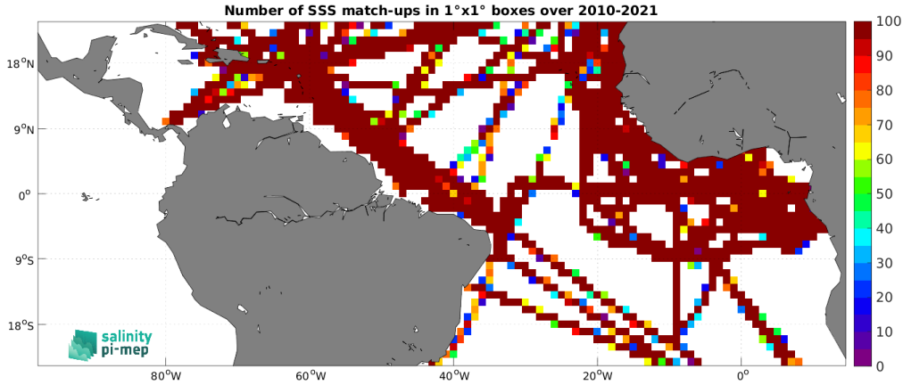
Figure 5: Number of SSS match-ups between TSG (GOSUD-Research-vessel) SSS and the SMOS SSS L3 v9 - 18 Days (CATDS-CEC-LOCEAN) SSS product for the Tropical Atlantic Ocean Pi-MEP region over 1^\circ \times 1^\circ boxes and for the full satellite product period.
