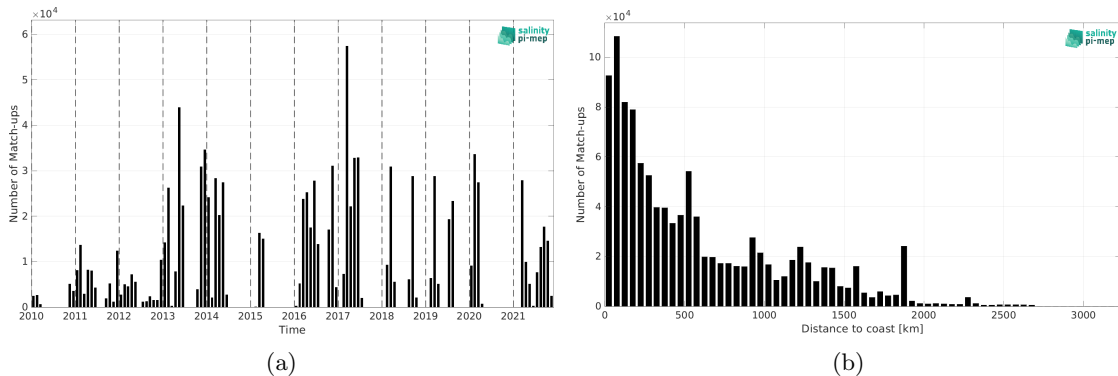
Figure 2: Number of match-ups between TSG (GOSUD-Research-vessel) and SMOS SSS L3 v9 - 18 Days (CATDS-CEC-LOCEAN) SSS as a function of time (a) and as function of the distance to coast (b) over the Tropical Atlantic Ocean Pi-MEP region and for the full satellite product period.
