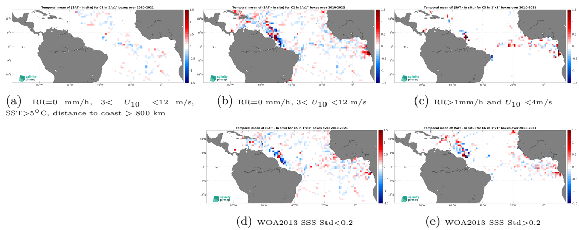
Figure 14: Temporal mean gridded over spatial boxes of size 1^\circ \times 1^\circ of \Delta\text{SSS} (SMOS SSS L3 v9 - 18 Days (CATDS-CEC-LOCEAN) - TSG (GOSUD-Research-vessel)) for 5 different subdatasets corresponding to:RR=0 mm/h, 3 < U_{10} < 12 m/s, SST>5°C, distance to coast > 800 km (a), RR=0 mm/h, 3 < U_{10} < 12 m/s (b), RR>1mm/h and U_{10} < 4 m/s (c), WOA2013 SSS Std<0.2 (d), WOA2013 SSS Std>0.2 (e).
