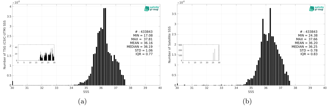
Figure 3: Histograms of SSS from TSG (CSIC-UTM) (a) and SMOS SSS L3 v9 - 18 Days (CATDS-CEC-LOCEAN) (b) considering all match-up pairs per bins of 0.1 over the Tropical Atlantic Ocean Pi-MEP region and for the full satellite product period.
