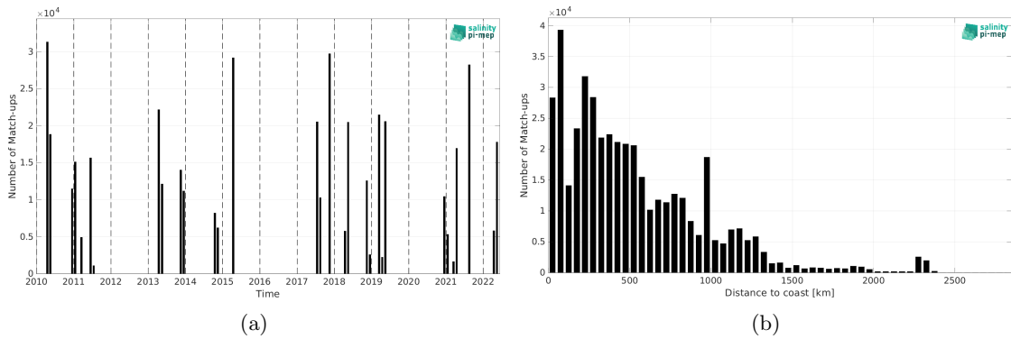
Figure 2: Number of match-ups between TSG (CSIC-UTM) and SMOS SSS L3 v9 - 18 Days (CATDS-CEC-LOCEAN) SSS as a function of time (a) and as function of the distance to coast (b) over the Tropical Atlantic Ocean Pi-MEP region and for the full satellite product period.
