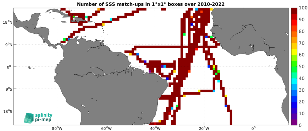
Figure 5: Number of SSS match-ups between TSG (CSIC-UTM) SSS and the SMOS SSS L3 v9 - 18 Days (CATDS-CEC-LOCEAN) SSS product for the Tropical Atlantic Ocean Pi-MEP region over 1^\circ \times 1^\circ boxes and for the full satellite product period.
