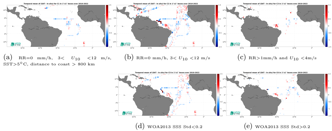
Figure 14: Temporal mean gridded over spatial boxes of size 1^\circ \times 1^\circ of \Delta SSS (SMOS SSS L3 v9 - 18 Days (CATDS-CEC-LOCEAN) - TSG (CSIC-UTM)) for 5 different subdatasets corresponding to:RR=0 mm/h, 3 < U_{10} < 12 m/s, SST >5^\circ\text{C} , distance to coast > 800 km (a), RR=0 mm/h, 3 < U_{10} < 12 m/s (b), RR >1 mm/h and U_{10} < 4 m/s (c), WOA2013 SSS Std <0.2 (d), WOA2013 SSS Std >0.2 (e).
