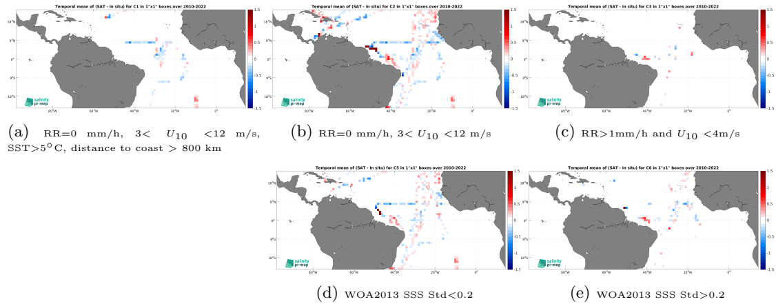
Figure 12: Temporal mean gridded over spatial boxes of size 1^\circ \times 1^\circ of \Delta\text{SSS} (SMOS SSS L3 v9 - 18 Days (CATDS-CEC-LOCEAN) - TSG (CSIC-UTM)) for 5 different subdatasets corresponding to:RR=0 mm/h, 3 < U_{10} < 12 m/s, SST >5^\circ\text{C} , distance to coast > 800 km (a), RR=0 mm/h, 3 < U_{10} < 12 m/s (b), RR >1 mm/h and U_{10} < 4 m/s (c), WOA2013 SSS Std <0.2 (d), WOA2013 SSS Std >0.2 (e).
