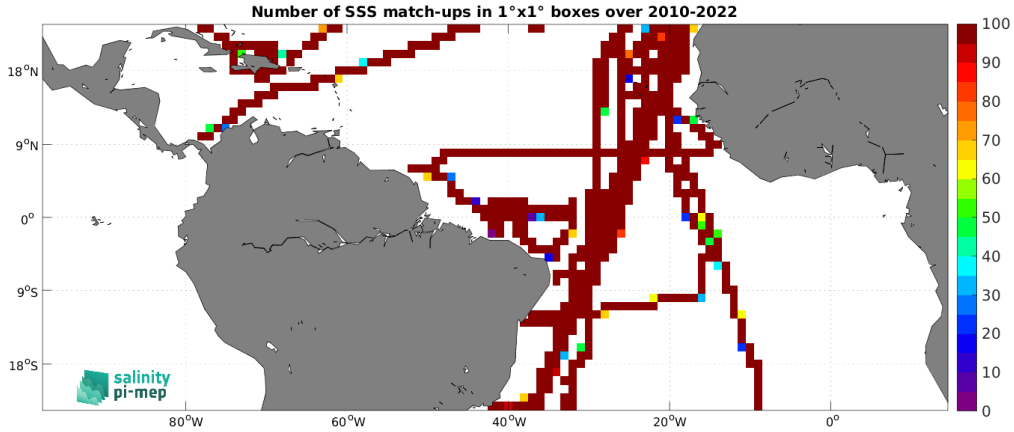
Figure 4: Number of SSS match-ups between TSG (CSIC-UTM) SSS and the SMOS SSS L3 v9 - 18 Days (CATDS-CEC-LOCEAN) SSS product for the Tropical Atlantic Ocean Pi-MEP region over 1^\circ \times 1^\circ boxes and for the full satellite product period.
