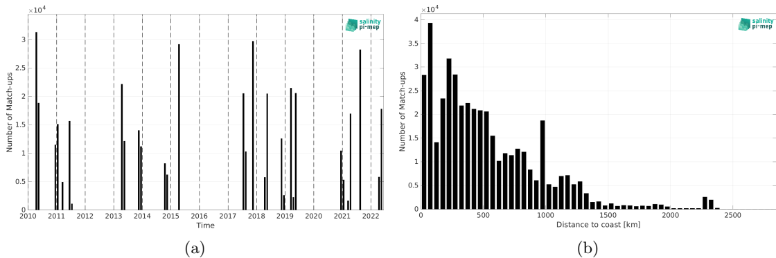
Figure 1: Number of match-ups between TSG (CSIC-UTM) and SMOS SSS L3 v9 - 18 Days (CATDS-CEC-LOCEAN) SSS as a function of time (a) and as function of the distance to coast (b) over the Tropical Atlantic Ocean Pi-MEP region and for the full satellite product period.
