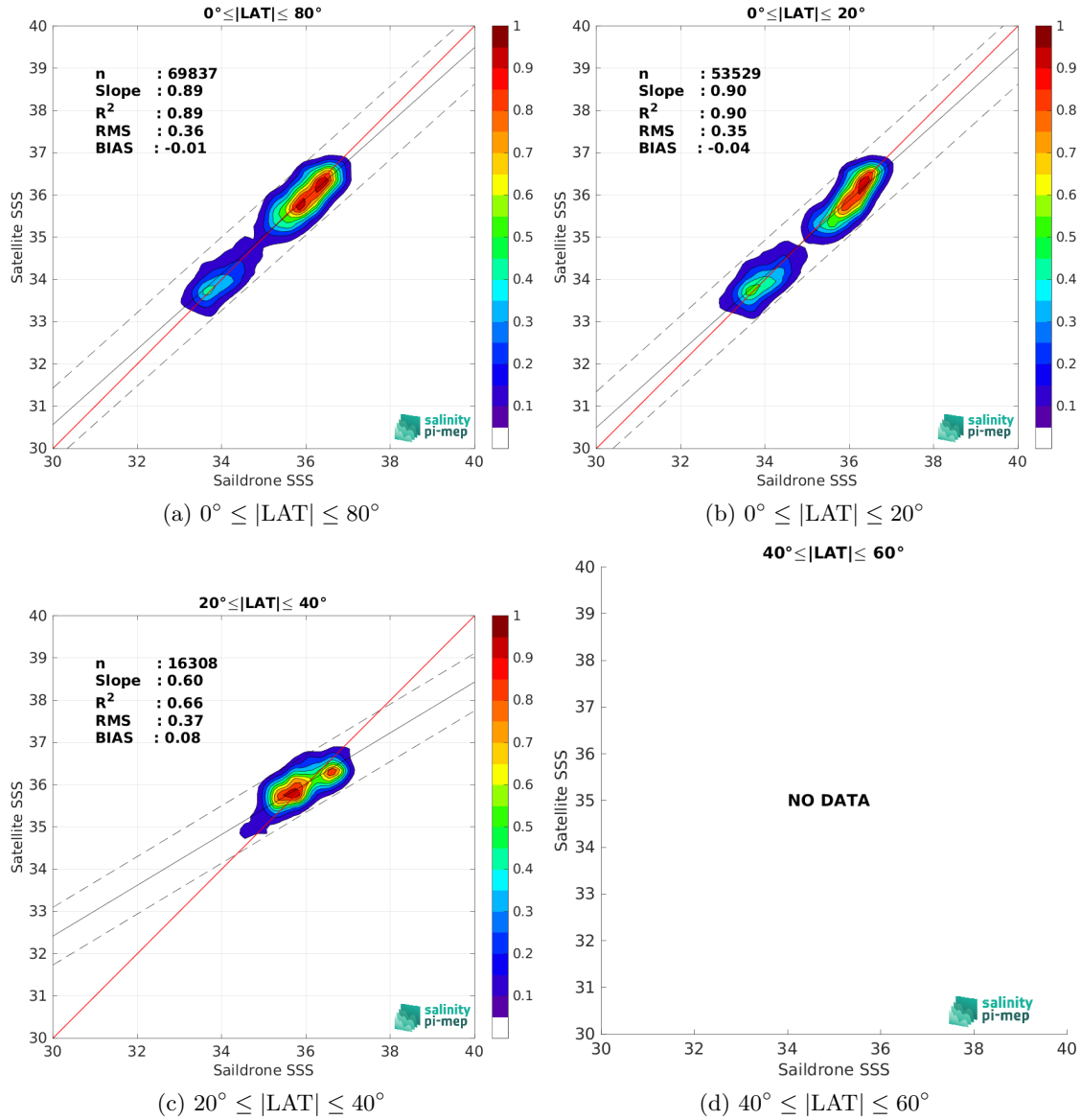
Figure 10: Contour maps of the concentration of SMOS SSS L3 v9 - 18 Days (CATDS-CEC-LOCEAN) SSS (y-axis) versus Saldrone SSS (x-axis) at match-up pairs for different latitude bands. For each plot, the red line shows x=y . The black thin and dashed lines indicate a linear fit through the data cloud and the \pm 95\% confidence levels, respectively. The number match-up pairs n , the slope and R^2 coefficient of the linear fit, the root mean square (RMS) and the mean bias between satellite and in situ data are indicated for each latitude band in each plots.
