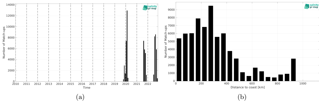
Figure 2: Number of match-ups between Saildrone and SMOS SSS L3 v9 - 18 Days (CATDS-CEC-LOCEAN) SSS as a function of time (a) and as function of the distance to coast (b) over the Tropical Atlantic Ocean Pi-MEP region and for the full satellite product period.
