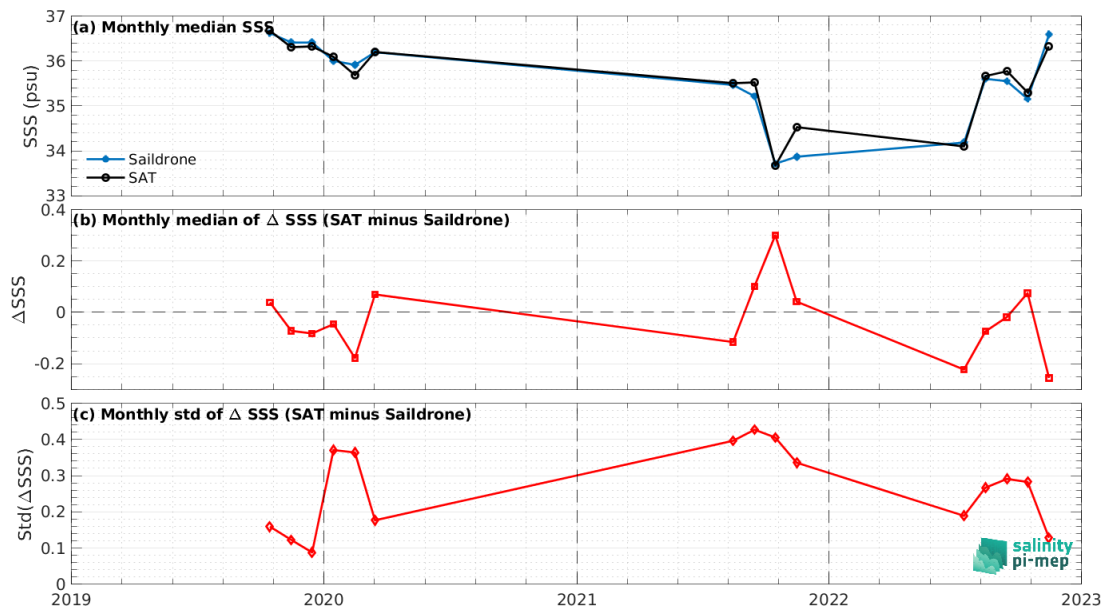
Figure 8: Time series of the monthly median SSS (top), median of \Delta SSS (Satellite - Sairdrone) and Std of \Delta SSS (Satellite - Sairdrone) over the Tropical Atlantic Ocean Pi-MEP region considering all match-ups collected by the Pi-MEP.
