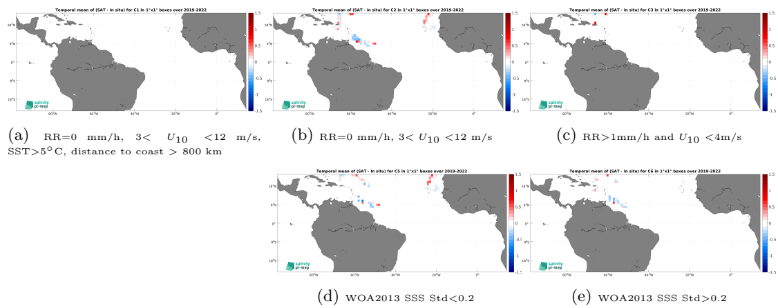
Figure 14: Temporal mean gridded over spatial boxes of size 1^\circ \times 1^\circ of \Delta\text{SSS} (SMOS SSS L3 v9 - 18 Days (CATDS-CEC-LOCEAN) - Saildrone) for 5 different subdatasets corresponding to:RR=0 mm/h, 3 < U_{10} < 12 m/s, SST>5°C, distance to coast > 800 km (a), RR=0 mm/h, 3 < U_{10} < 12 m/s (b), RR>1mm/h and U_{10} < 4 m/s (c), WOA2013 SSS Std<0.2 (d), WOA2013 SSS Std>0.2 (e).
