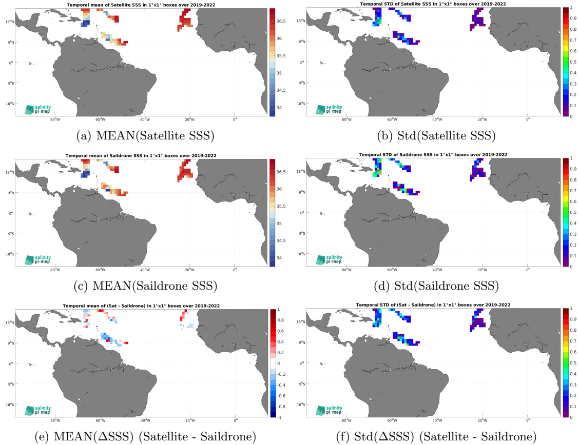
Figure 6: Temporal mean (left) and Std (right) of SSS from SMOS SSS L3 v9 - 18 Days (CATDS-CEC-LOCEAN) (top), Saildrone (middle), and of \Delta\text{SSS} (Satellite - Saildrone). Only match-up pairs are used to generate these maps.
