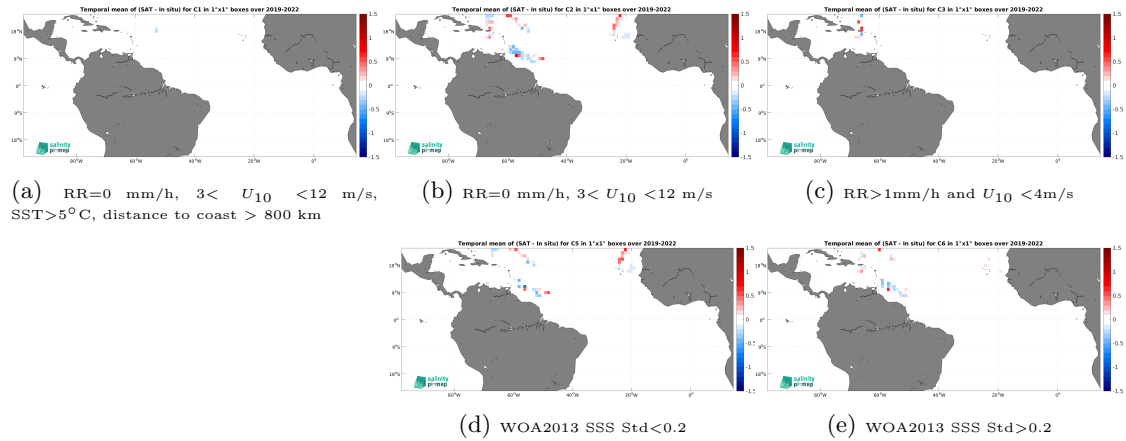
Figure 12: Temporal mean gridded over spatial boxes of size 1^\circ \times 1^\circ of \Delta SSS (SMOS SSS L3 v9 - 18 Days (CATDS-CEC-LOCEAN) - Sailydrone) for 5 different subdatasets corresponding to:RR=0 mm/h, 3 < U_{10} < 12 m/s, SST >5^\circ\text{C} , distance to coast > 800 km (a), RR=0 mm/h, 3 < U_{10} < 12 m/s (b), RR >1 mm/h and U_{10} < 4 m/s (c), WOA2013 SSS Std <0.2 (d), WOA2013 SSS Std >0.2 (e).
