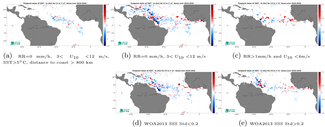
Figure 11: Temporal mean gridded over spatial boxes of size 1^\circ \times 1^\circ of \Delta SSS (SMOS SSS L3 v9 - 18 Days (CATDS-CEC-LOCEAN) - Surface drifters) for 5 different subdatasets corresponding to:RR=0 mm/h, 3 < U_{10} < 12 m/s, SST >5^\circ C, distance to coast > 800 km (a), RR=0 mm/h, 3 < U_{10} < 12 m/s (b), RR >1 mm/h and U_{10} < 4 m/s (c), WOA2013 SSS Std <0.2 (d), WOA2013 SSS Std >0.2 (e).
