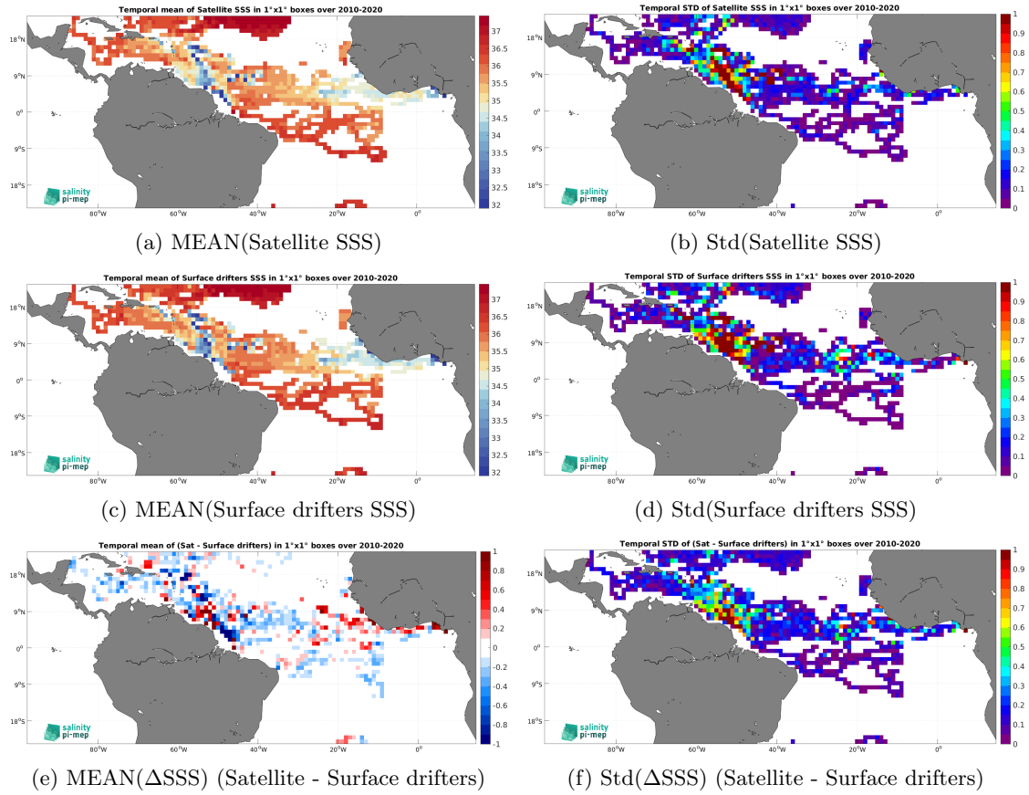
Figure 5: Temporal mean (left) and Std (right) of SSS from SMOS SSS L3 v9 - 18 Days (CATDS-CEC-LOCEAN) (top), Surface drifters (middle), and of \Delta SSS (Satellite - Surface drifters). Only match-up pairs are used to generate these maps.
