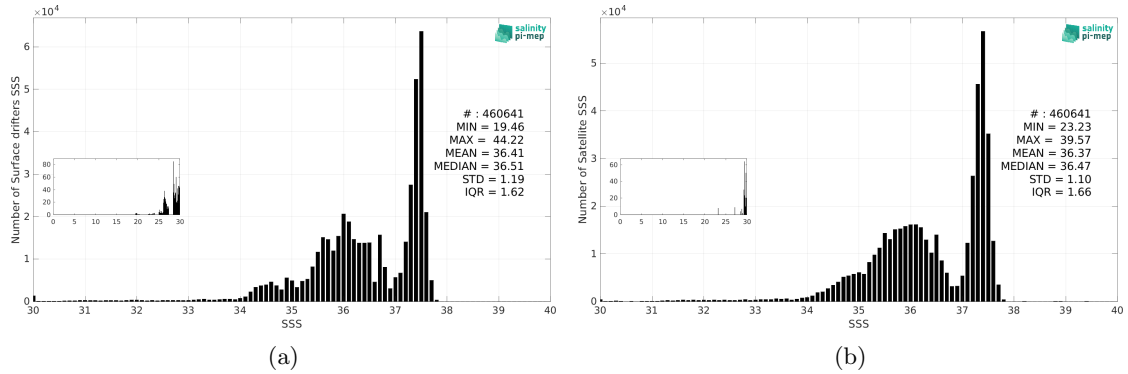
Figure 2: Histograms of SSS from Surface drifters (a) and SMOS SSS L3 v9 - 18 Days (CATDS-CEC-LOCEAN) (b) considering all match-up pairs per bins of 0.1 over the Tropical Atlantic Ocean Pi-MEP region and for the full satellite product period.
