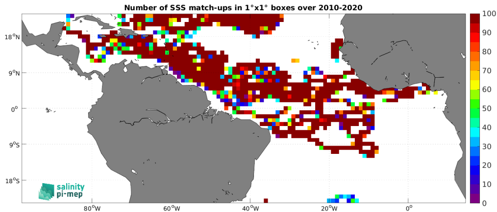
Figure 3: Number of SSS match-ups between Surface drifters SSS and the SMOS SSS L3 v9 - 18 Days (CATDS-CEC-LOCEAN) SSS product for the Tropical Atlantic Ocean Pi-MEP region over 1^\circ \times 1^\circ boxes and for the full satellite product period.
